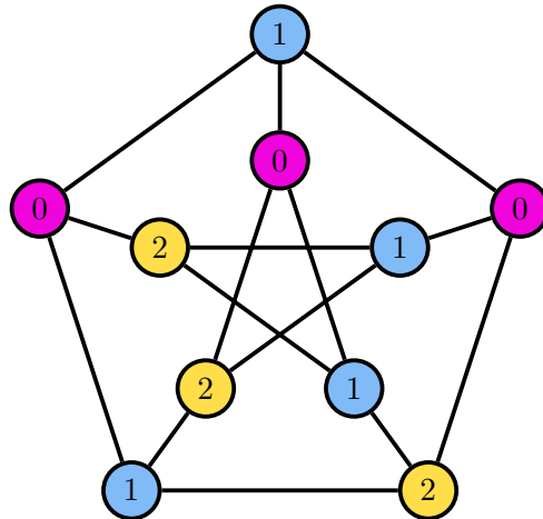
Figure 14: A 3-coloring of Petersen's graph
