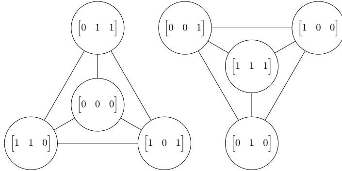
Figure 1.9: The graph \mathbb{Z}_2^\Delta
