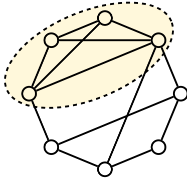
Figure 15: A graph that contains a clique of size 4
