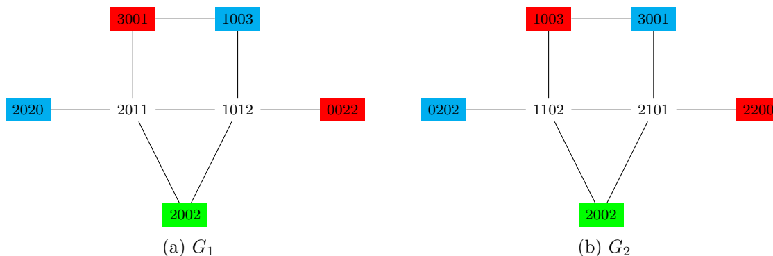
Figure 1.8: The colorings of G_1 and G_2 cannot be extended as 4-colorings
