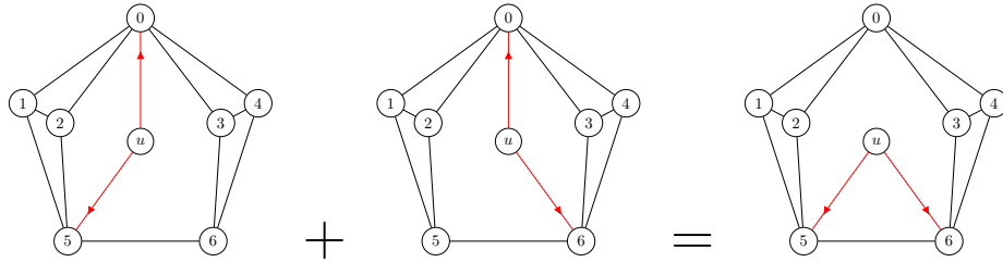
Figure 1.18: Sum of two diamond widgets
