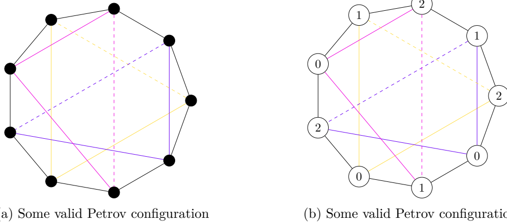
Figure 2.10: A Petrov configuration gives two non zero terms of the inner product
