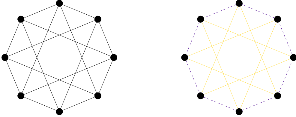
Figure 2.1: The complete bipartite graph K_{4,4} and a cycle factor in dotted purple
