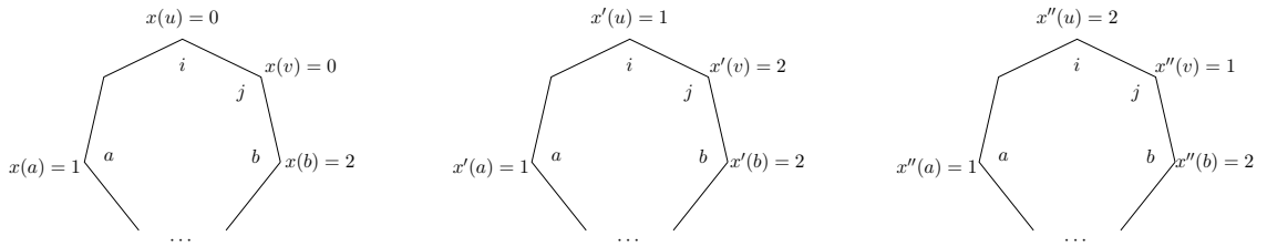
Figure 2.6: Representation of the edge-clique \{x, x', x''\}
