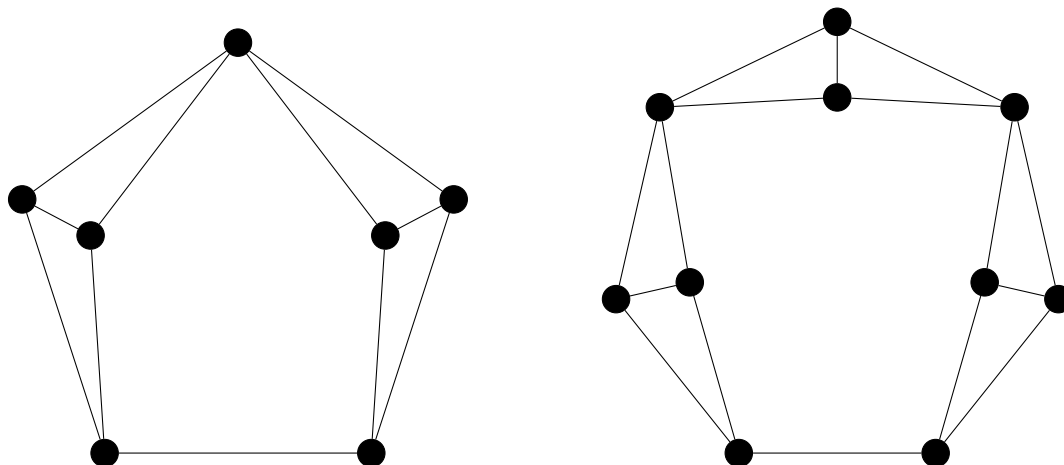
Figure 1.13: Moser Spindle
