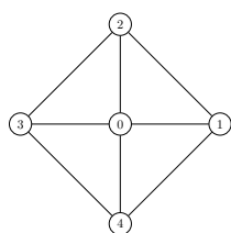
(a) The graph W_4
