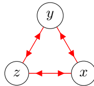
Figure 1.22: Widget given by a dominated triple
