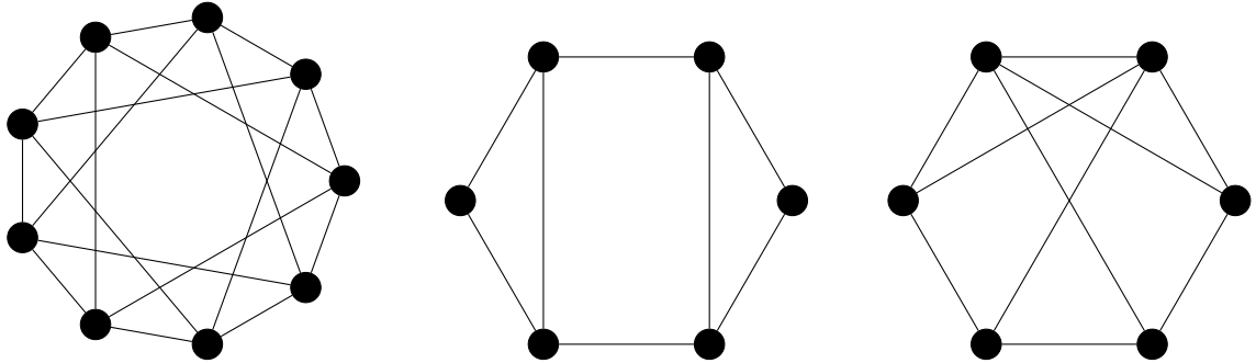
Figure 2.3: Examples of graphs of the form “cycle + triangles”
