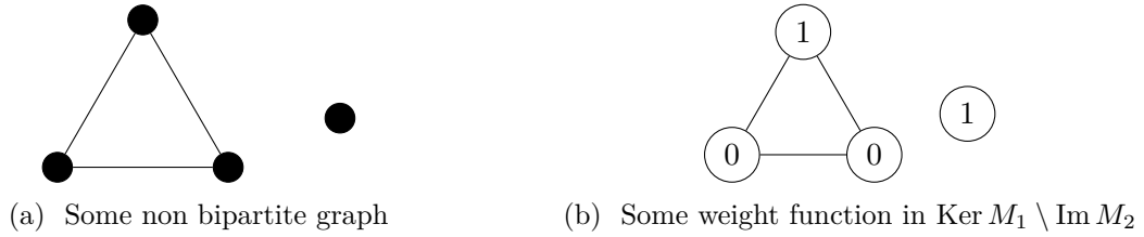
Figure 1.21: Non connected graphs can be non bipartite not for homological reasons
