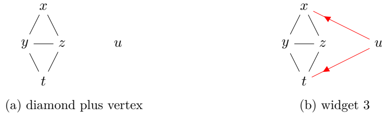
Figure 1.16: Widget 3
