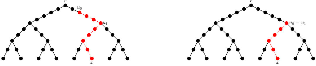
Figure 3.7: some non-3-sparse paths
