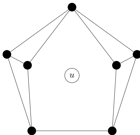
Figure 1.17: Moser Spindle
