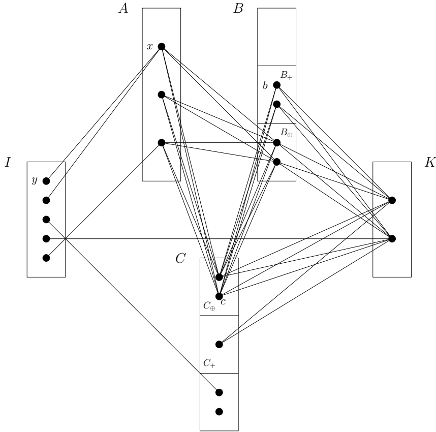
Figure 3.4: Structure of a nested t -module
