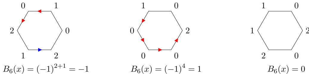
Figure 2.5: Examples of value for Bousquet precoloring
