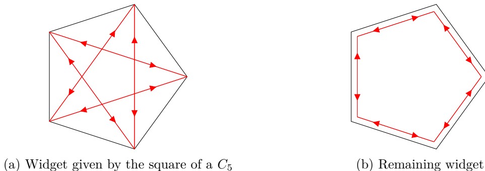
Figure 1.23: Widget for a graph G with a C_5 so that G satisfies H_3
