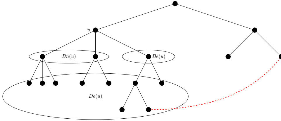
Figure 3.9: Structure of T' with an edited edge in dotted red
