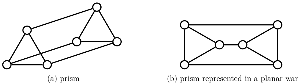
Figure 11: Two representations of the prism
