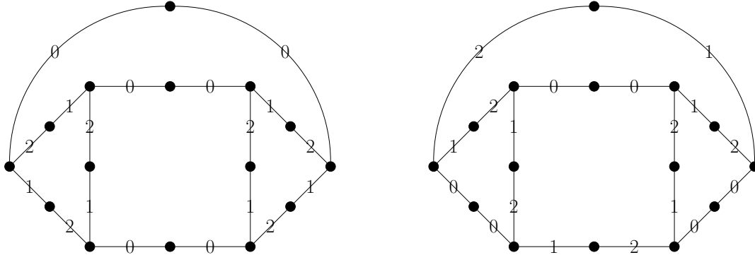
Figure 2.13: Some valid Fourier labelling for the subdivided prism
