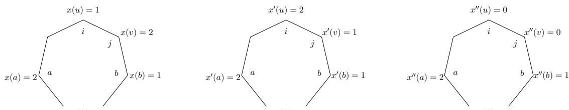
Figure 2.8: Representation of the edge-clique \{x, x', x''\}
