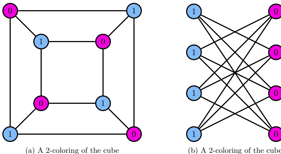
Figure 13: Coloring of the cube with two colors
