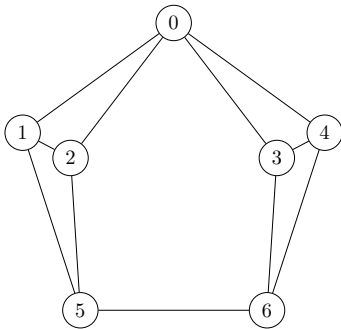
Figure 1.4: Moser Spindle graph and its matrix M_3
