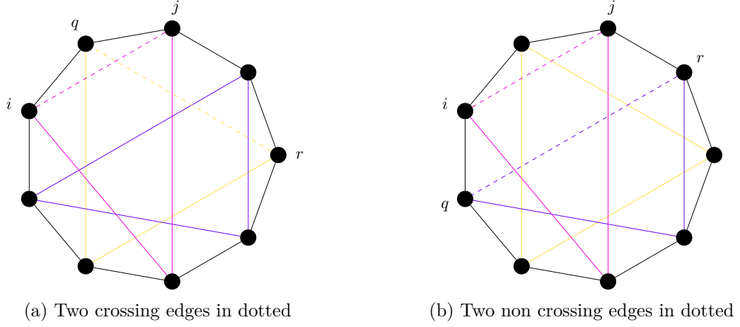
Figure 2.9: Crossing and non crossing edges
