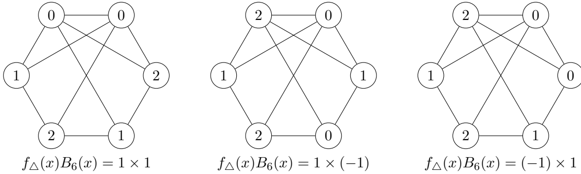
Figure 2.12: The inner product \langle f_{\Delta}, B_n \rangle may have positive and negative terms
