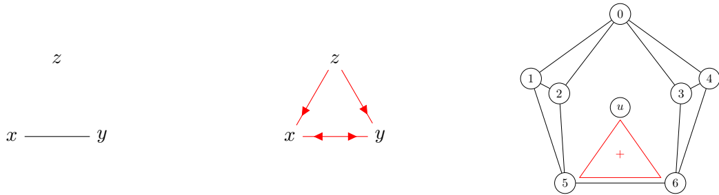
Figure 1.18: Sum of two diamond widgets
