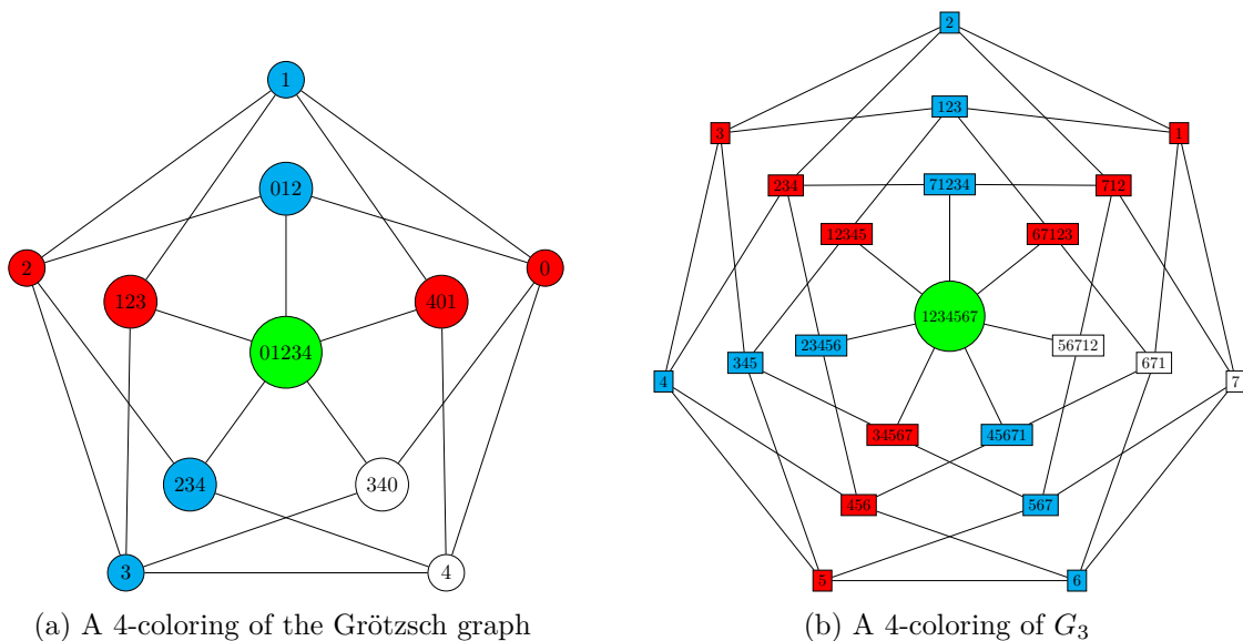
Figure 1.10: Proper 4-colorings of G_2 and G_3
