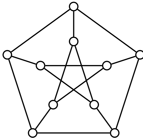
Figure 12: Petersen's graph
