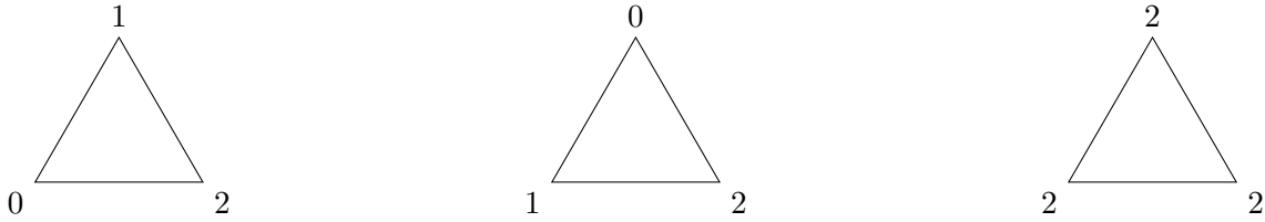
Figure C.1: The configuration of \widehat{f}_0 on some edge-clique
