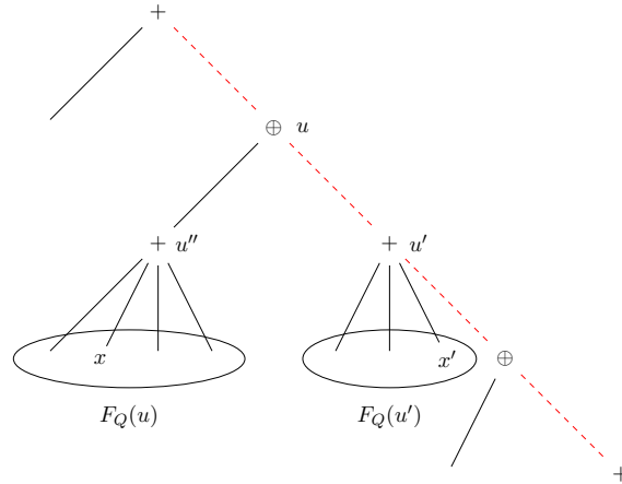
Figure 3.10: Consecutive free nodes in the path Q drawn in dotted red
