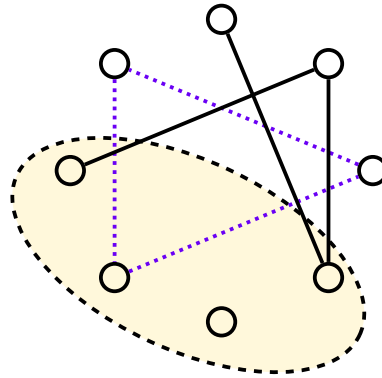
Figure 10: A clique of maximum size with edges in dotted purple and a maximum size stable set inside the dotted ellipse
