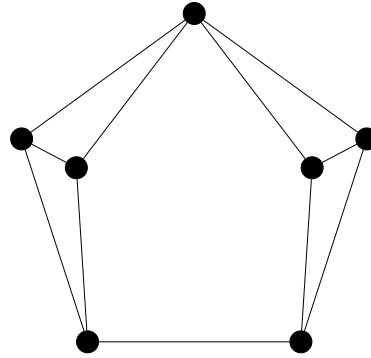
(b) The Moser Spindle graph
