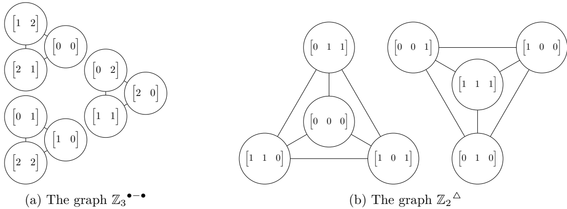
Figure 1.5: Examples of power graphs
