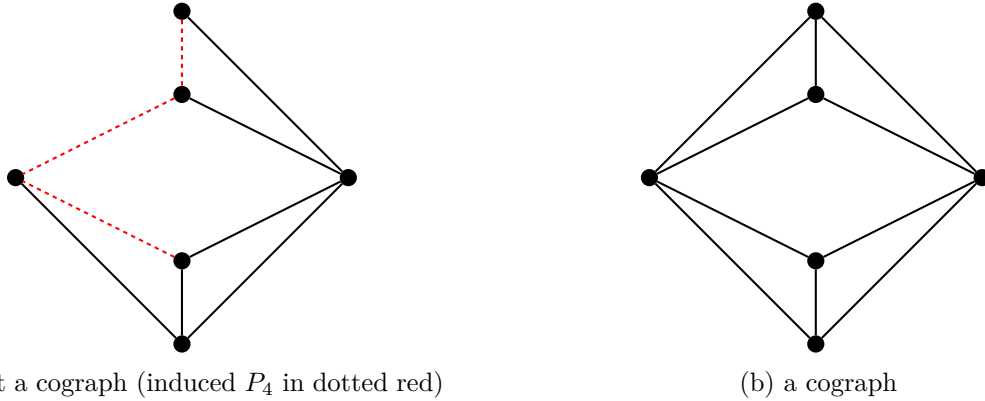
Figure 3.1: Example of a cograph and a counter example
