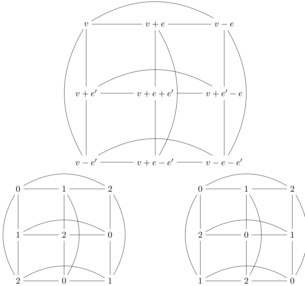
Figure 1.11: Two kind of 3-colorings for a subgraph of 3^G
