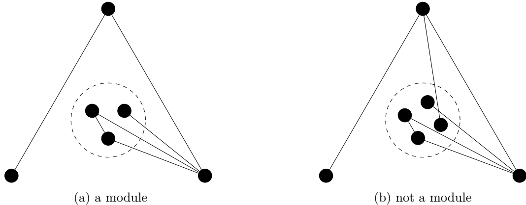
Figure 3.3: Example and counter example of modules
