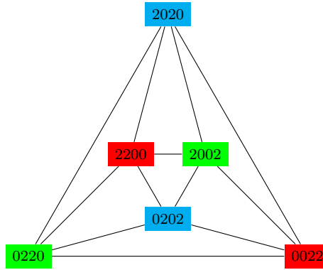
Figure 1.6: 3-coloring of a subgraph H of \mathbb{Z}_4^{K_4}
