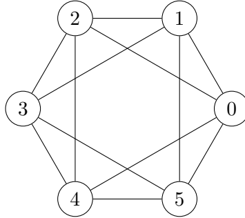
Figure 2.11: Some 3-colorable graph
