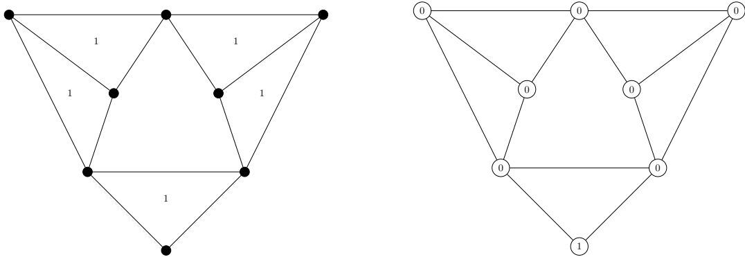
Figure 1.1: A 3-clique certificate in \mathbb{F}_2
