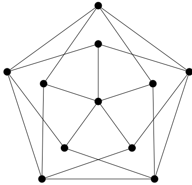
(a) The Grötzsch's graph
