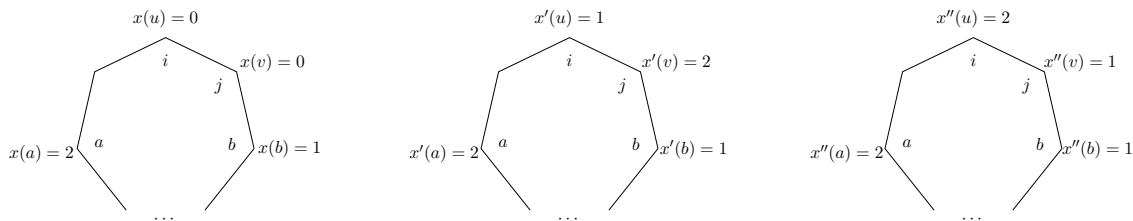
Figure 2.7: Representation of the edge-clique \{x, x', x''\}
