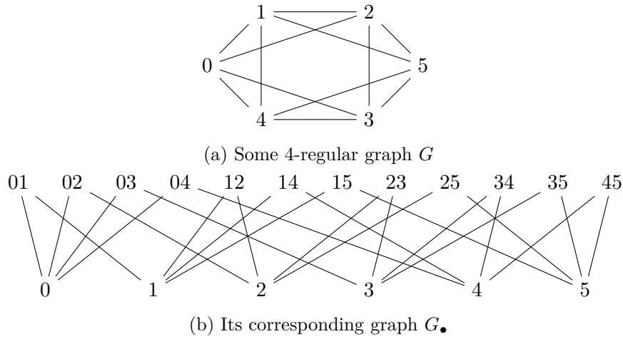
Figure 2.2: Subdivision of a graph
