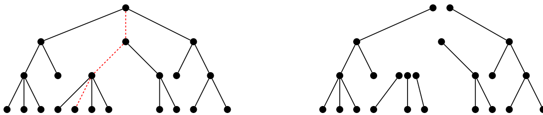
Figure 3.8: exploding a tree with path R (in dotted red)
