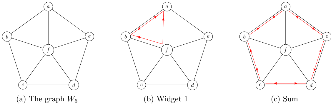
Figure 1.19: Building an edge-clique certificate for a wheel
