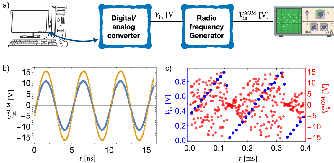
Figure 2.6: a) Diagram for controlling the radio frequency generator (RFG) through an input voltage V_{\text{in}} . Its output V_{\text{in}}^{\text{AOM}} is measured by an oscilloscope. b) Time response of the RFG for V_{\text{in}} constant in time with an intensity of 1.0 V in orange and 0.5 V in blue. The oscillation period is 5 ns. c) Linear variation of V_{\text{in}} in time and associated response V_{\text{in}}^{\text{AOM}} of the RFG. Since the periods of the two signals have a few orders of magnitude of difference and the trigger on the oscilloscope was set on the linear variation of V_{\text{in}} , it is not possible to resolve the fast oscillations shown in b) for V_{\text{in}}^{\text{AOM}} . As a consequence, this signal corresponds to a series of uncorrelated points with amplitudes that change in time.
