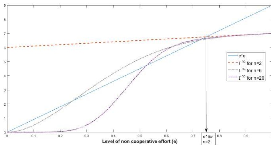
Figure 1.3: Non Cooperative equilibria of the n-player game.
