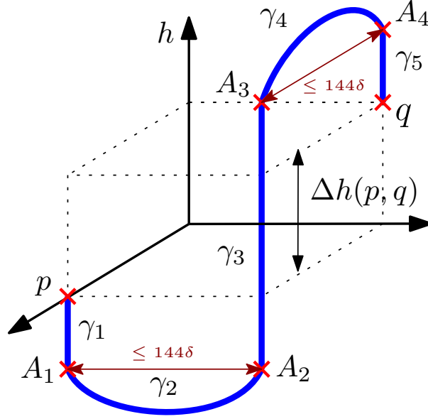
Figure 4.2: Construction of the path \gamma when h(p) \leq h(q) for Lemma 4.3.1 .
