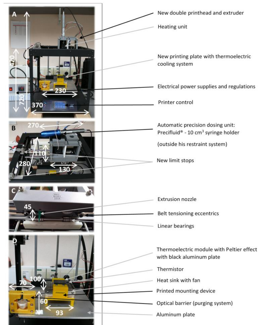
Figure 3. (A) General view of the lab-scale modified Ghost printer. (B) Top view of the printhead with the volumetric dosing system removed. (C) Bottom view of the printhead. (D) View of the new printing plate (usable area 16 cm 2 ). Dimensions are in mm. The drawings of the specifically-designed parts for modifying the 3D printer are available in Supplementary Materials S2.
