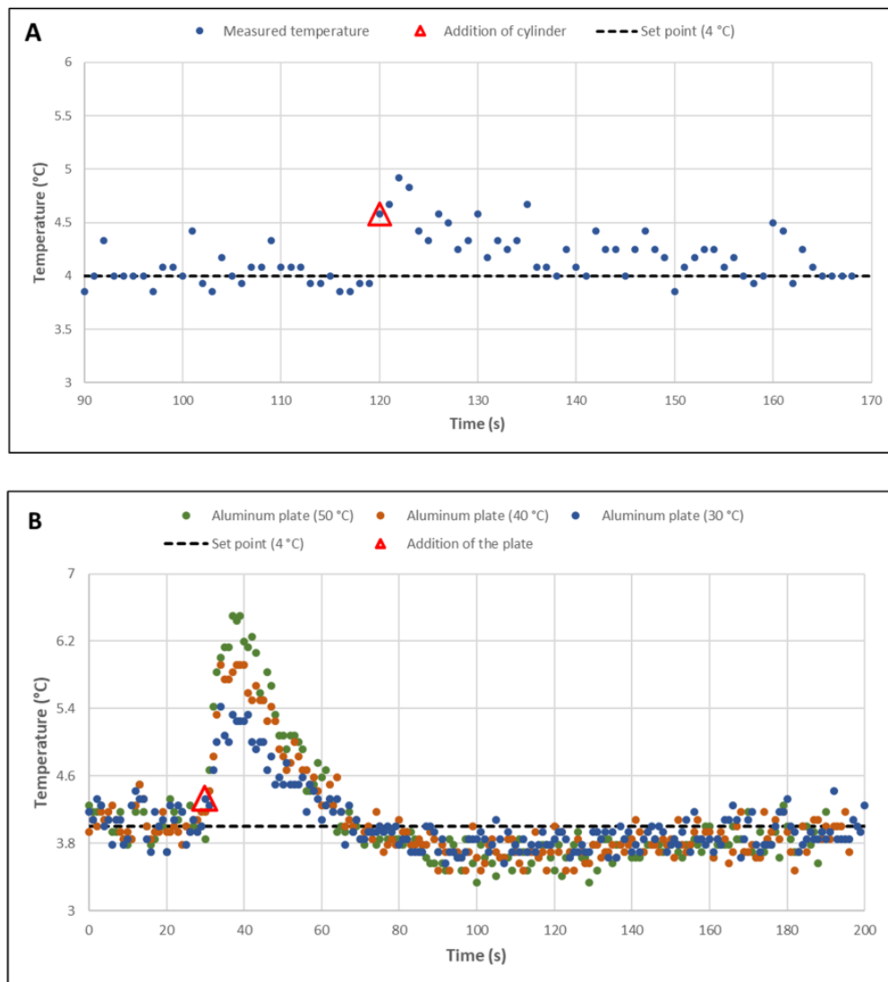
Figure 5. (A) Visualization of the temperature deviation from the setpoint after a hot gelatin cylinder (30 °C) 20 mm in diameter and 10 mm high was placed on the 16 cm 2 printing plate. (B) After placing an aluminum plate 2 mm thick and 16 cm 2 in cross section heated to 30 °C, 40 °C, and 50 °C on the printing plate.
