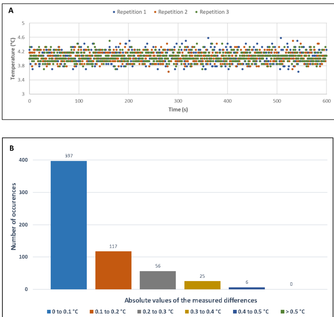
Figure 4. Graphical representation illustrating the temperature control of the printing plate. (A) Stability over 600 s for a setpoint temperature of 4 °C and one measurement per second. (B) Data distribution according to the absolute value of their deviation from the setpoint.
