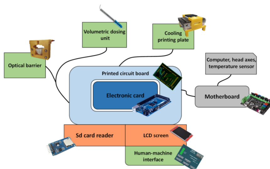
Figure 2. Schematic representation of the various electronically controlled components of the 3D food printer built. “Supplementary Materials S1” gives accurate information about the connectivity between the different added elements.
