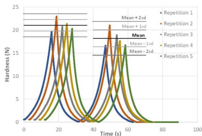
Figure 9. Hardness measurements of printed protein gels using the TPA test. The horizontal line represents the mean (in black) of the maximum protein forces for the five samples, and for the two successive compressions. The standard deviations around this mean are represented by the shaded horizontal lines.
