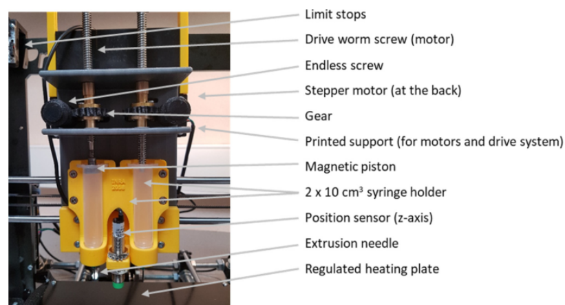
Figure 1. Printhead developed based on a Prusa i3 3D printer. The different modified elements were designed with Inventor ® and then 3D-printed.
