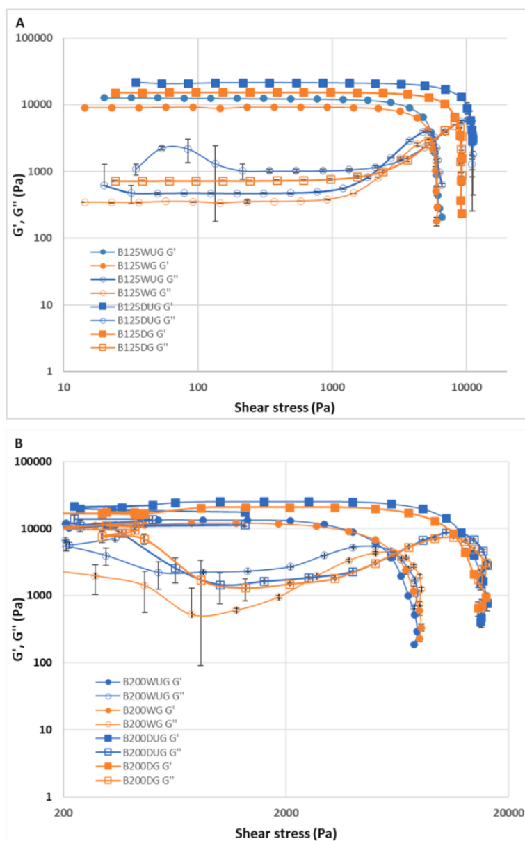
Fig. 4. Average curves of storage modulus ( G' ) and loss modulus ( G'' ). A - Mean G' and G'' curves for conditions B125W and B125D. B - Mean G' and G'' curves for conditions B200W and B200D. Calculated from 3 repetitions. Error bars correspond to the SEM.
