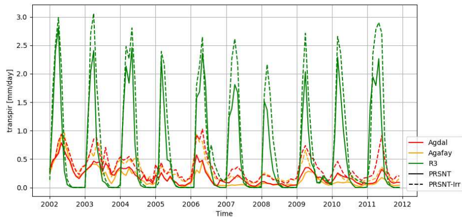
Figure 4.18: Monthly averaged transpiration ( \text{mm day}^{-1} ) over Agdal (red color), Agafay (orange) and R3 (green) during the 10-year simulation 2002-2011. Solid lines correspond to the PRSNT configuration, dashed lines correspond to the PRSNT-Irr.
