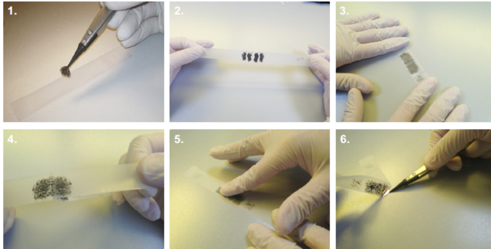
Figure A.3: Illustration of the steps of the mechanical exfoliation of 2D-materials. Adapted from [16].
