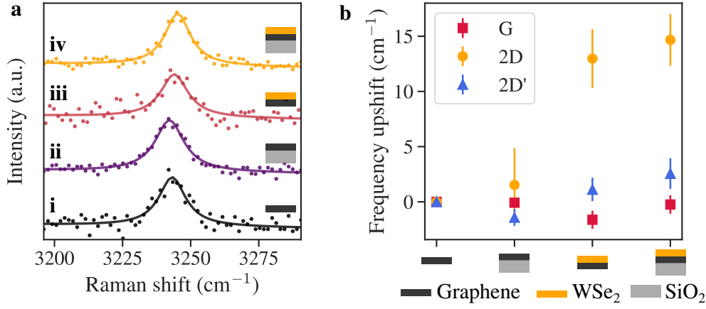
Figure 3.6: Upshift of the 2D'-mode frequency in various dielectric environments.
