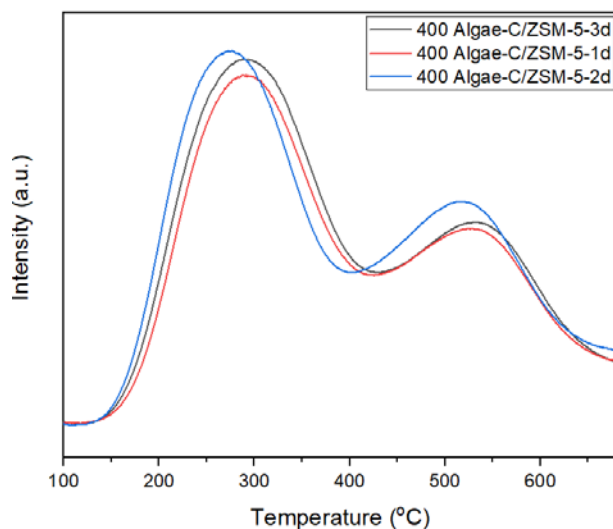
Figure 4.20 NH 3 -TPD profiles of 400 Algae-C/ZSM-5 with different hydrothermal times (3d, 2d, 1d).
