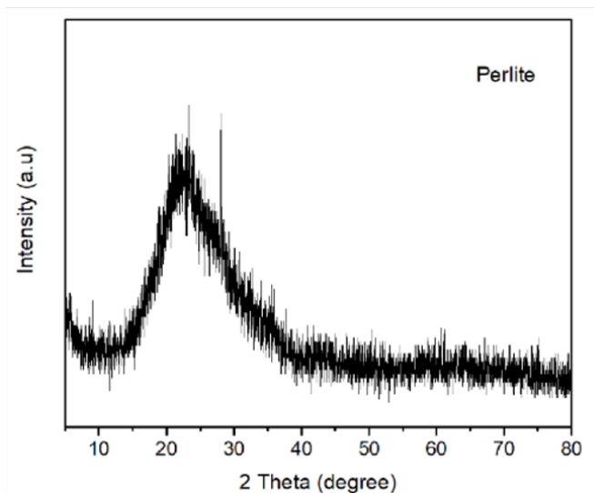
Figure 5.4 XRD pattern of perlite.
