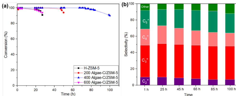
Figure 4.16 (a) Methanol conversion and (b) product selectivity of Algae-C/ZSM-5-3d with different Algae-C addition in the MTO at 350 °C, WHSV=2 h -1 .
