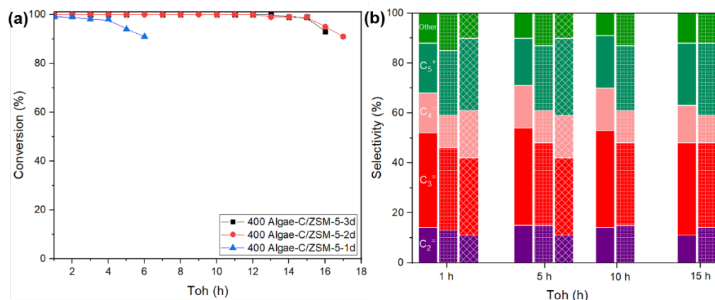
Figure 4.21 Methanol conversion of different catalysts (a), products selectivity of 400 Algae-C/ZSM-5 (■ 3d, ● 2d, ▲ 1d) in the MTO at 400 °C, WHSV=8 h -1 .
