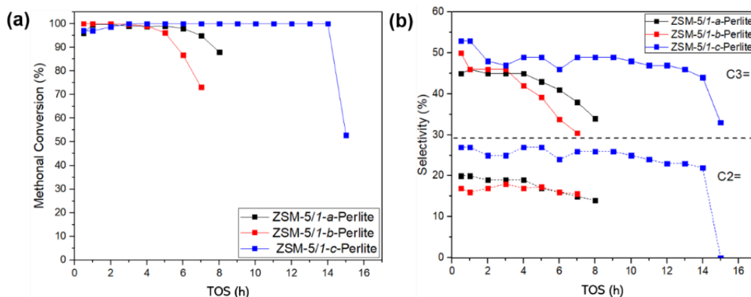
Figure 5.10 (a) Methanol conversion, (b) Ethylene and propylene selectivities in the MTO process at 475 °C over ZSM-5/1- n -Perlite ( n = a , b , c ) samples.
