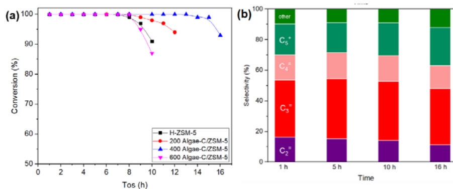
Figure 4.17 (a) Methanol conversion and (b) product selectivity of Algae-C/ZSM-5-3d with different Algae-C addition in the MTO at 400 °C, WHSV=8 h -1 .
