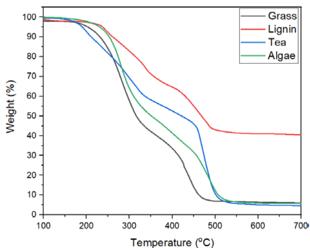
Figure 3.2 TG curves of Grass, Lignin, Algae and Tea biomasses.
