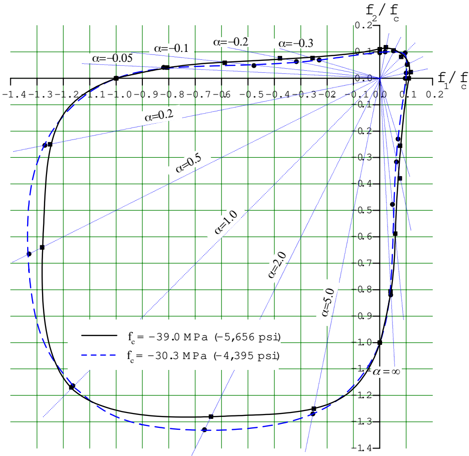
Figure 1.4 • Biaxial strength envelopes for two different types of concrete under biaxial stress (Lee et al., 2004). f_c is the compressive strength of the specimen.
