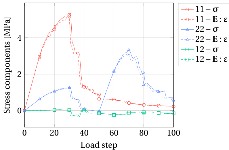
Figure 4.8 • Comparison the symmetrized stress from the discrete model \sigma (reference) to the stress from the measured effective elasticity tensor \mathbf{E} : \epsilon .
