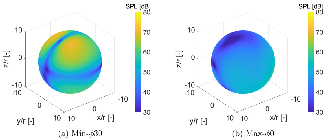
Figure 5.19: 3D directivity patterns of the 1st BPF (700 Hz) for total loading noise sources in loudest (a) and quietest configurations (b) with COR propellers.
