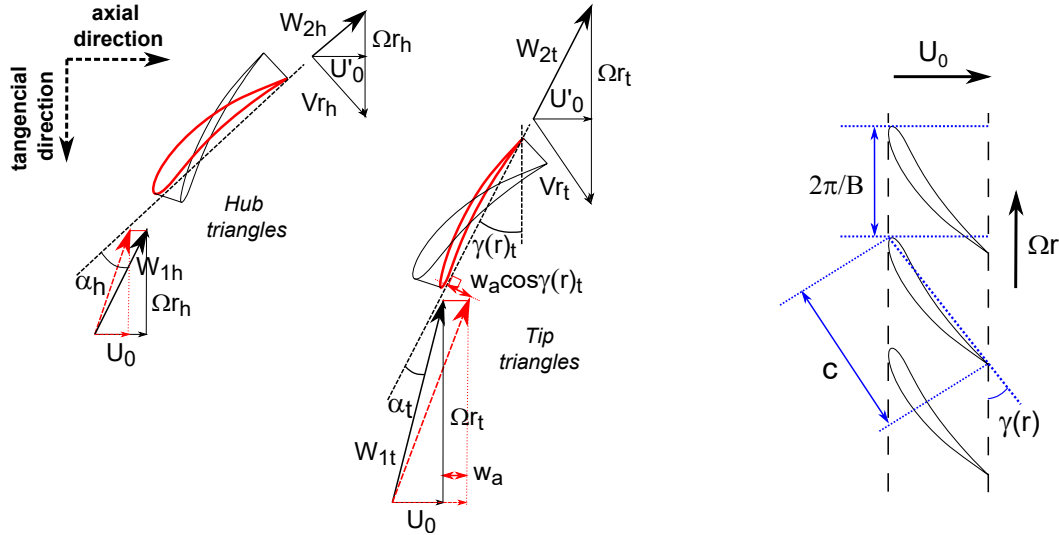
(a) Velocity triangles at the blade hub and tip (b) Unwrapped representation of a strip
