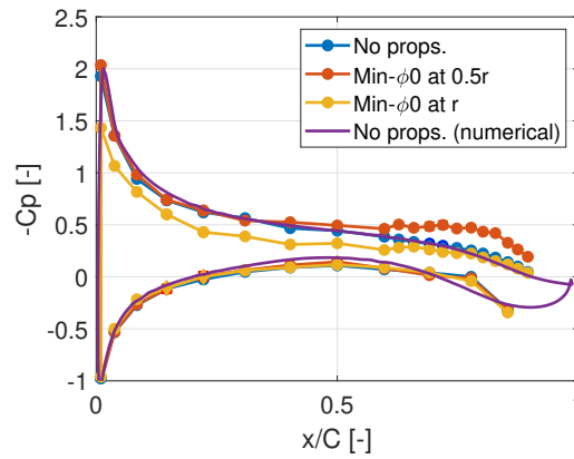
Figure 3.26: Experimental and numerical C_P comparison with COR propellers.
