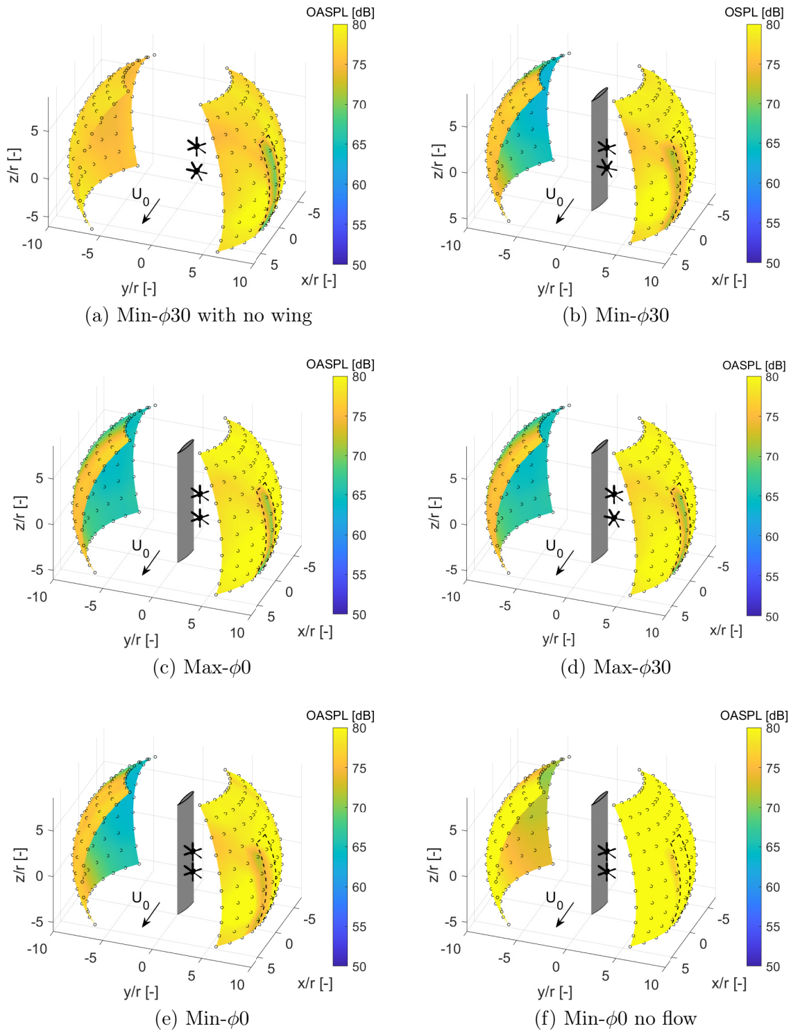
Figure 3.43: 3D directivity patterns of broadband-noise OASPL (4 – 24 kHz) of configurations with COR propellers.
