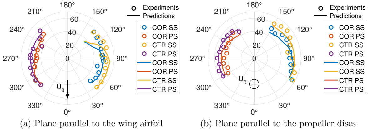
Figure 5.24: Experimental and analytical 2D directivity patterns of the 1st BPF ( 700 \text{ Hz} ) in Max- \phi_0 configurations, for CTR and COR arrangements. SS: suction side and PS: pressure side.
