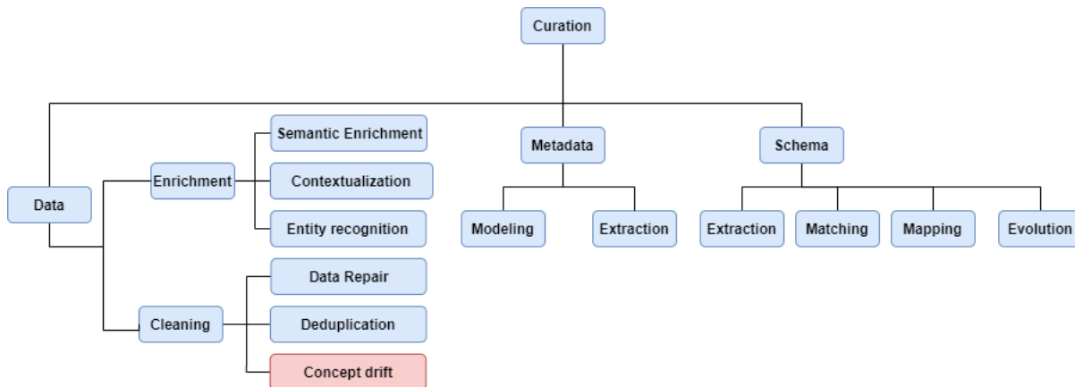
Figure 2.7: Taxonomy of data curation tasks
