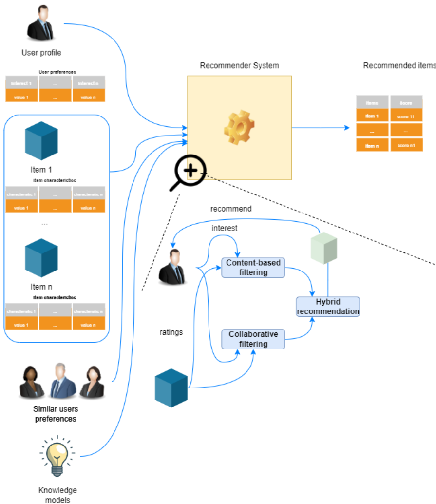
Figure 2.9: Hybrid filtering
