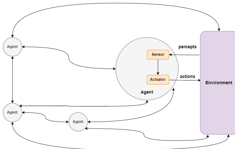
Figure 2.5: Multi-agent system
