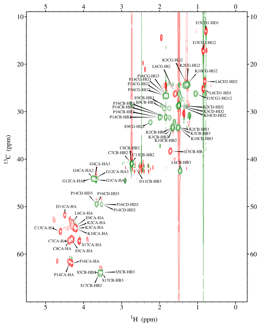
Figure 4.57 - Assignments of 2D ^1\text{H} - ^{13}\text{C} HSQC MEG 2.1 isoform 1b (17 aa, G42 - S58) peptide in DMSO- d_6 at a concentration of 2 mM. Experiments have been recorded at 27 °C with Varian Inova spectrometer operated at a ^1\text{H} frequency of 600 MHz (14.1 T) and equipped with a triple HCN cryoprobe enhanced in ^1\text{H} and ^{13}\text{C} . Assignments of amino acids are numbered within the analyzed peptide (1-17).
