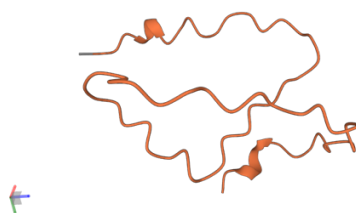
Figure 4.23 - MEG 6 protein structure prediction via ESMFold.
