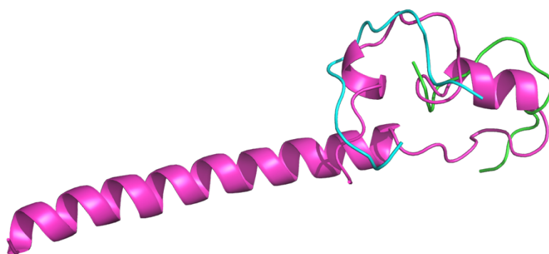
Figure 5.1 - Overlay of the structure obtained after 4 \mu s run of molecular dynamics with two peptides (iso 1f - green and 1g - cyan) determined by NMR.
