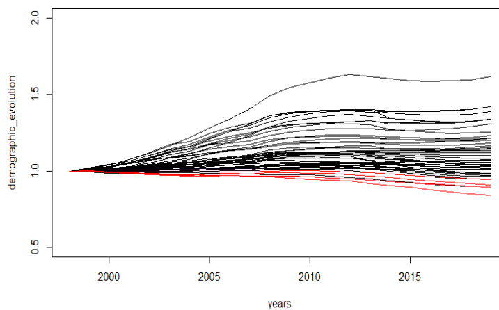
Figure 5.5: The demographic evolution curves (from 1998 to 2019) in each provinces are presented. Curves in red correspond to provinces inside \hat{C}_H , curves in black correspond to provinces outside \hat{C}_H .
