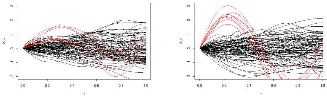
Figure 3.9: An example of the simulated data for the sBm process with \Delta_3(t) = \sin(2\pi t) (left panel) and \Delta_3(t) = 2.5 \sin(2\pi t) (right panel). Curves in red correspond to the observations in the cluster.
