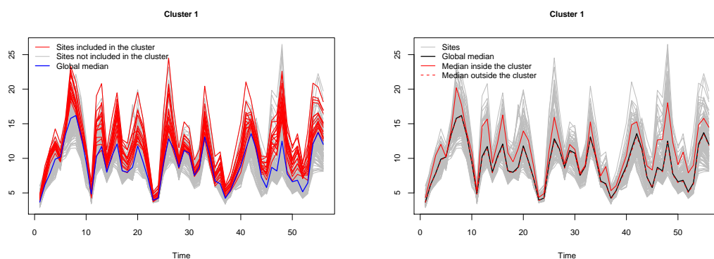
Figure 4.7: Characterization of the most likely cluster for the URBESS scan approach in the context of univariate functional data with the functions plot_curves_clusters() (left panel) and plot_summary_curves() (right panel)
