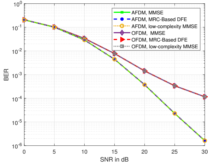
(a) Integer Doppler shifts
