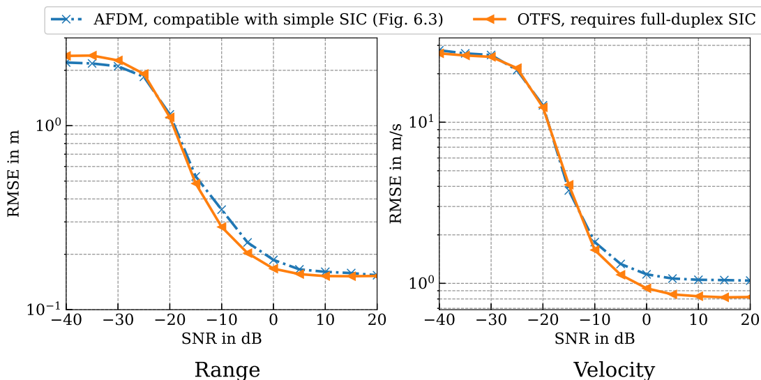
Figure 6.5: Sensing performance of AFDM-based and OTFS-based ISAC
