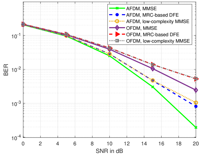
(b) Fractional Doppler shifts
