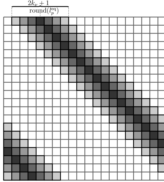
Figure 3.6: Structure of \mathbf{H}_p for fractional Doppler shifts
