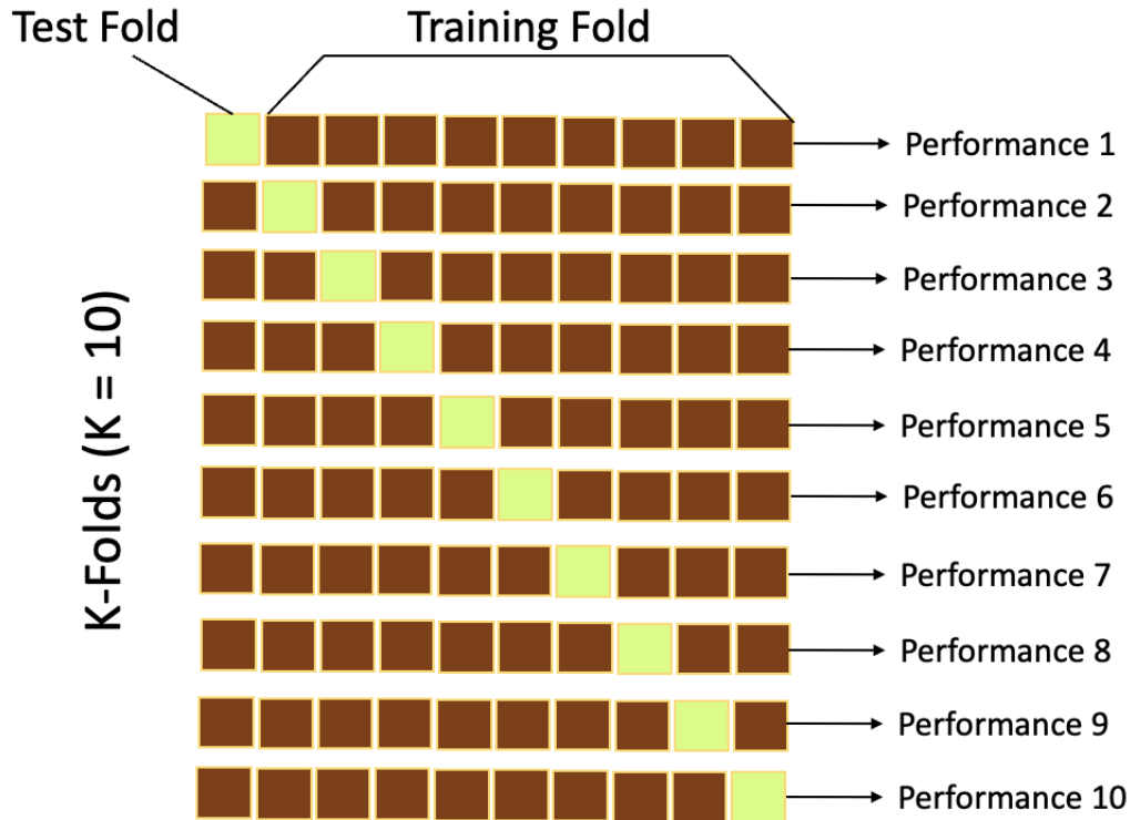
Figure 4.3: Cross Validation
