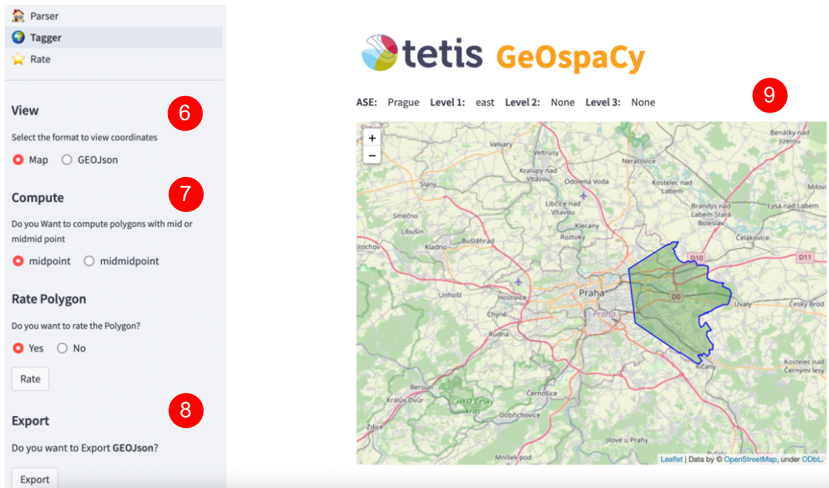
Figure 3.10: Geocoding Method
