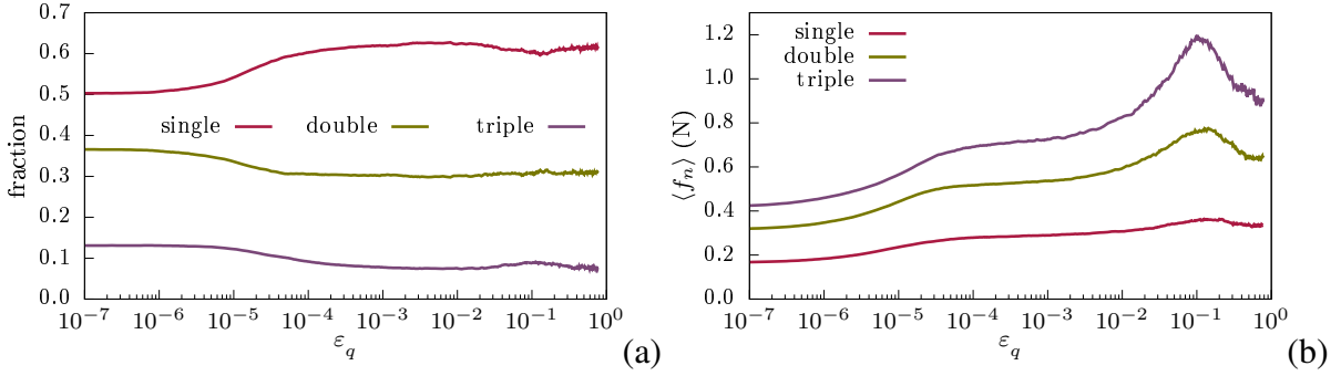
Fig. 2-17. The fraction (a) and the average normal force \langle f_n \rangle (b) of single, double and triple contacts as a function of shear strain \epsilon_q in the packing of icosahedral particles with friction coefficient \mu_s = 0.1 .
