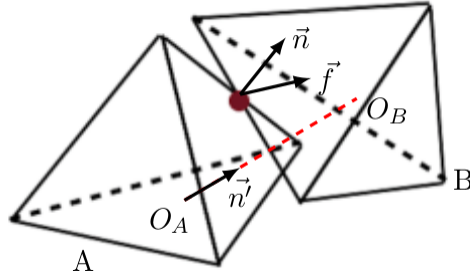
Fig. B-2. Geometry of a contact between two polyhedra. \vec{n} is unit normal vector of contact point, \vec{n}' is unit normal vector of branch length.
