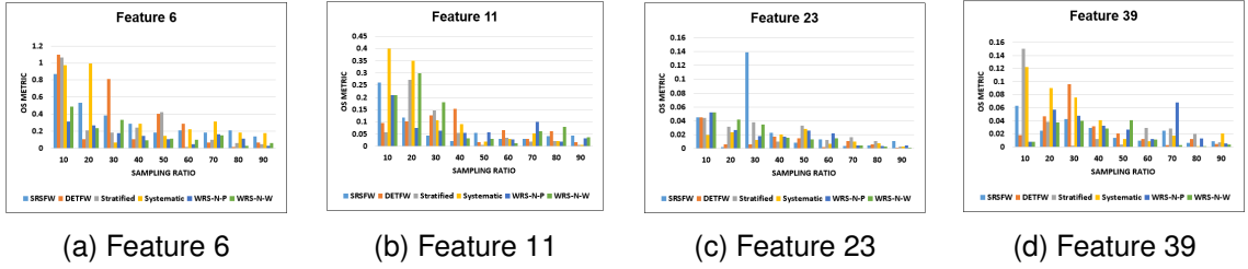
Figure 2.7: Comparison of OS metric for non-stream sampling policies at different sampling ratios for features 6, 11, 23, and 39.
