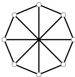
Figure 3.3: Wagner graph
