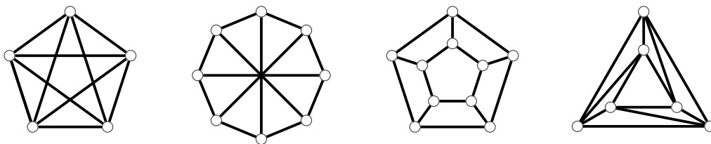
Figure 3.4: Forbidden minors for graphs of treewidth at most 3
