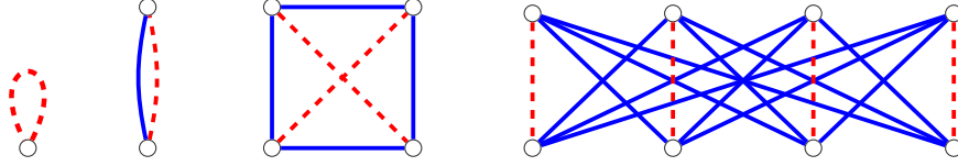
Figure 3.1: \mathcal{SPC}_d for d \in \{0, 1, 2, 3\}
