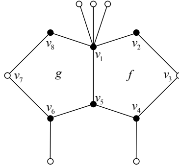
Figure 6.3: The configuration of Lemma 6.11.
