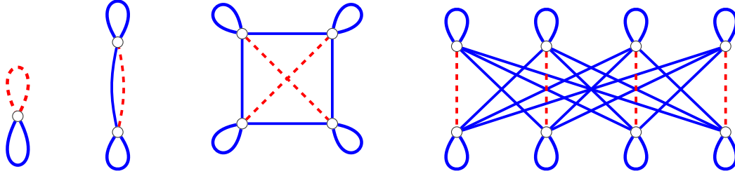
Figure 3.2: \mathcal{SPC}_d^o for d \in \{0, 1, 2, 3\}
