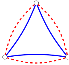
Figure 2.2: \rho(K_3^2) = 1
