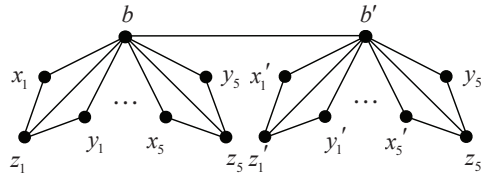
Figure 7.2: The auxiliary graph \mathcal{B} .
