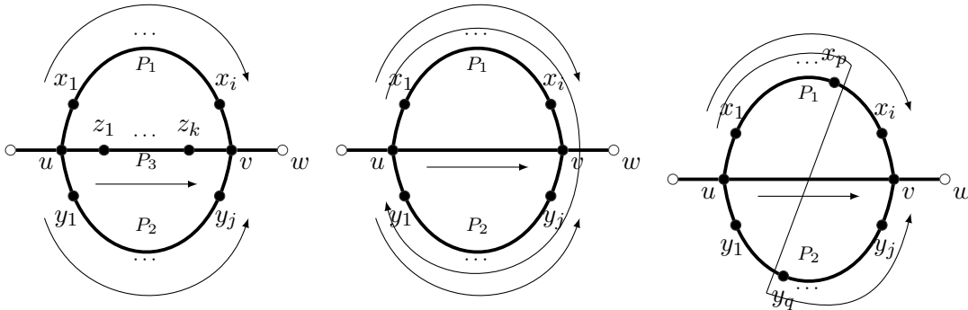
Figure 5.1: 3 disjoint light paths between u and v
