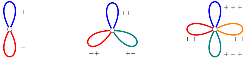
Figure 5.2: (L_1, \sigma) Figure 5.3: (L_2, \sigma_1, \sigma_2) Figure 5.4: (L_3, \sigma_1, \sigma_2, \sigma_3)
