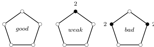
Figure 6.1: good, weak and bad 5-faces
