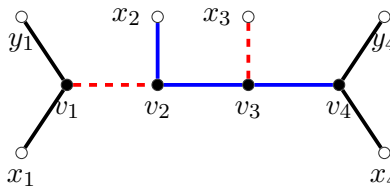
Figure 4.1: Four vertices of degree 3 in Claim 4.12
