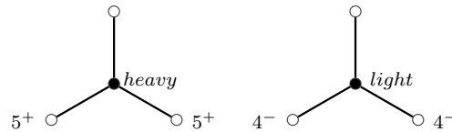
Figure 6.2: heavy and light 3-vertices
