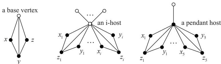
Figure 7.1: A base vertex, an i -host and a pendant host.
