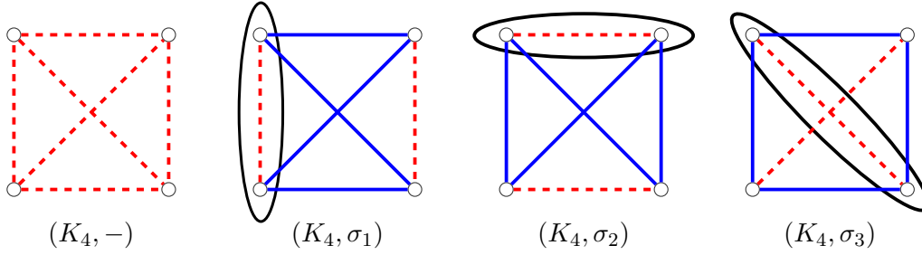
Figure 2.1: A 3-packing of (K_4, -)
