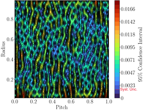
(b) Uncertainty.
