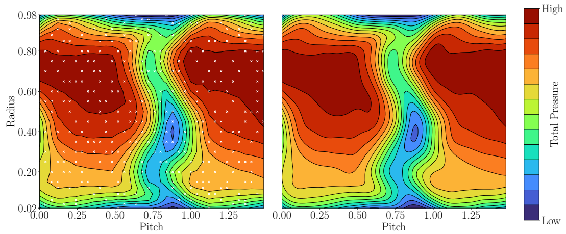
(c) 33% Measurements used. \rho = 0.110 .
