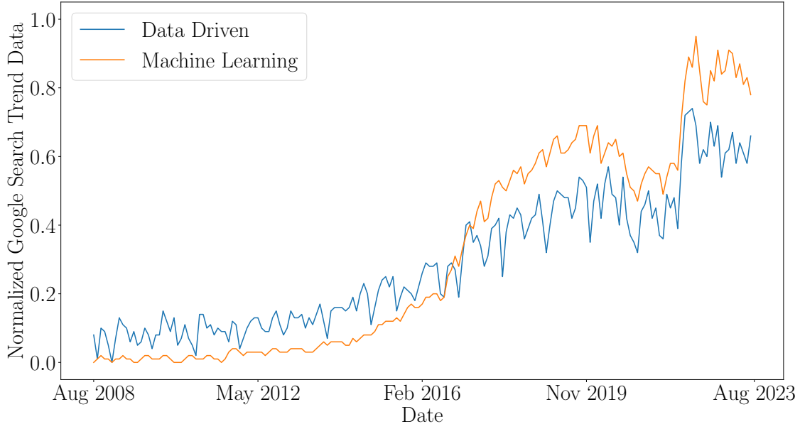
Figure 2.6. Normalized Google search trends evolution over time for the keywords 'machine learning' and 'data driven'. Both keywords follow a similar trend.
