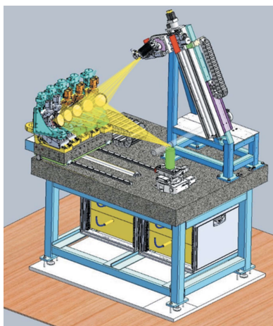
Figure 5.2: Schematic drawing of ROBL's five-crystal X-ray emission spectrometer. Extracted from Scheinost et al. [200]. Figure used with permission from IUCr Journals.
