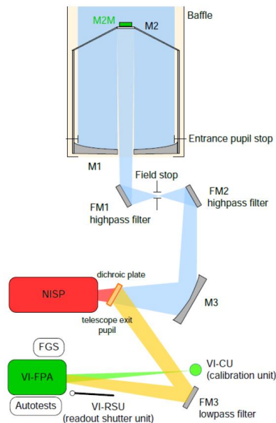
Figure 7: Optical schematic of the Euclid Payload Module (PLM) – Courtesy Airbus Defense and Space [32].
