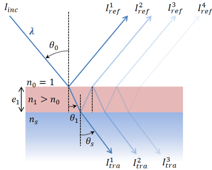
Figure 29: Illustration of rays from multiple reflections and transmissions on a monolayer stack (red) applied to a substrate (blue).
