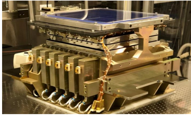
Figure 8: VIS instrument after its integration at CEA-IRFU [Image Credits: CEA]
