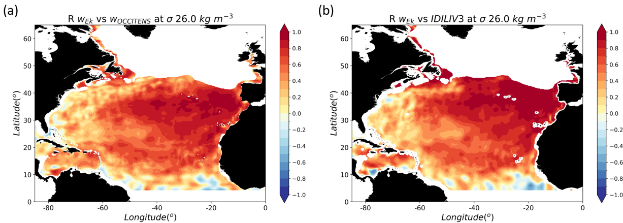
Figure 4.7: Time correlation coefficient between Ekman pumping vertical velocity ( w_{Ek} ) and the model's output (a) and estimated (b) vertical velocity field over \sigma 26 \text{ kg m}^{-3} .
