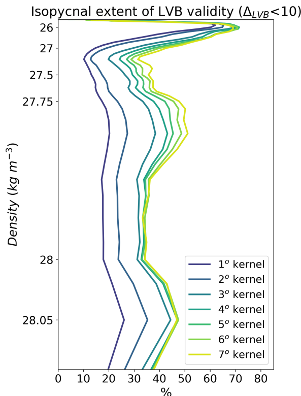
Figure 3.3: 56-year average LVB validity extent (%) over isopycnal levels in the unmasked region outside the 4° belt from the western boundary, as a function of spatial smoothing size from 1 to 7° kernel.
