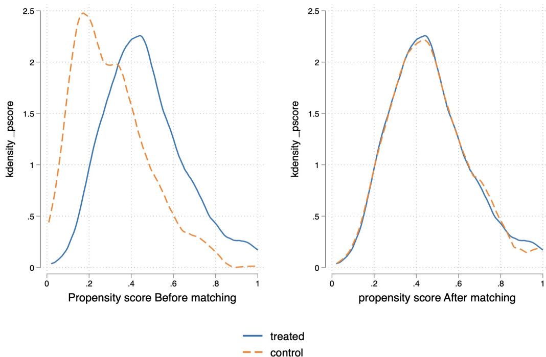
FIGURE 2.5 : Common support before and after matching of treated and controls units
