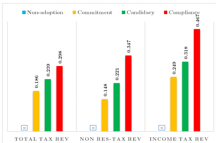
FIGURE 3.4 : The evolution of the estimated fixed-effects coefficients
