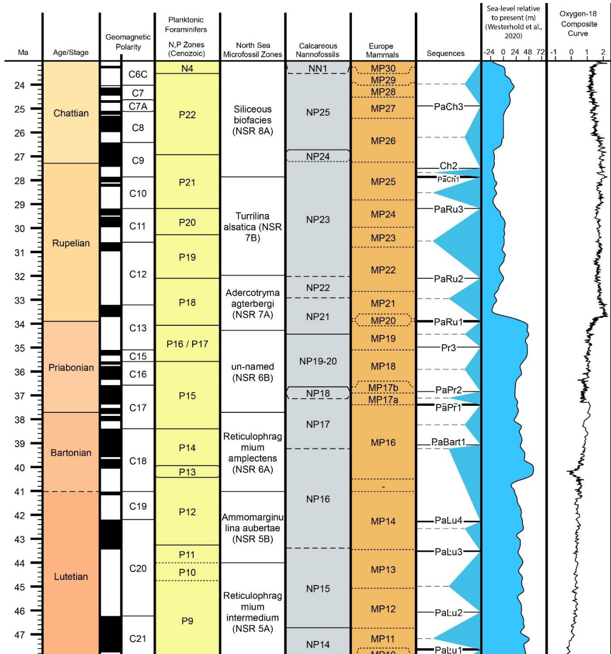
Figure 37: Lutetian-Chattian Geological Time Scale ( Gradstein et al., 2012 ) with corresponding magnetic chrons, planktonic foraminifers' zones, North Sea Microfossil zones, calcareous nannofossils zones, European mammals zones, sea-level sequences, eustasy variations, and oceanic \delta^{18}\text{O} curve. Made with TimeScaleCreator .
