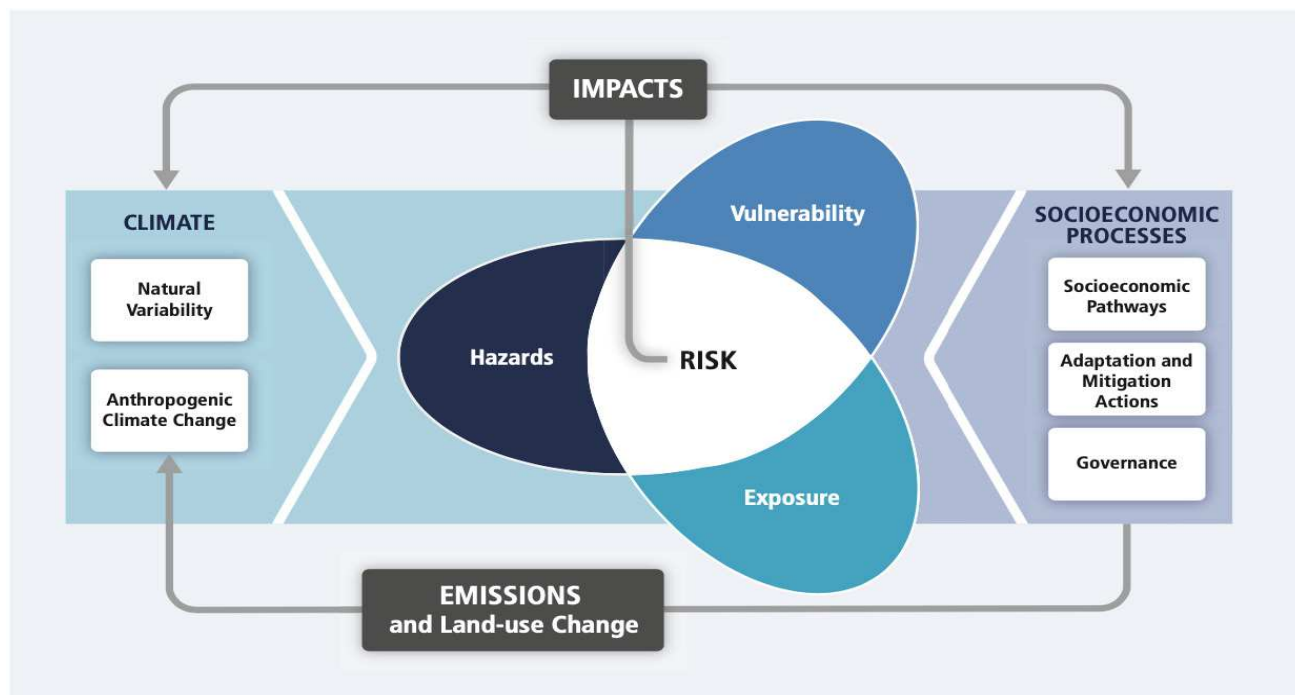
Fig. 2. Illustration of the core concepts of the WGII AR5. Risk of climate-related impacts results from the interaction of climate-related hazards (including hazardous events and trends) with the vulnerability and exposure of human and natural systems. Changes in both the climate system (left) and socioeconomic processes including adaptation and mitigation (right) are drivers of hazards, exposure, and vulnerability. Source: Lavell et al. (2012)
