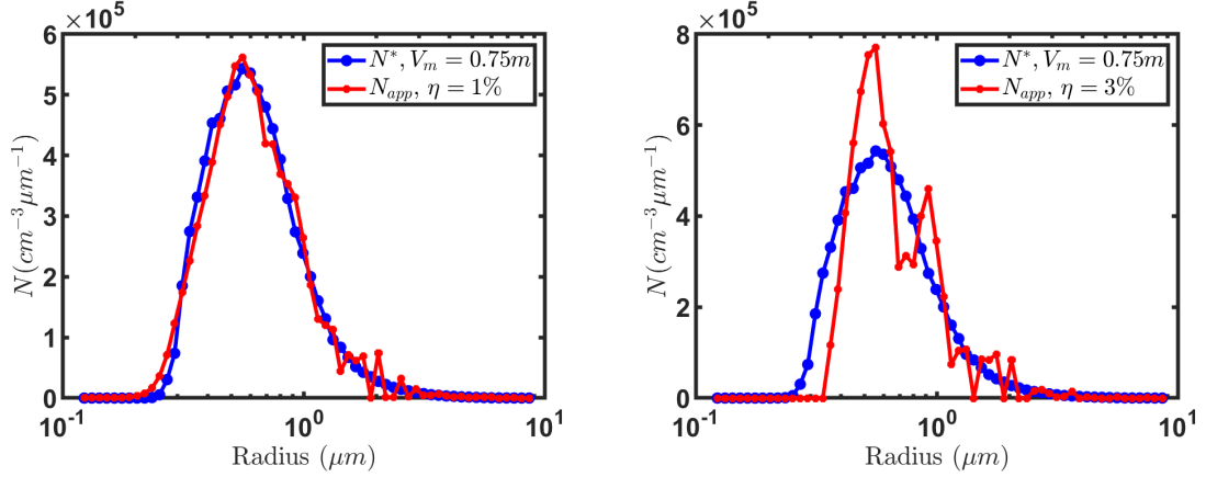
Figure 6.11: Identification results with noise (1% on the left, 3% on the right) in backscattering with anisotropic case.
