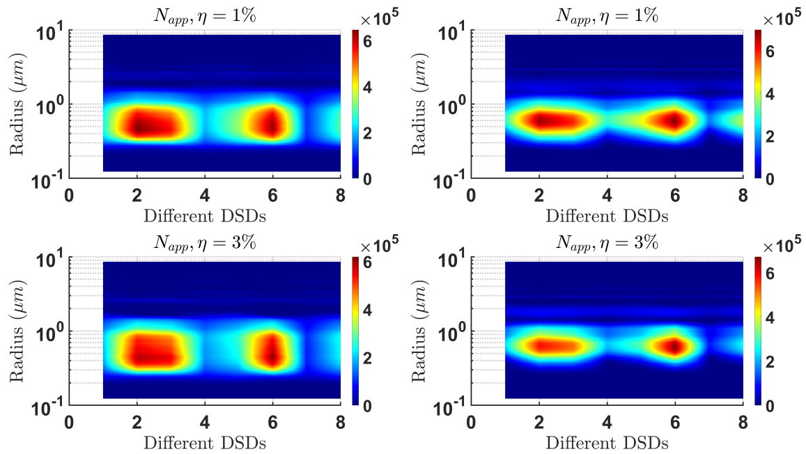
Figure 6.15: Identification results of various PAVIN DSDs, by using a collimated source, obtained with forescattering measurements, isotropic modelling (left), backscattering measurements and isotropic modelling (right) for \eta=1 , and 3\% .
