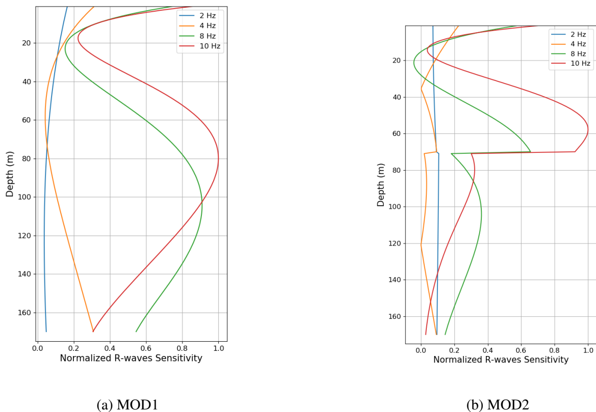
Fig. 4.11 Normalised sensitivity kernel at 2, 4, 8 and 10 Hz, computed for 1D velocity models described in Table 4.1. (a) 170 m of marls (MOD1); (b) 70 m limestone above 100 m of marls. Sensitivity is the partial derivative of R-waves phase velocity with respect to the S-wave velocity.
