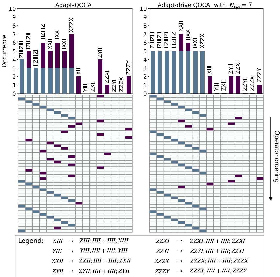
Figure 7.5 Operator occurrence FHM 2 \times 2 . The bar charts represent the number of times the operators in \mathcal{O}_{\text{QOCA}} appear in the circuit built by adapt-QOCA (left) and in adapt-drive QOCA for N_{ops} = 7 (right). The labels on the bar chart are defined in the legend. The 8 first operators (from the left to the right) are the operators of \mathcal{O}_{\text{VHA}} and the 8 following are the operators in \mathcal{O}_{\text{drive}} . The tables below the bar charts show the order in which the operators are added to the PQC along the operator ordering arrow. When a block of VHA is added to the ansatz the 8 first operators on the left are added one after another (in blue). The number of operators added from a VHA block is also indicated in blue in the bar chart.
