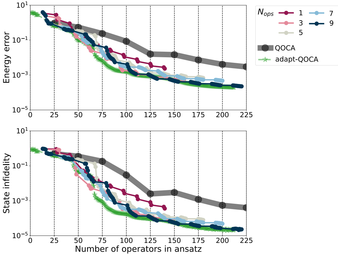
Figure 7.3 Ansatz performance for the 2 \times 3 FHM. Same figure as in Fig. 7.1 for the 2 \times 3 FHM, and with the difference that adapt-drive QOCA was grown with the QOCA pool, and only for odd values of N_{ops} ranging from 1 to 9.
