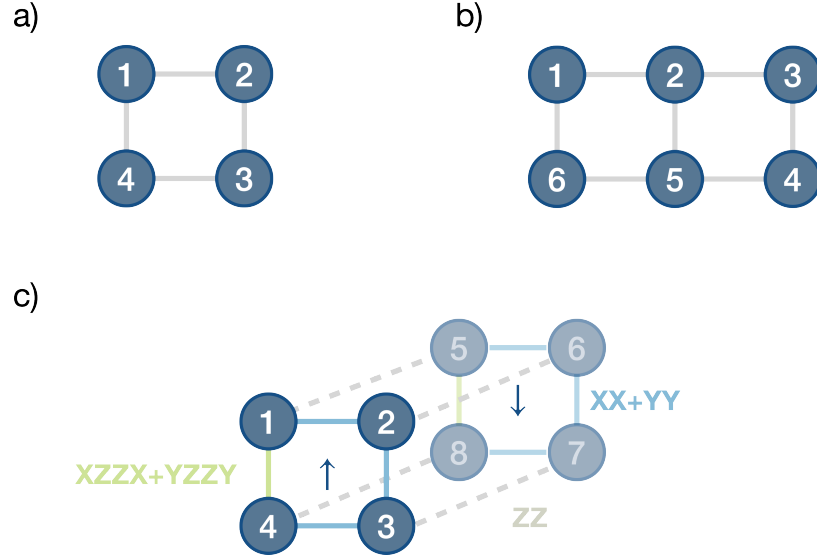
Figure 5.3 FHM lattice sites. Illustration of a) a 2 \times 2 lattice and b) 2 \times 3 lattice, with labeling of the sites. c) Diagram of the qubits representing a 2 \times 2 lattice. The 4 first (last) qubits represent spin up (down) particles. The lines connecting the qubits represent the qubit interaction terms appearing in the Fermi-Hubbard Hamiltonian: ZZ (dashed gray), XX + YY (blue), X_1Z_2Z_3X_4 + Y_1Z_2Z_3Y_4 and X_5Z_6Z_7X_8 + Y_5Z_6Z_7Y_8 (green).
