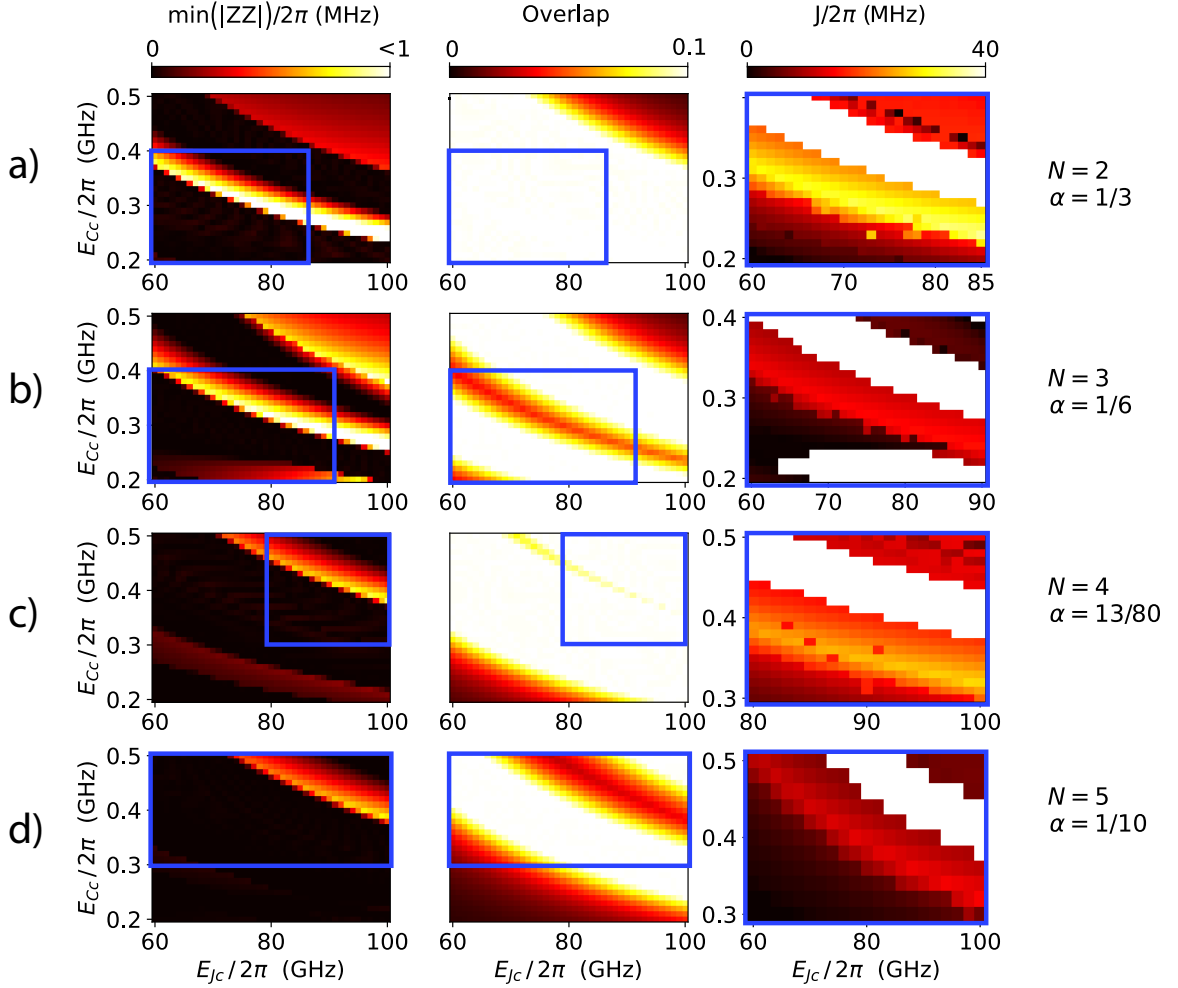
Figure 3.9 Colormap of ZZ , the overlap and J_{ab} versus E_{C_c} and E_{J_c} for multiple (N, \alpha) : a) N = 2 & \alpha = 1/3 , b) N = 3 & \alpha = 1/6 , c) N = 4 & \alpha = 13/80 and d) N = 5 & \alpha = 1/10 . All the colormaps are at the same scale and any value of |ZZ| > 1 MHz is plotted in white. For each N and \alpha , the gate rate is simulated in the regions surround by the blue box in the colormaps of ZZ and of the overlaps. We omit to simulate J_{ab} where the minimum ZZ point is above 0.1 MHz, those points are indicated in white. The qubit and coupling parameters used in this figure are the ones indicated in Eq. (3.56).
