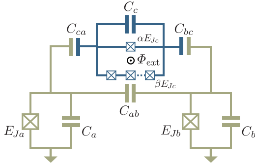
FIG. 8. Circuit schematic and notations used in the derivation of the circuit Lagrangian in Appendix B. The coupler consists of two branches of total capacitances C_\alpha and C_\beta (not indicated in the figure). The \alpha branch consists of a single Josephson junction, while the ‘ \beta ’ branch contains N junctions in series. The bare coupler and transmon modes are connected capacitively through coupling capacitances C_{ab,bc,ca} .
