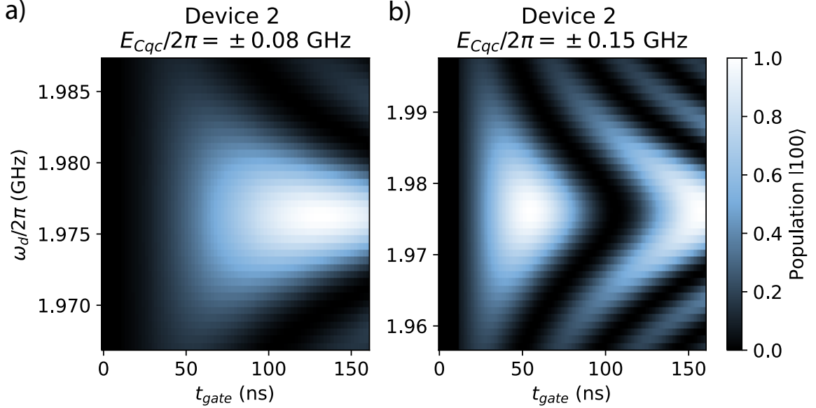
Figure 4.5 Simulation of the population in qubit a versus the pulse time t_{gate} for multiple drive frequencies \omega_d for device 2 with \delta\varphi/2\pi = 0.01 . a) Simulated data using the device parameters in Eq. (4.2) b) Simulated data using the device parameters in Eq. (4.2) but with larger couplings E_{Cbc}/2\pi = -E_{Cac}/2\pi = 0.15 GHz.
