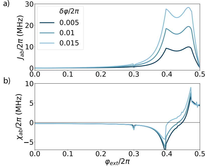
Figure 3.10 a) i SWAP gate J_{ab} rate and b) dynamical ZZ interaction \chi_{ab} versus flux. Each colored line corresponds to a different drive amplitude \delta\varphi/2\pi ranging from 0.005 to 0.015. The two main resonances at \varphi_{ext}/2\pi = 0.4 and 0.4725 correspond to the avoided crossing between the qubits and the coupler. The device parameters used in this figure are the ones indicated in Eq. (3.56).
