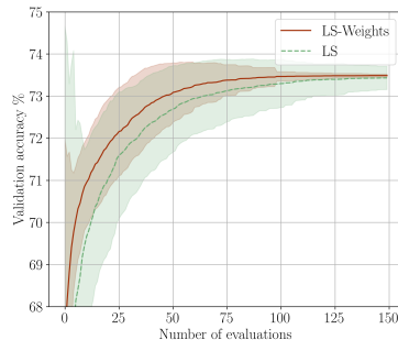
(b) Cifar100
