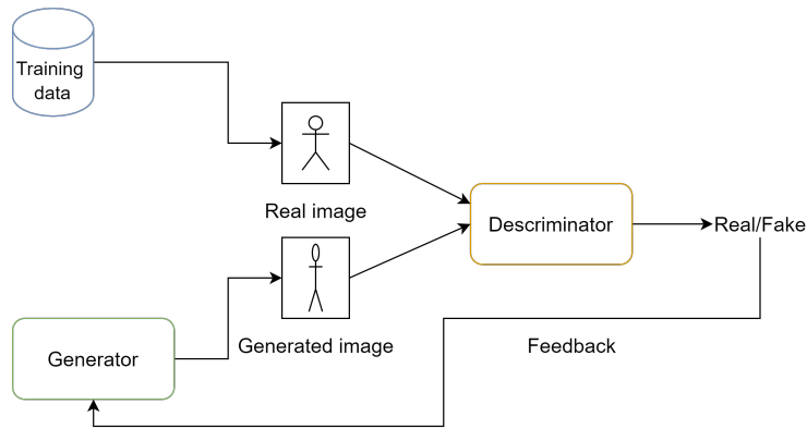
Figure 1.9: GAN representation.
