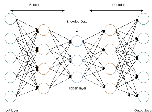
Figure 1.7: Autoencoder.
