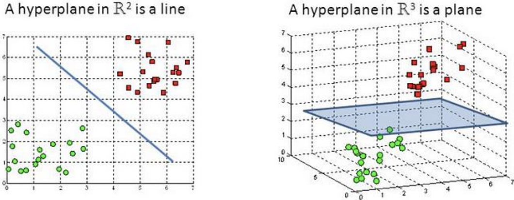
Figure 15: Visualization of SVMs separating the green and red points in a two- and three-dimensions spaces. Taken from [91].
