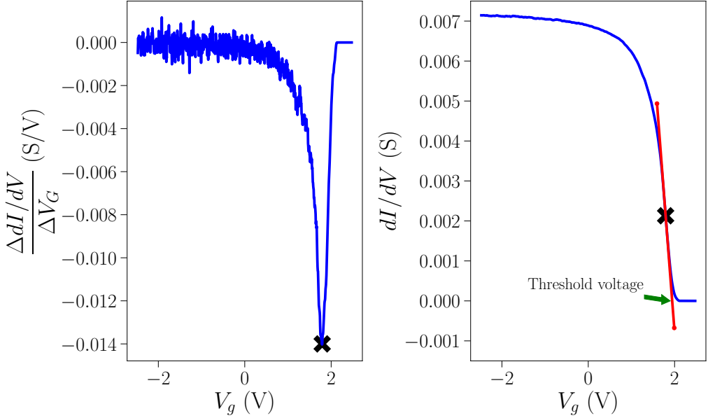
Figure 3.8 – Left: Numerical differentiation of the conductance of the device with L = 500 nm with respect to the gate voltage. The black cross marks the point with the minimum derivative value. Right: The conductance as a function of the gate voltage of the same device. The black cross is locating at the same spot on the horizontal axis. The red line has the same slope as the value in the vertical axis of the figure on the left. The threshold voltage is marked by the green arrow.
