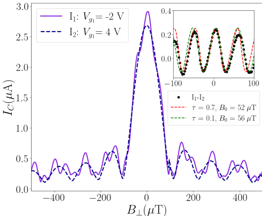
Figure 6.9 – The measured critical current ( I_C ) as a function of the perpendicular magnetic field ( B_\perp ) extracted from the I-V characteristics of the SQUID in Figure 6.2(b) at V_{g2} = -2.0 \text{ V} and V_{g1} equals to: ( I_1 , solid purple) -2 \text{ V} , and ( I_2 , dashed dark blue) 4 \text{ V} . The inset shows the fitting of I_1 - I_2 with the CPR of the short junction model.
