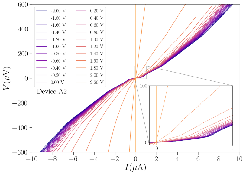
Figure B.2 – Current-voltage ( I - V ) characteristic of the device A2 at different gate voltages ( V_g ).
