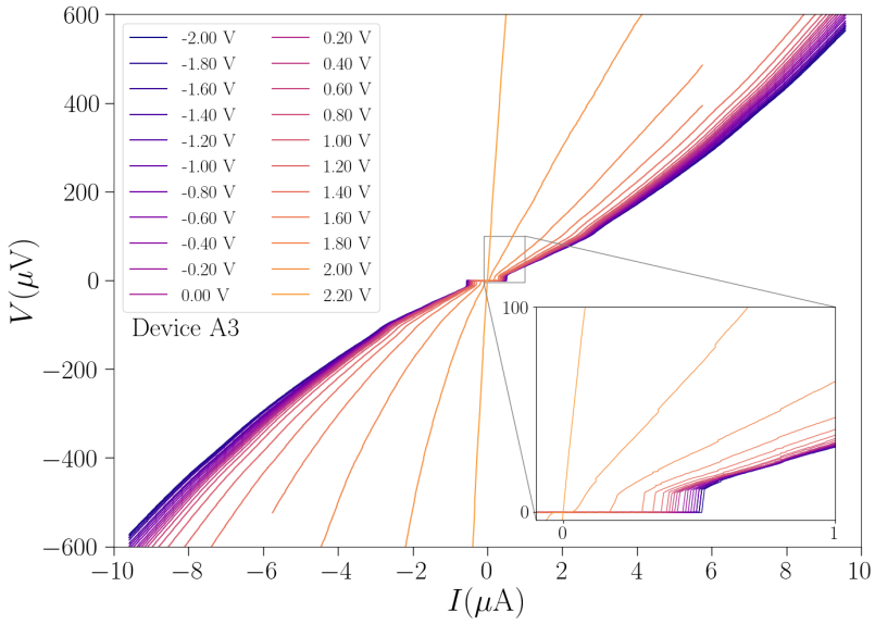
Figure B.3 – Current-voltage ( I - V ) characteristic of the device A3 at different gate voltages ( V_g ).
