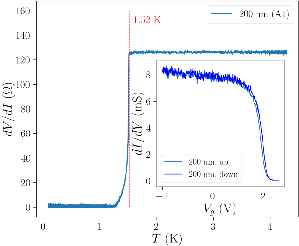
Figure 3.15 – Resistance of the device "A1" as a function of temperature at V_g = -2 V. From the curve, T_C has been estimated to be 1.52 K. The inset shows the pinch-off curve of the device at 4.2 K. There is a small shift in the threshold voltage depending on the direction of voltage ramping.
