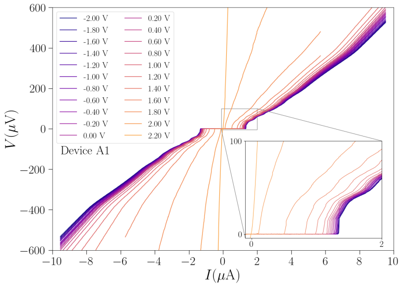
Figure B.1 – Current-voltage ( I - V ) characteristic of the device A1 at different gate voltages ( V_g ).
