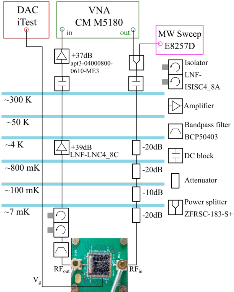
Figure 5.5 – Schematic of the measurement setup for gatemon characterization. The input RF signal is generated by a vector network analyzer (VNA) and passes through several attenuators at different temperatures. The output signal is filtered and amplified before being analyzed by the VNA. The gate voltage is controlled by a digital-to-analog converter (DAC).
