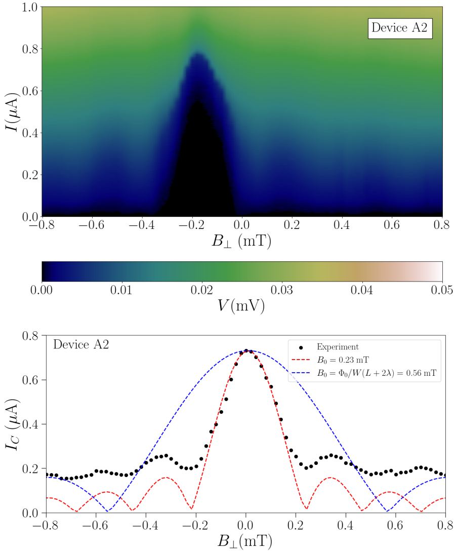
Figure B.15 – (upper) Voltage drop ( V ) across the device A2 as a function of the current ( I ) and the out-of-plane magnetic field ( B_{\perp} ). (lower) Critical current extracted from the colormap above. The Fraunhofer fitting with the extracted critical current is shown by the red dashed line. The period of the Fraunhofer from the fitting is found to be 0.23 mT, in comparison with \Phi_0/W(L + 2\lambda) = 0.56 mT calculated from the junction parameters (blue dashed line).
