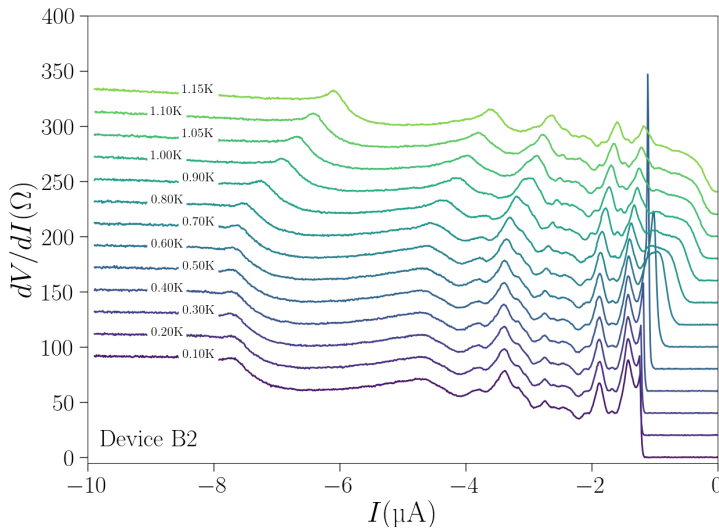
Figure B.12 – Differential resistance ( dV/dI ) of the device B2 as a function of the current ( I ) at different temperatures ( T ) at V_g = -2 V.
