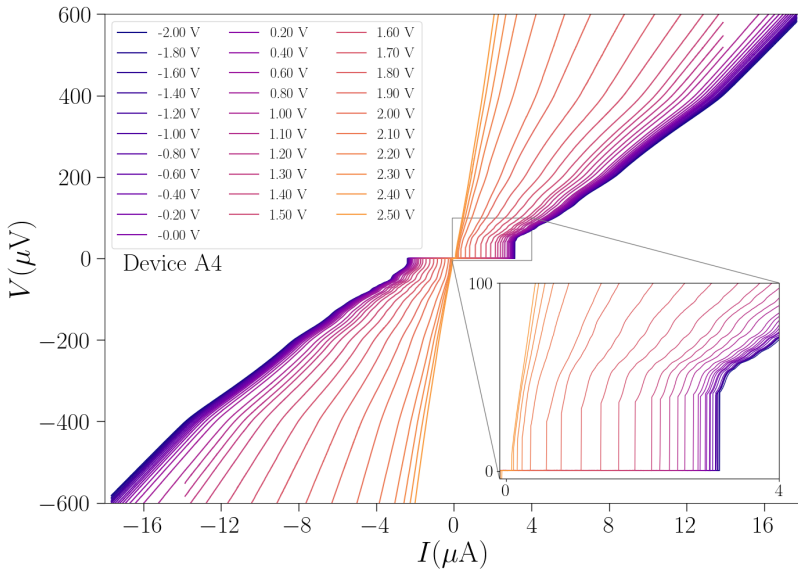
Figure B.4 – Current-voltage ( I - V ) characteristic of the device A4 at different gate voltages ( V_g ).
