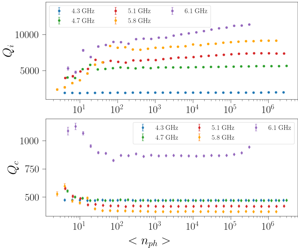
Figure 4.8 – Internal quality factor ( Q_i ) and coupling quality factor ( Q_c ) of the resonators shown in Figure 4.5(b) plotted as a function of the average photon number ( \langle n_{ph} \rangle )
