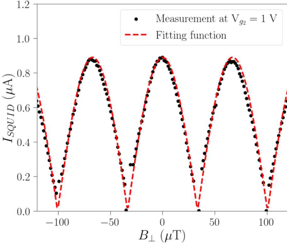
Figure 6.5 – The measured SQUID current ( I_{SQUID} ) is presented as a function of the perpendicular magnetic field ( B_{\perp} ), extracted from the I-V characteristics of the SQUID shown in Figure 6.2(a), under the symmetric regime ( V_{g_1} = -2.0 V and V_{g_2} = 1.0 V). The red dashed line represents the curve fit of the symmetric SQUID equation. The fitting yields a period of 67 \mu\text{T} for the SQUID oscillations.
