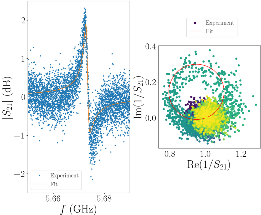
Figure 5.7 – Transmission spectrum of the resonator and the circle fit obtained at P_{VNA} = -40 dBm and an estimated P_{in} below -126 dBm, both at V_g = 0 V.
