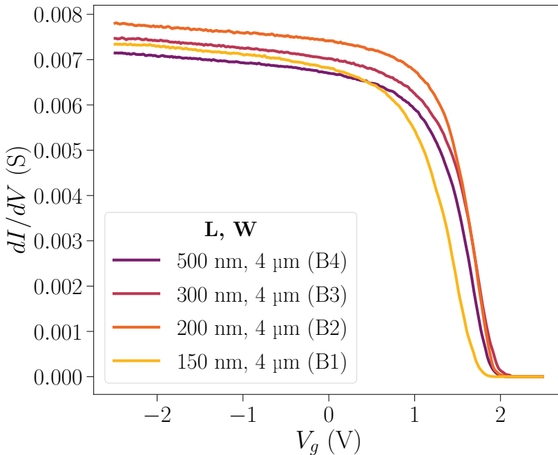
Figure 3.7 – The conductance ( dI/dV ) of four JoFETs with L=150 nm, 200 nm, 300 nm and 500 nm as a function of the gate voltage ( V_g ) at low temperature (4.2 K). This data is obtained at the zero DC voltage applied. The AC voltage applies to the device is 0.5 mV at 77 Hz.
