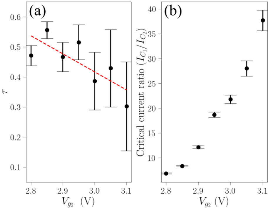
Figure 6.7 – (a) Transparency ( \tau ) of the junction as a function of the gate voltage ( V_{g_2} ). The uncertainty of the fit is indicated by the error bars in the figure. The transparency exhibits a decreasing trend with increasing gate voltage. (b) Critical current ratio ( I_{C_1}/I_{C_2} ) as a function of V_{g_2} .
