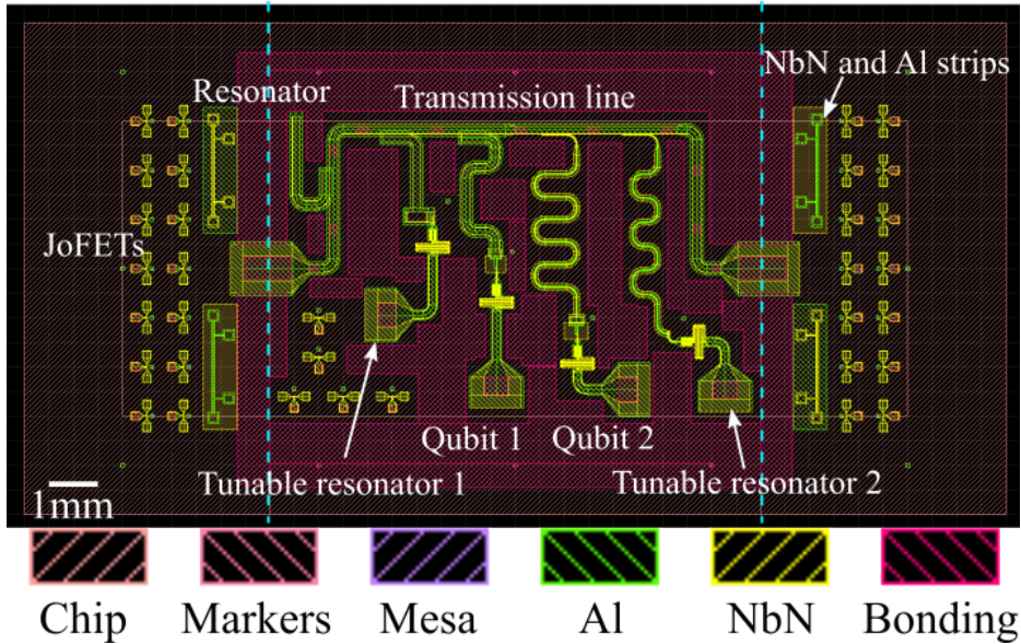
Figure 5.1 – GDS design of the sample is shown in the figure. The design includes an NbN transmission line coupled to the NbN resonator, Tunable resonator 1, Tunable resonator 2, Qubit 1, and Qubit 2. Additionally, there are several JoFETs, NbN strips, and Al strips on the sides to perform DC characterization tests. The color patterns in the design represent different lithography layers, as indicated in the figure.
