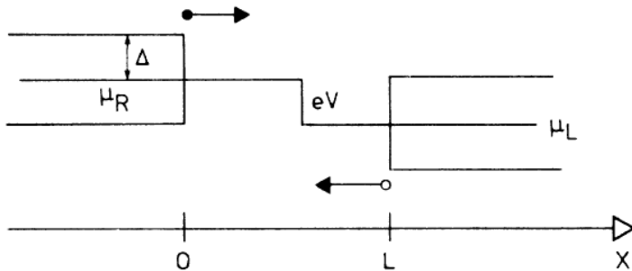
Figure 3.30 – Schematic diagram of the S-N-S junction in this model. The figure shows chemical potential of the leads ( \mu_R , and \mu_L ), superconducting gap ( \Delta ), voltage bias between two leads ( eV ), and an electron moving to the right and a hole moving to the left. The potential barriers " H\delta(x) " are located at x = 0 , and L . The figure is reproduced from [82].
