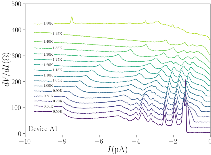
Figure B.9 – Differential resistance ( dV/dI ) of the device A1 as a function of the current ( I ) at different temperatures ( T ) at V_g = -2 V.
