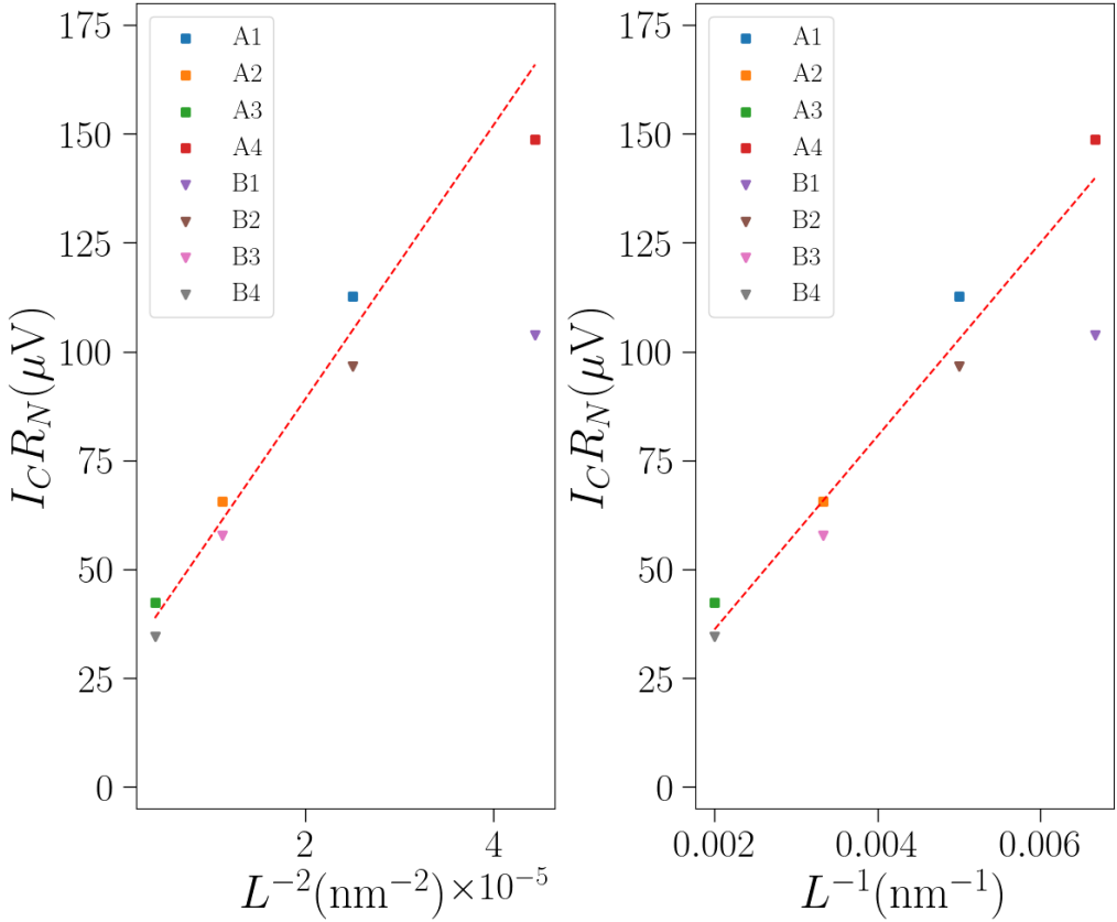
Figure 3.20 – I_C R_N as a function of: (left) the inverse of the square of the junction length ( L^{-2} ), and (right) the inverse of the junction length. Both curves show the I_C R_N decreasing when the junction length becomes longer.
