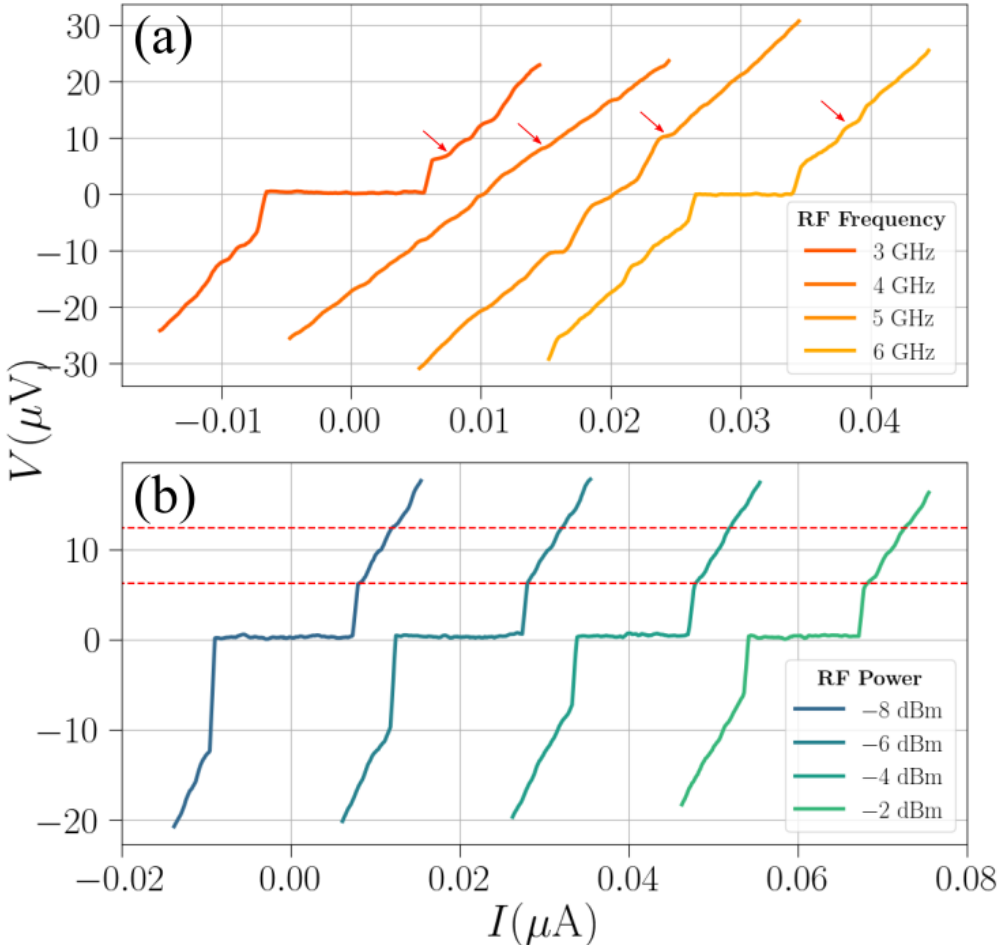
Figure 6.11 – (a) I-V characteristics of an asymmetric SQUID ( L_1 = 200 nm, L_2 = 200 nm, W_1 = 1 \mu\text{m} , W_2 = 5 \mu\text{m} , S = 4 \times 4 \mu\text{m}^2 , V_{g1} = 2.2 V, V_{g2} = 4 V) based on SiGe heterostructure as a function of radiated microwave frequencies. The applied microwave power at the generator is set to be -3 dBm. (b) I-V characteristics of the same SQUID as a function of applied microwave powers. The microwave frequency is fixed at 3 GHz.
