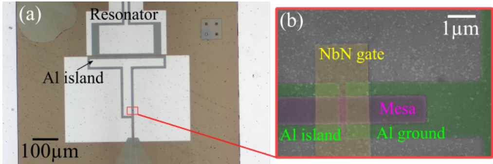
Figure 5.3 – (a) Optical image of the gatemon qubit consists of an Al island and an Al-Ge-Al junction with NbN top gate. The island is coupling capacitively to the resonator through the metal pad visible in the image. (b) False-colored SEM image of the junction.
