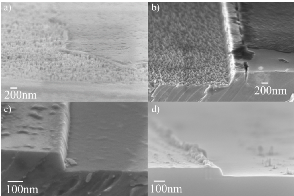
Figure 2.7 – Tilted-angle SEM images. a , Gas: 50 sccm \text{Cl}_2 , 5 sccm \text{O}_2 , 12 sccm \text{N}_2 . ICP power 50 W/ bias power 20 W. Etching time: 2+2 minutes. b , Step 1) Gas: 50 sccm \text{CF}_4 . ICP power 1000 W/ bias power 100 W. Etching time: 10 s. Following by step 2) Gas: 50 sccm \text{Cl}_2 , 5 sccm \text{O}_2 , 12 sccm \text{N}_2 . ICP power 50 W/ bias power 20 W. Etching time: 5 minutes. c , Gas: 50 sccm \text{CF}_4 . ICP power 1000 W/ bias power 100 W. Etching time: 10 s. d , Gas: 10 sccm \text{CF}_4 , 40 sccm Ar. ICP power 200 W/ bias power 25 W. Etching time: 30 s.
