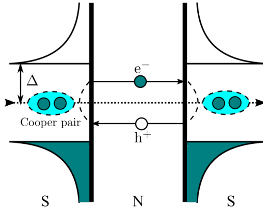
Figure 3.4 – Schematic of the energy band diagram of a superconductor-normal-superconductor (S-N-S) junction. The figure shows the superconducting gap ( \Delta ) in the density of states of the superconducting leads that open below T_C , and the quasiparticles (Cooper pairs, electrons, and holes) confining in the Andreev bound states.
