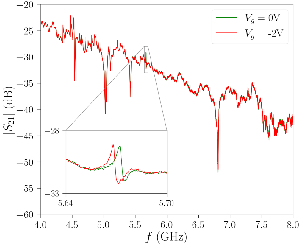
Figure 5.6 – Magnitude of the transmission coefficient |S_{21}| in the frequency range between 4 and 8 GHz at gate voltages of 0 V and -2 V. The inset shows a zoomed-in view of the transmission data specifically for the resonator of Qubit 2.
