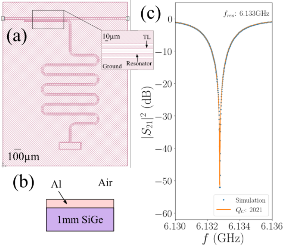
Figure 4.2 – (a) A design, consisting a superconducting resonator coupling to a transmission line, implemented in SONNET simulation software. (b) Schematic depicting the cross-section of the layer in (a). (c) Simulation result showing resonance at 6.133 GHz with a coupling quality factor ( Q_c ) of 2021.
