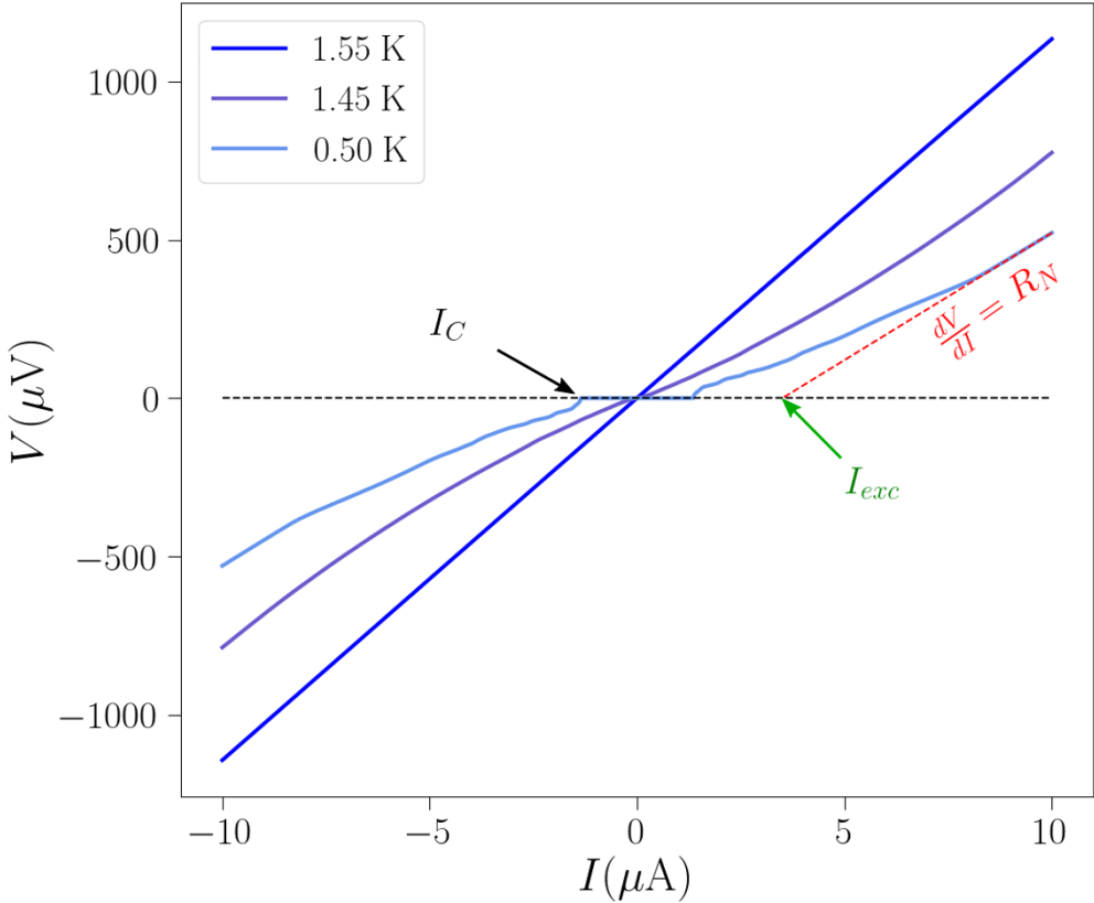
Figure 3.16 – Current-voltage characteristic of the JoFET "A1" with a junction length of 200 nm and a junction width of 4 \mu\text{m} at the gate voltage of -2 V and the temperature of 1.55 K (blue), 1.45 K (violet), and 0.50 K (light blue). The plateau in the light blue curve represents the zero-resistance state, which indicates the flow of the non-dissipative current. The zero-resistance state disappears in the violet curve due to the suppression of the proximity effect in germanium when the temperature is close to T_C of aluminum. When the temperature goes above T_C of aluminum, the aluminum leads change from superconducting to normal, which makes the resistance go up in the blue curve. The critical current ( I_C ) is defined by the current at the switching point of the zero-resistance state. The slope when V > 2\Delta defines the normal state resistance ( R_N ). The excess current ( I_{exc} ) is the intercept between this slope and the horizontal axis.
