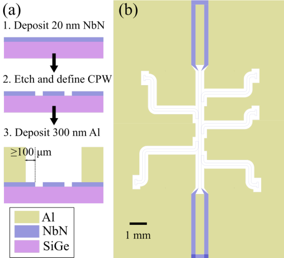
Figure 4.4 – Schematic illustrating the fabrication process of NbN resonators. (a) The process flow comprises the following steps: (1) Deposition of a 20 nm NbN layer. (2) ICP etching to define the coplanar waveguide (CPW). (3) Deposition of a 300 nm Al layer for bonding pads. (b) A graphical design system (GDS) layout corresponding to the process flow depicted in (a).
