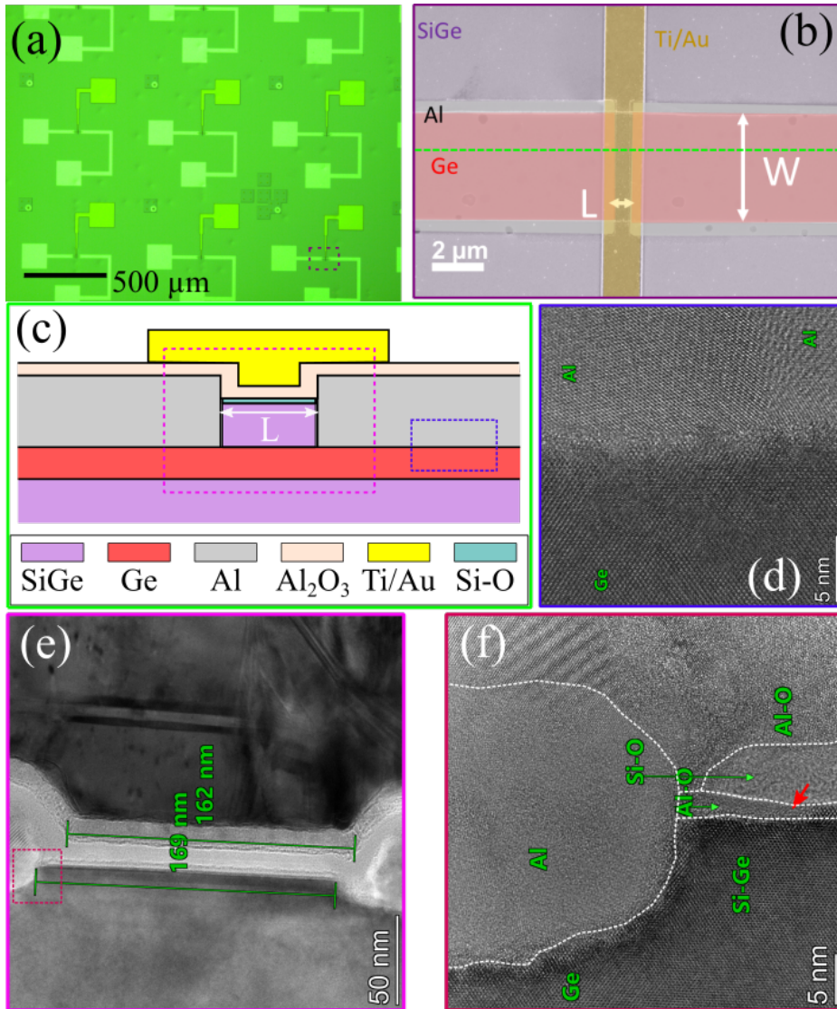
Figure 3.5 – (a) An optical microscope image of the chip we measured (b) a false-colored SEM image of a JoFET device at the junction showing Al leads on a Ge channel with a Ti/Au top gate. The junction length is defined by the space between two ohmic contacts ( L ), and the junction width ( W ) is defined by the lateral dimension of the mesa. (c) Schematic of the device A germanium quantum well (QW) (red) is capped between two barriers of SiGe layers (purple). The source and drain aluminum contacts (gray) are connected to the QW. (d) a TEM image of the area in the blue box in (c) showing direct contact between Al and Ge. (e) a TEM image of the area in the magenta box in (c) showing the gate stack. (f) a TEM image showing the zoom-in of the area in the maroon box in (e) showing the components of the gate stack. Subfigures (d), (e), and (f) are produced by J. L. Lábár and I. Levente [EK MFA, Budapest, Hungary].
