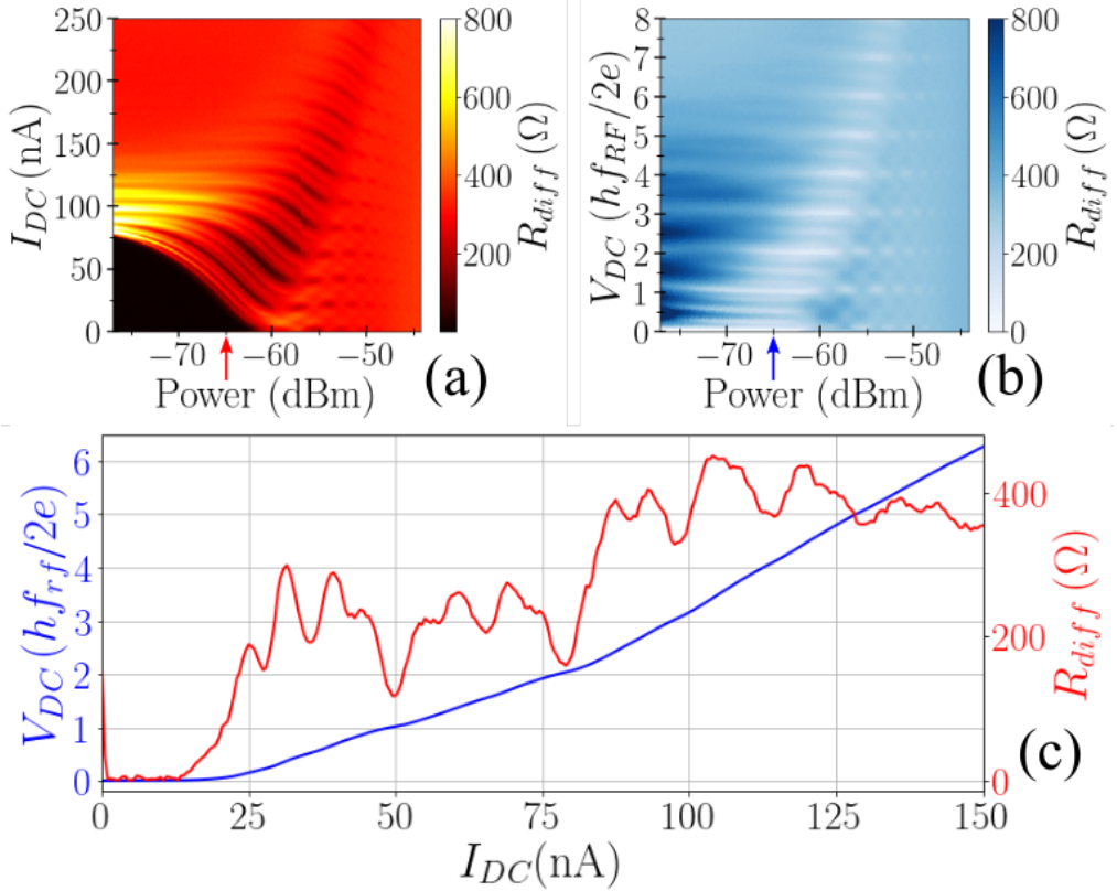
Figure 6.13 – (a) The DC current ( I_{DC} ) as a function of differential resistance ( R_{diff} ) and microwave powers of the device in Figure 6.2(d) at V_{g1} = -2 V, and V_{g2} = 2 V. (b) The normalized DC voltage ( V_{DC} in a unit of hf_{RF}/2e ) as a function of R_{diff} and microwave powers from the same device. (c) (blue) I-V characteristic, and (red) R_{diff} versus I_{DC} at the microwave power of -65 dBm. [A. Leblanc, a doctoral student in the lab].
