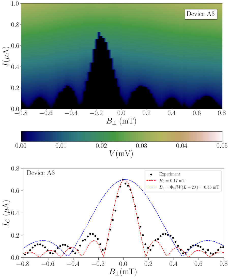
Figure B.16 – (upper) Voltage drop ( V ) across the device A3 as a function of the current ( I ) and the out-of-plane magnetic field ( B_{\perp} ). (lower) Critical current extracted from the colormap above. The Fraunhofer fitting with the extracted critical current is shown by the red dashed line. The period of the Fraunhofer from the fitting is found to be 0.17 mT, in comparison with \Phi_0/W(L + 2\lambda) = 0.46 mT calculated from the junction parameters (blue dashed line).
