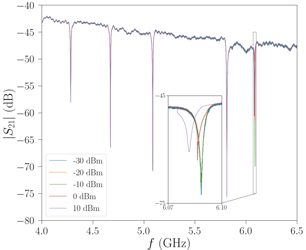
Figure 4.6 – The magnitude of the transmission ( |S_{21}| ) of the sample depicted in Figure 4.5(b) is shown as a function of frequency ( f ) at various VNA power levels. Five resonances corresponding to resonators positioned at 4.28, 4.67, 5.09, 5.81, and 6.09 GHz are observed. The inset illustrates the frequency shift of the 6.09 GHz resonator with changing VNA power. The measurement temperature is set at 10 mK.
