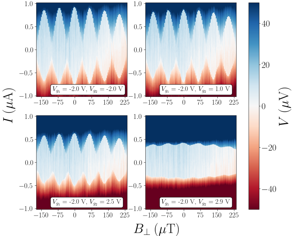
Figure 6.4 – The voltage drop ( V ) across the SQUID device depicted as a function of the out-of-plane magnetic field ( B_{\perp} ) and the current ( I ) at the gate voltage of the first junction set at -2.0 V. The gate voltage applied to the second junction is varied as follows: (upper left) -2.0 V, (upper right) 1.0 V, (lower left) 2.5 V, and (lower right) 2.9 V. The skewness of the interference pattern is observable in the two lower panels of the figure.
