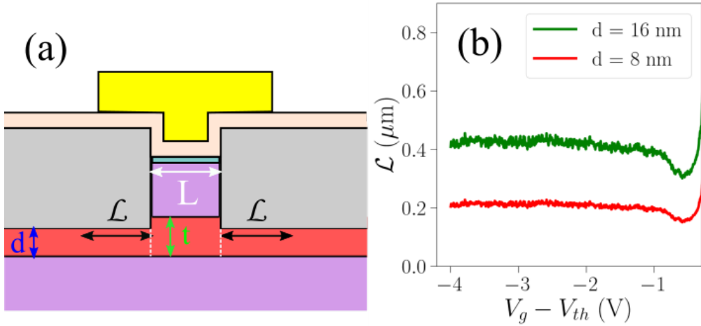
Figure 3.13 – Schematic diagram of the contact resistance model depicts the side view of the device and labels the junction length ( L ), the effective contact length ( \mathcal{L} ) and the quantum well thickness (full: t and etched: d ).
