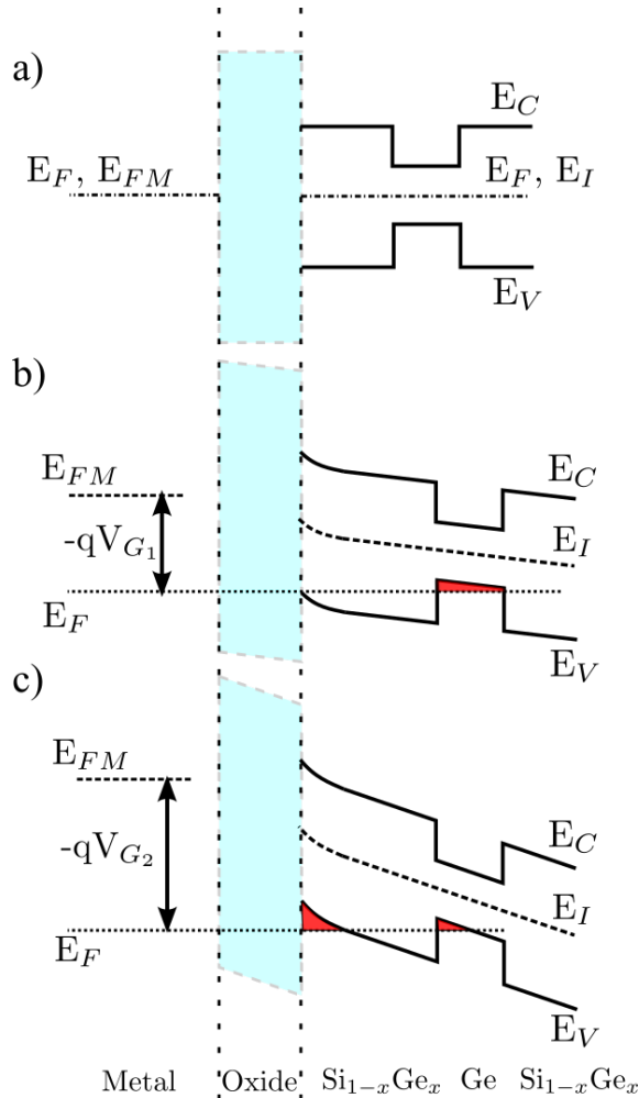
Figure 3.12 – Schematic of the band diagram of the device in three different situations. a) Not connected: The Fermi level of the metal and the semiconductor are independent. There are confinement energy levels in the conduction band and the valence band of the quantum well due to the band gap difference. b) Accumulation: The energy band of the oxide and the semiconductor are bent due to the voltage applied on the metal. There are carriers above the Fermi level confined in the quantum well participating in the conduction. c) Saturation: When the negative voltage is applied on the gate until a certain point, the energy levels at the interface due to the band bending start to become lower than those in the quantum well. Hence, the carriers can tunnel from the quantum well and be accumulated at these energy levels. Since the carriers confined in these levels are not participating in the conduction, the carrier density is saturated and the square resistance measured start to level off. ( From the diagram: E_F is the Fermi level of the device, E_{FM} is the energy level of the metal with respect to the Fermi level, E_I is the Fermi level in the intrinsic semiconductor, E_C and E_V are the conduction band and the valence band of the semiconductor, and V_{G_{1,2}} are the gate voltages applied on the metal.)
