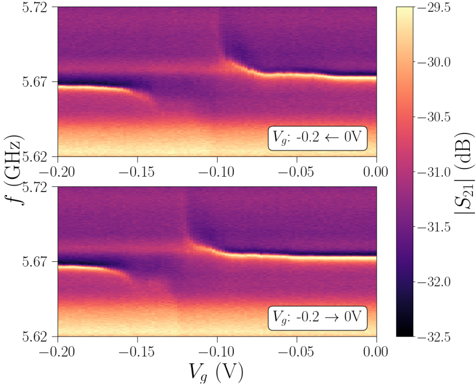
Figure 5.10 – Magnitude of |S_{21}| plotted as a function of frequency and gate voltage at P_{VNA} = -30 dBm. The measurement exhibits a noticeable shift in the anticrossing feature when the direction of voltage ramping is reversed.
