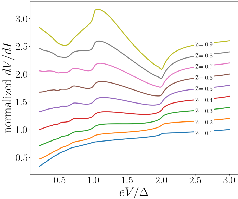
Figure 3.32 – Differential resistances ( dV/dI ) as a function of normalized voltage bias ( eV/\Delta ) at T = 0.25T_C for various value of Z .
