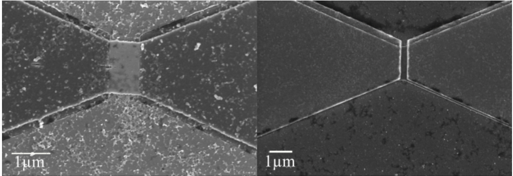
Figure 2.9 – SEM images of the devices, zooming at the junctions, taken after the ohmic contacts step. The junction in the left (right) image has been etched by gluing the sample to a Si carrier wafer using Crystalbond (CGR7016) as an adhesive material. The rest of the etching process is similar.
