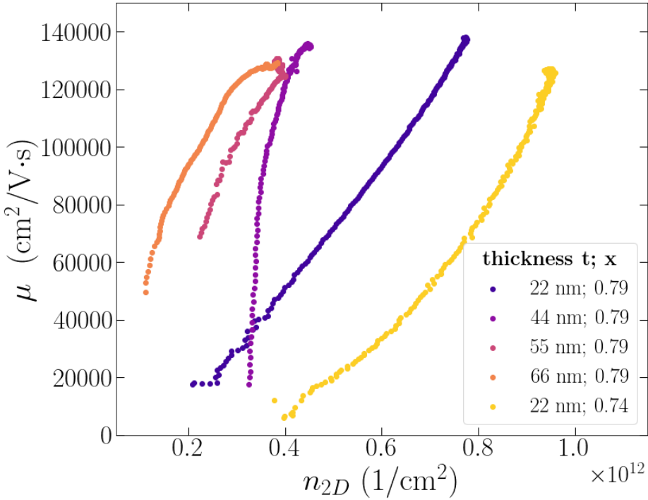
Figure 2.2 – Hole mobility ( \mu ) as a function of the two-dimensional carrier density ( n_{2D} ) obtained from the Hall measurement. The plot shows the data from the Hall bars made in the wafers of the SiGe heterostructures with the different concentrations ( x ) and the different thicknesses ( t ) [E. Kiyooka, a doctoral student in the lab].
