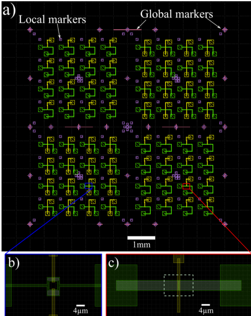
Figure 2.3 – a , GDS design contains global markers, local markers, and devices (JoFETs and SQUIDs). Global markers are on the side and are used for associating the chip coordinate with the GDS coordinate. Local markers are located next to each device. b , an example of SQUID's design with two junctions in parallel. c , an example of JoFET's design with one junction
