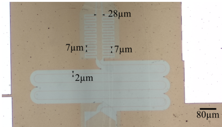
Figure 5.4 – Optical image of the low-pass LC filter. The filter includes a finger capacitor, which contributes to the capacitance, and an NbN meander, which contributes to the kinetic inductance. The geometry of the filter results in a calculated cutoff frequency of 1.1 GHz.
