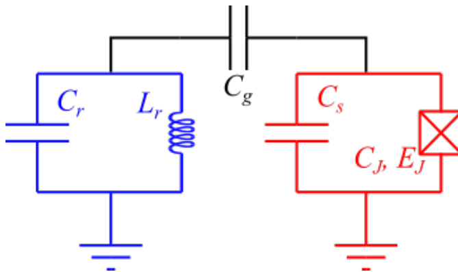
Figure 1.3 – Schematic of a transmon coupled to a resonator via a capacitor C_g . The Josephson junction in the transmon is shunted by a capacitor with a capacitance much larger than the junction capacitance ( C_s \gg C_J ). Coupling interaction causes a dispersive shift in the resonator’s frequency depending on the state, |0\rangle or |1\rangle , of the transmon.
