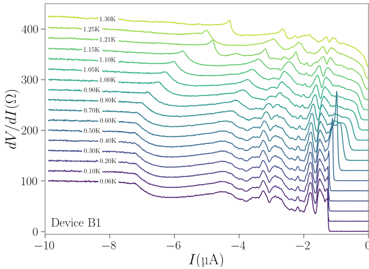
Figure B.11 – Differential resistance ( dV/dI ) of the device B1 as a function of the current ( I ) at different temperatures ( T ) at V_g = -2 V.
