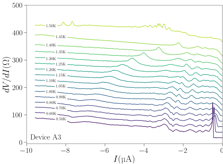
Figure B.10 – Differential resistance ( dV/dI ) of the device A3 as a function of the current ( I ) at different temperatures ( T ) at V_g = -2 V.
