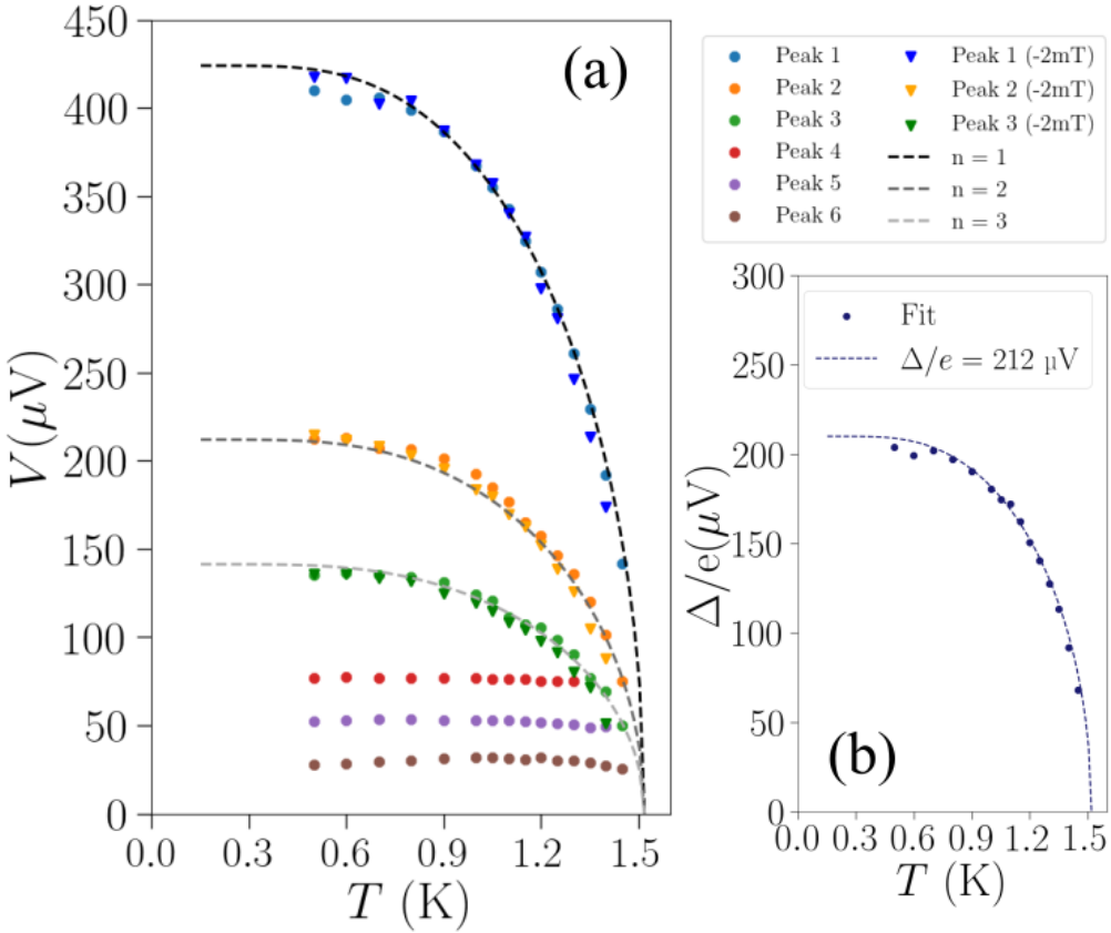
Figure 3.27 – (a) The measurement of the temperature dependence of the position in the voltage of the sub-gap features (Peak 1, Peak 2, Peak 3, Peak 4, Peak 5, and Peak 6) extracted from the curves in Figure 3.25, and Figure 3.26. (b) The derived superconducting gap ( \Delta ) as a function of the temperature ( T ). The dashed lines in the figure represent the behavior of the superconducting gap according to Equation 3.11.
