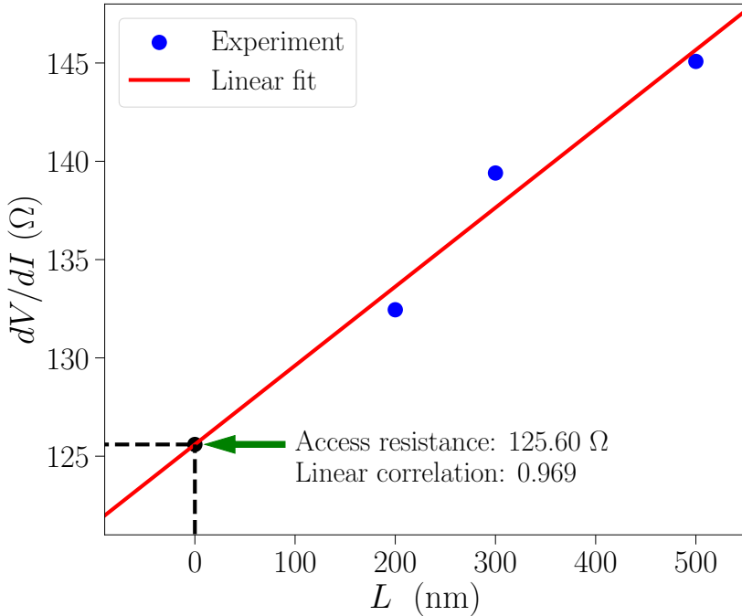
Figure 3.10 – The fitting method corresponds to the equation 3.5. The blue scattered points represent the resistance data from Figure 3.9 at the V_g - V_{th} = -2 V. It has been assumed that the junction lengths follow the lengths in the lithography design. The linear regression of the data is shown by the red line, and the access resistance is represented by the black dot in the figure.
