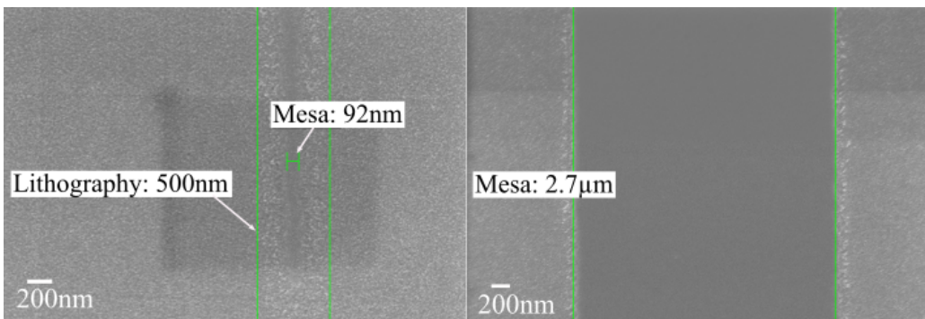
Figure 2.6 – SEM images of the mesa fabricated by the wet etching using a solution of HF:HNO 3 :H 2 O in the proportion of 20:52:40. The mesa in the left (right) image is designed to be 500nm (3 \mu\text{m} ) wide.
