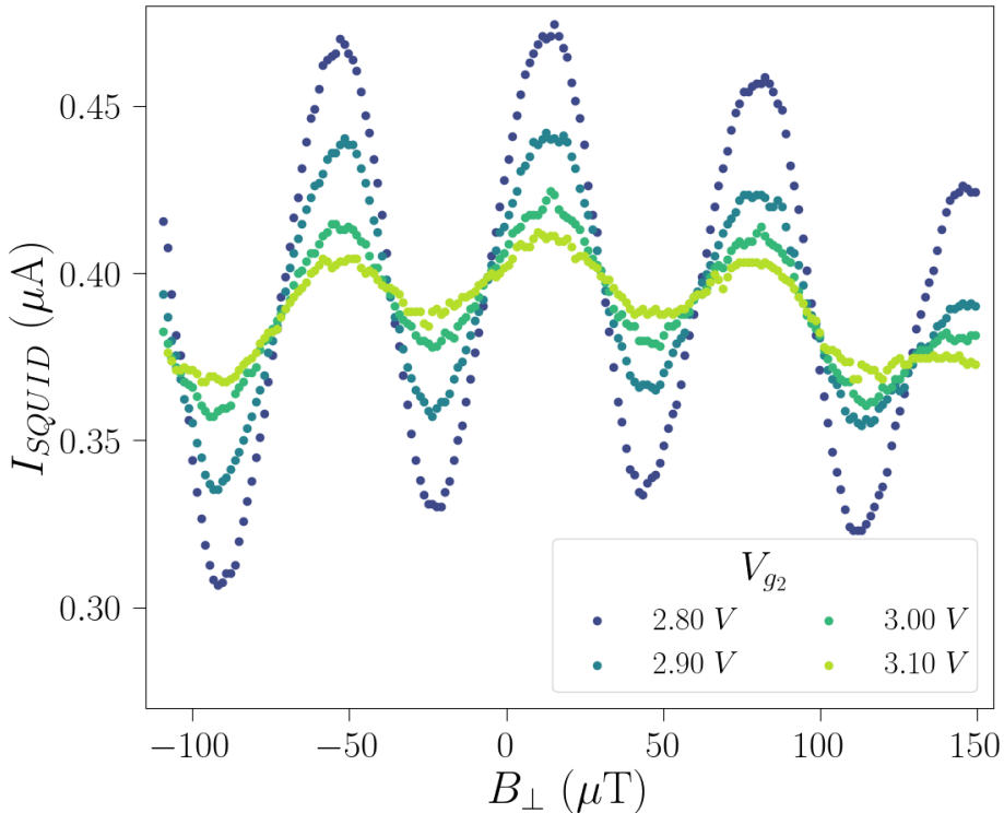
Figure 6.6 – The measured SQUID current ( I_{SQUID} ) is plotted as a function of the perpendicular magnetic field ( B_{\perp} ), extracted from the I-V characteristics of the SQUID shown in Figure 6.2(a) at V_{g_1} = -2.0 V and V_{g_2} ranging from 2.8 to 3.1 V.
