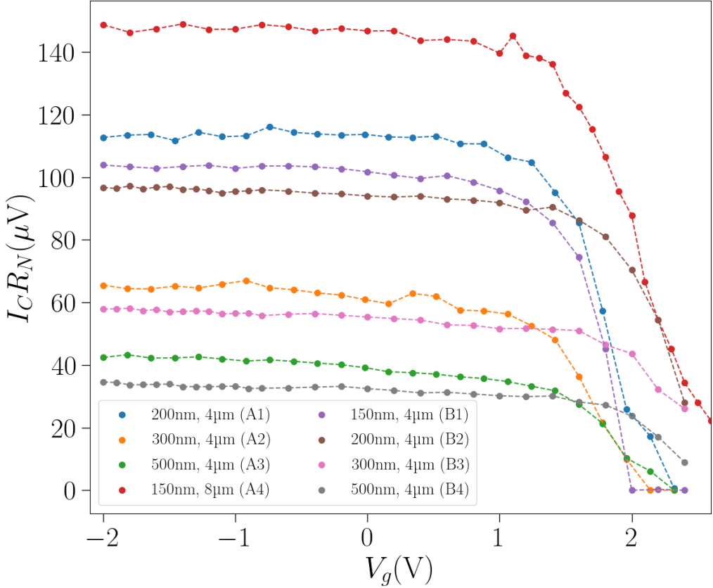
Figure 3.19 – The " I_C R_N " product calculated from the extracted value in Figure 3.18.
