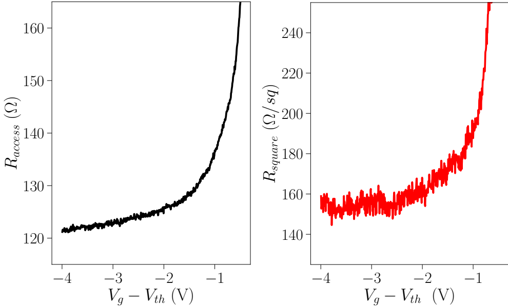
Figure 3.11 – Access resistance of the devices ( Left ), and square resistance of the germanium 2DHG ( Right ) extracted from the data of the resistance as a function of the gate voltage obtained from the devices with junction lengths of 200 nm, 300 nm and 500 nm using linear regression method.
