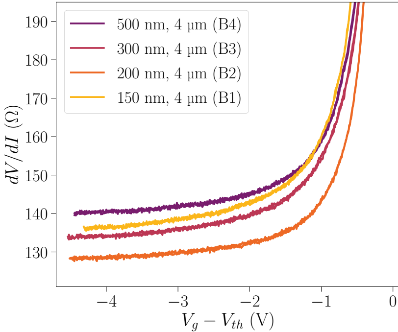
Figure 3.9 – Resistance as a function of the gate voltage with respect to the threshold. The colors and the labels in the legend indicate the junction lengths of the device by the lithography design.
