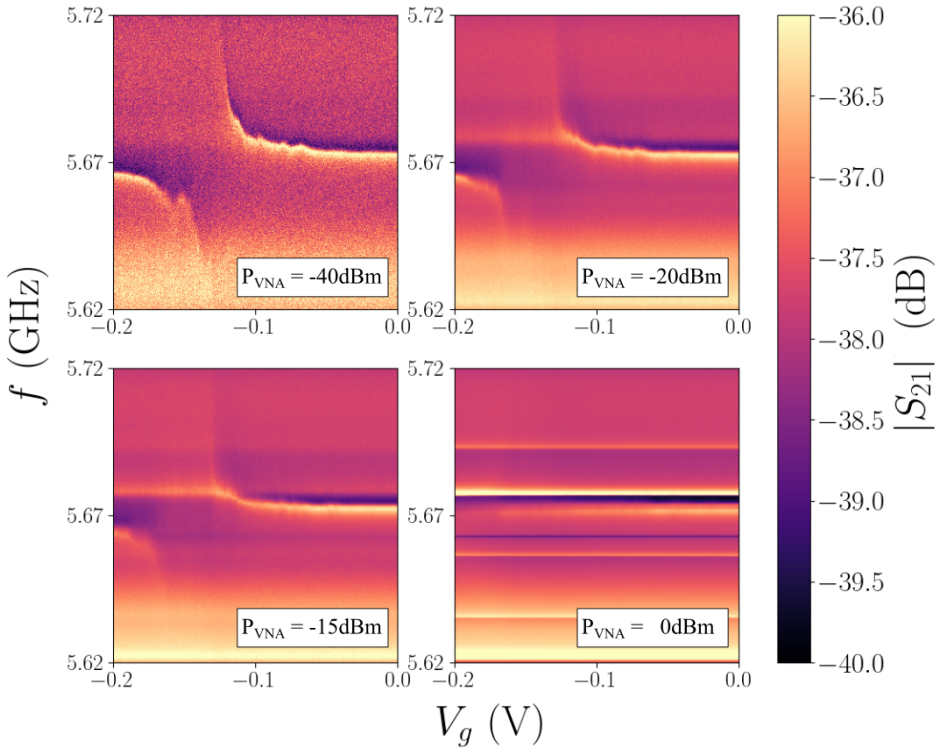
Figure 5.9 – Magnitude of |S_{21}| plotted as a function of frequency and gate voltage at different P_{VNA} values. The anticrossing branch is most visible at the lowest input power ( P_{VNA} = -40 dBm). As the power increases, the visibility of the anticrossing feature diminishes, and it eventually disappears when P_{VNA} = 0 dBm.
