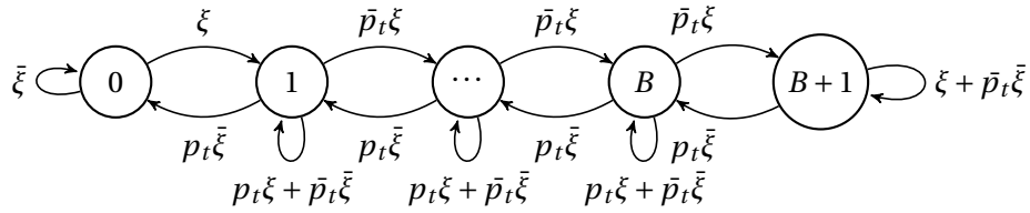
Figure 4.5 – DTMC model of the typical BS with a finite buffer length.
