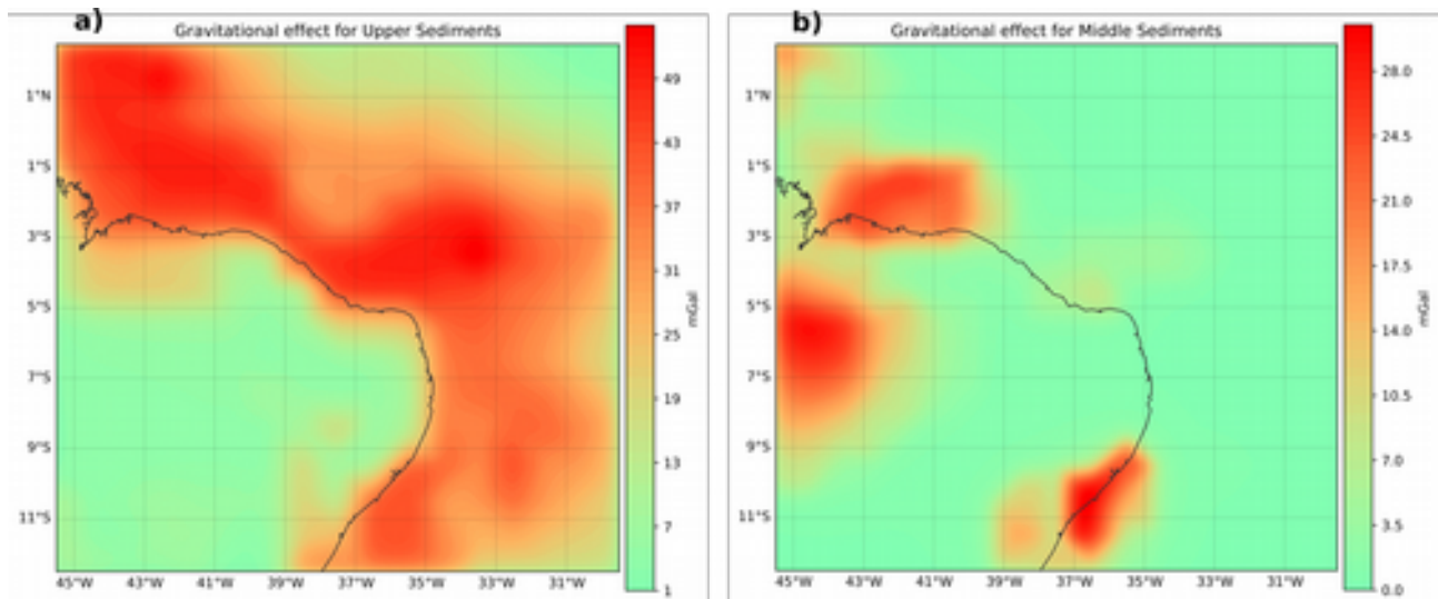
Figure 5.1.5.9 – Gravitational effect of each sediment layer (mGal). a) Gravitational effect of the Upper sediment layer (mGal); b) Gravitational effect of the Middle sediment layer (mGal)
