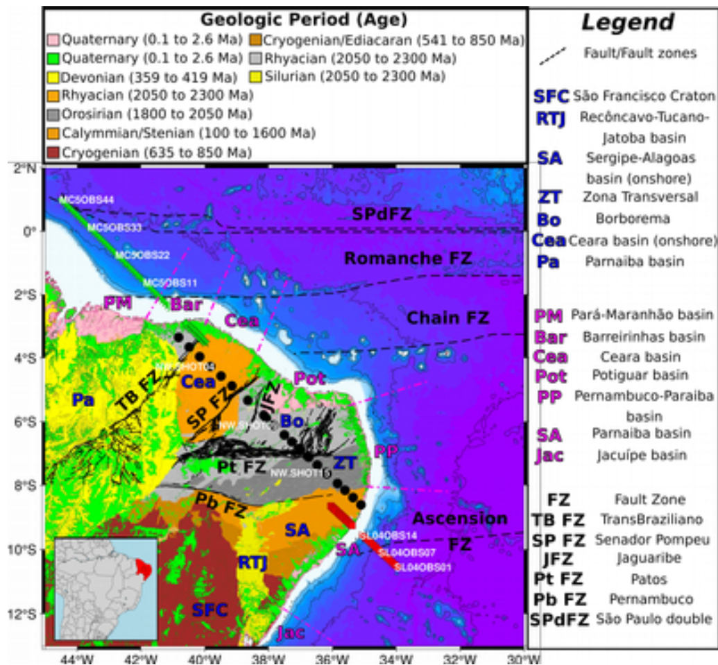
Figure 6.1 – Geology of the research area and studied profiles. (Green stars – MC5 profile from the MAGIC experiment; Black dots – NW profile of the INCT-ET project; red squares – SL04 profile from the SALSA experiment)
