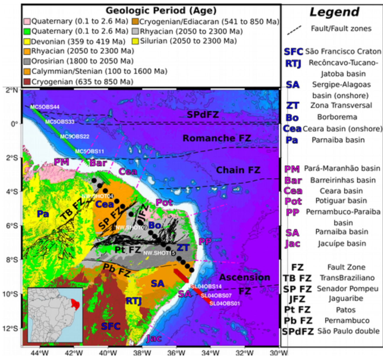
Figure 2.3.1 - Geology of the research area and studied profiles. (Green stars – MC5 profile from the MAGIC experiment; Black dots – NW profile of the INCT-ET project; red squares – SL04 profile from the SALSA experiment)
