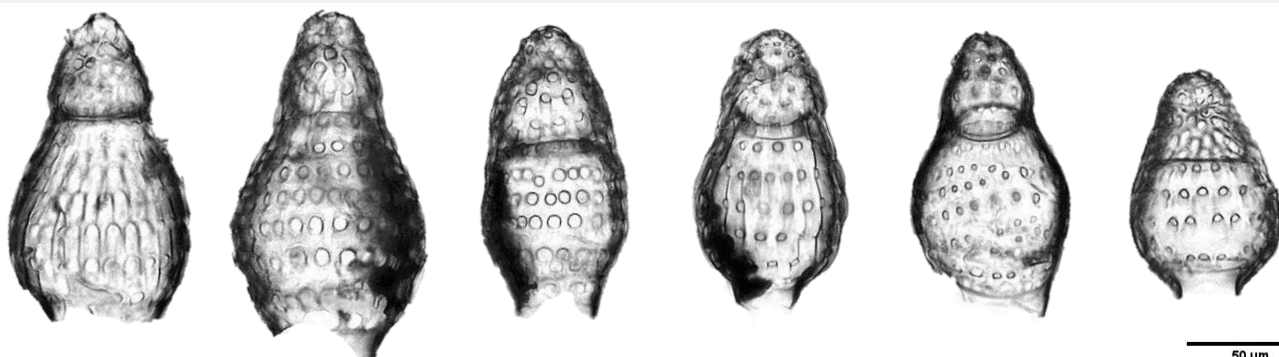
Dictyoprora spp.
