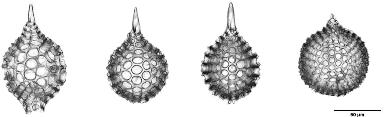
Zealithapium spp.
