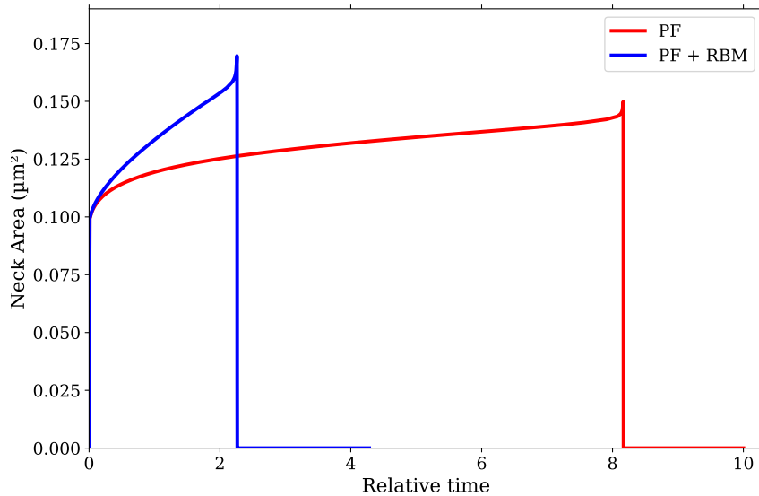
Figure 4.10: The evolution of neck growth over time for PF and PF+RBM model.
