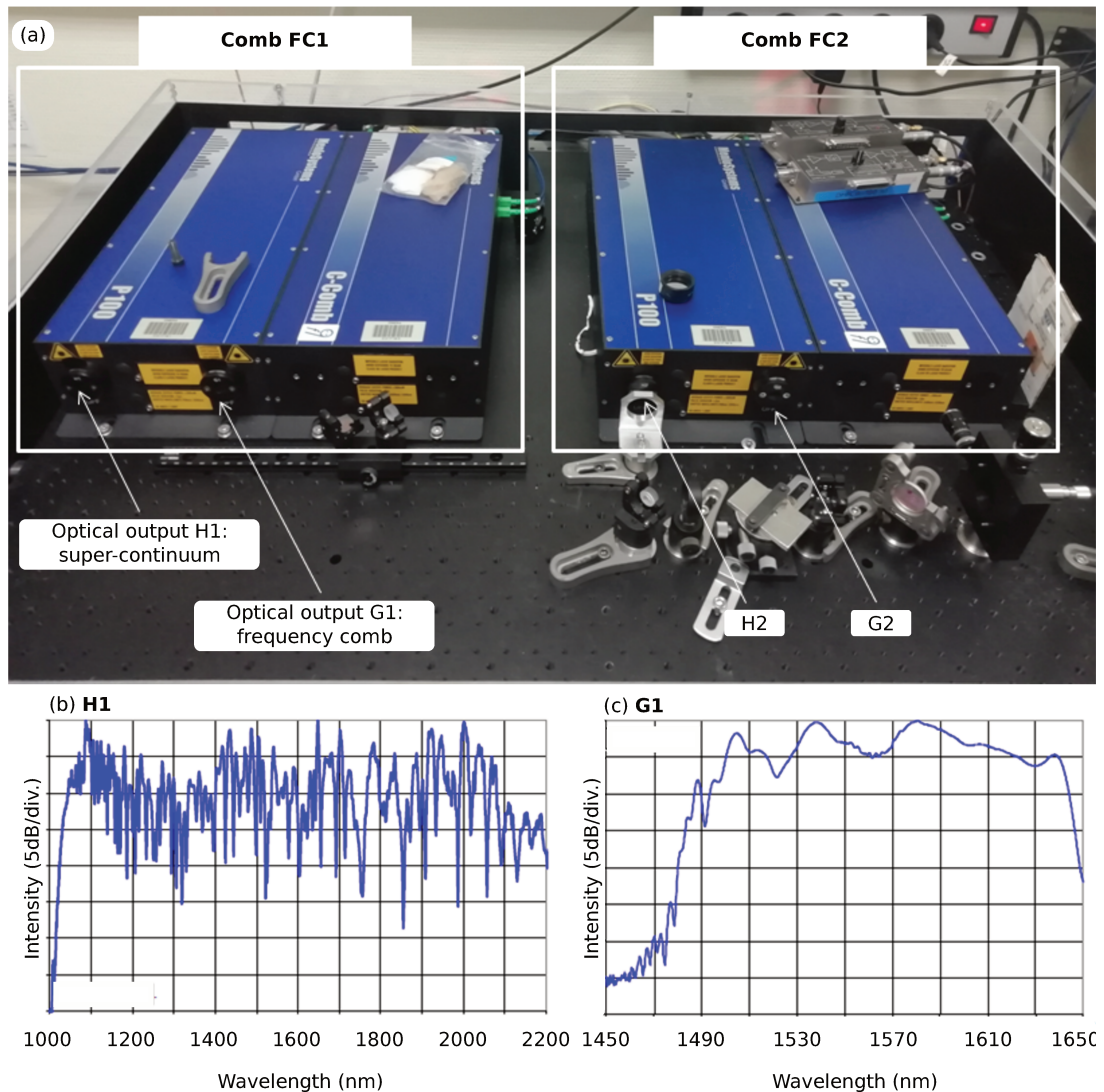
Figure A.1: Optical part of the setup.(a) Photograph of the optical table consisting of two commercial comb sources from MenloSystems, each with two free-space optical outputs: a frequency comb output G and an output H resulting from the spectral broadening of signal G, called "supercontinuum". (b) Optical spectra of the supercontinuum, H1, and of (c) the frequency comb, G1. Outputs for laser 1, from MenloSystems Technical Report, 2014.
