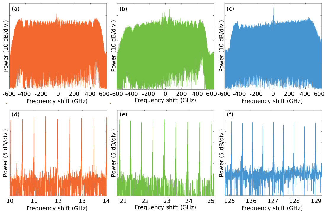
Figure 2.6: Example of broad spectrum at the output of the tri-core fiber for (a) Channel 1, (b) Channel 2 (c) and Channel 3. The high resolution (20 MHz) enables to show the teeth structure for each comb ((d) - (f)).
