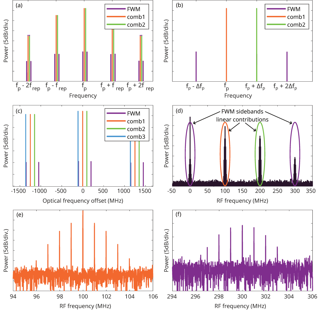
Figure 1.19: Numerical simulations of tri-comb interferometry for FWM spectroscopy. (a) Optical spectra of comb1 (orange) and comb2 (green) at f_{\text{rep}} that generate FWM sidebands (purple). The fiber has a length of L = 50 m, a dispersion parameter \beta_2 = 1 ps 2 /km, and a non-linear coefficient \gamma = 1 /W/km. (b) Zoom on the central spectral packets that shows the frequency shift of \Delta f_p between each line. (c) Optical spectrum of the FWM of comb1 and comb2, coupled with comb3 (blue), at f_{\text{rep}} + \Delta f_{\text{rep}} , used as local oscillator. (d) Associated electrical spectrum. The multi-heterodyne beating down converts the optical spectrum in the RF domain. Each contribution is isolated in a spectral packet centered at its difference of carrier frequency with the LO. (e) RF linear contribution of comb1 beating with comb3, centered at 100 MHz. (f) RF non-linear contribution of blue-shifted FWM sideband beating with comb3, centered at 300 MHz.
