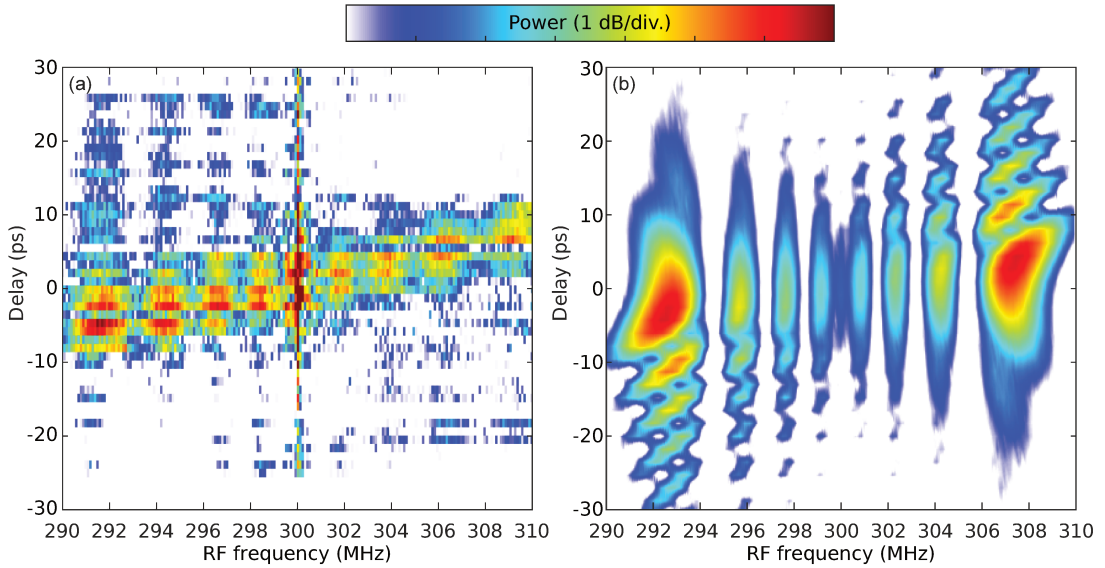
Figure 4.11: Envelopes of the spectrogram of the FWM component centred at 300 MHz. (a) Experimental results. (b) Numerical simulations.
