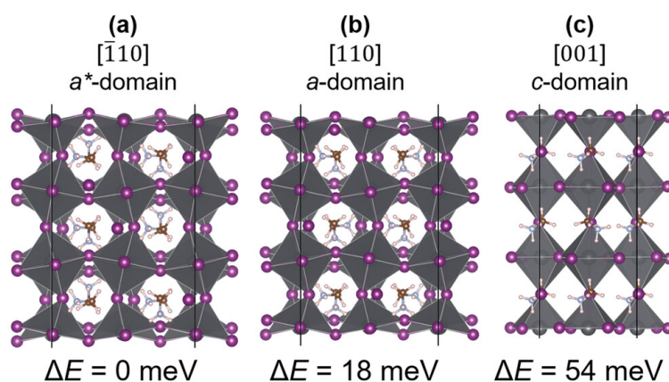
Figure 3.6: The three PbI 2 terminated surface configurations of tetragonal MAPbI 3 corresponding to a) [\bar{1}10] b) [110] and c) [001] orientations. The total energy is normalized by the number of MA molecules for comparison. The image is taken from [14].
