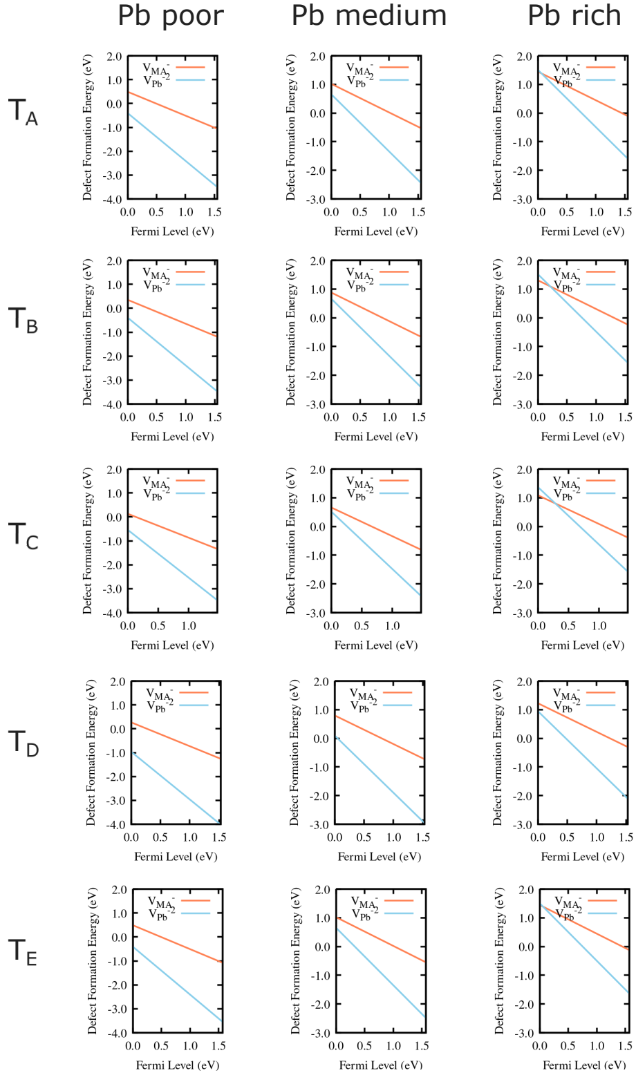
Figure 4.2: Plots illustrating the relationship between defect formation energy and Fermi level for the various tetragonal polymorphs [1]. The analysis covers three distinct scenarios, namely Pb-poor, Pb-medium, and Pb-rich conditions.
