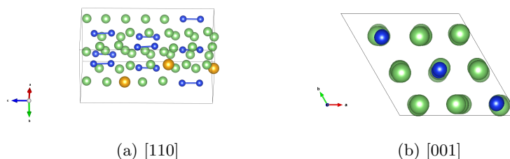
Figure 2.3: The unit cell ((a) [110] direction, (b) [001] direction) of the generally used and most stable \text{Li}_7\text{Si}_3 consisting of 9 columns containing 1 Si dumbbell each. Yellow spheres here are used to represent the vacancy sites that Li can potentially fill -they are the 3 rd Li site in 3 nearest neighbor columns. If 1, 2, or 3 sites are filled, we have the \text{Li}_{43}\text{Si}_{18} , \text{Li}_{44}\text{Si}_{18} , or the \text{Li}_5\text{Si}_2 phases, respectively.
