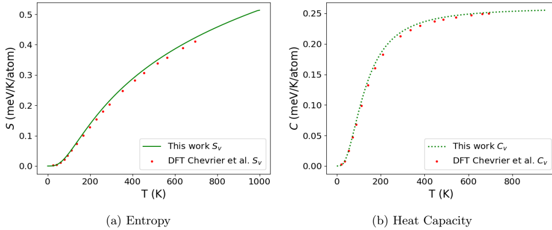
Figure 4.29: Plot of the \text{Li}_{15}\text{Si}_4 isochoric entropy (a) and heat capacity (b) vs temperature. Comparison with DFT HA by Chevrier et al [41].
