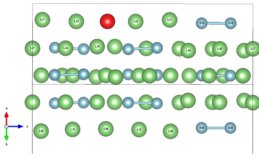
Figure 3.8: \text{Li}_7\text{Si}_3 unit cell labeled according to the symmetric CIF file found in Materials Project website [103] or in the appendix C. The red sphere represents the interstitial site for Li8 and its coordinates are a=0.22 , b=0.77 and c=0.66 (in fractional).
