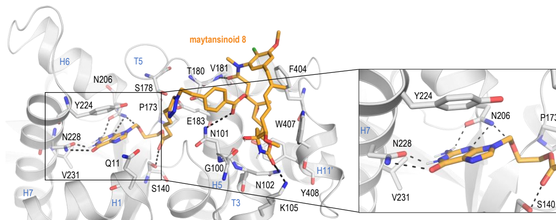
Figure IV-13. Docking results of maytansinoid-Acyclovir conjugates 7 (cyan) and 8 (orange). The \beta -tubulin is represented in light gray ribbon. The interacting residues and ligands are represented as sticks. Oxygen atoms are colored red, nitrogen atoms in navy blue, and chlorine atoms in green. Hydrogen bonds are displayed as black dashed lines.
