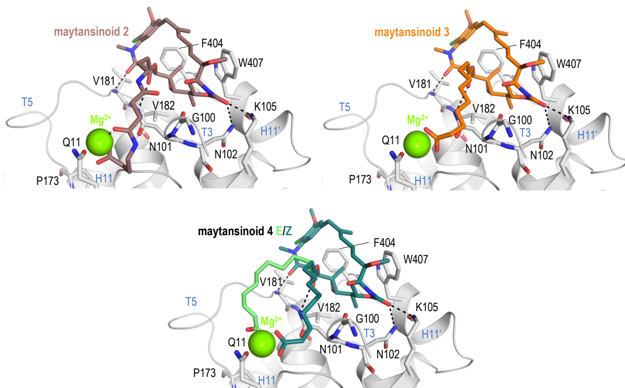
Figure IV-8. Docking results of the long-chain maytansinoids 2 , 3 and 4 when bound to \beta -tubulin in the presence of the Mg^{2+} (green sphere). The \beta -tubulin is represented in light gray ribbon. The interacting residues and ligands are represented as sticks. Oxygen atoms are colored red, nitrogen atoms in navy blue, and chlorine atoms in green. Hydrogen bonds are displayed as black dashed lines.
