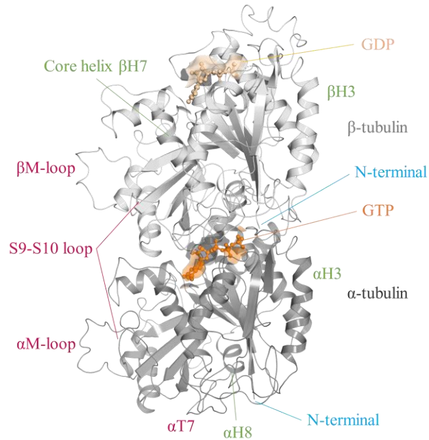
Figure I-1. 3D structure with PDB ID 1TUB of the first experimentally solved \alpha,\beta -tubulin heterodimer in complex with nucleotides GTP (dark orange) and GDP (light orange) in the \alpha (dark gray) and \beta -tubulin (light gray) monomers, respectively. The labels of the marked loops are colored in dark pink, the ones of the helices in green and the ones of the N-terminal amino acids in blue.
