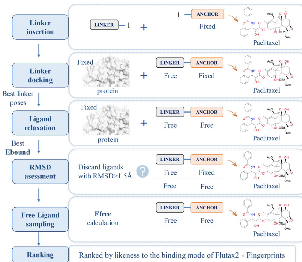
Figure V-6. Covalent docking protocol followed by S4MPLE.
