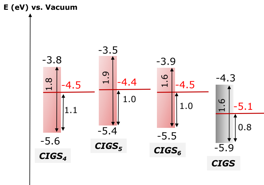
Figure 34: Schematic representation of the energy diagrams of CIGS_n lamellar compounds compared to CIGS chalcopyrite.
