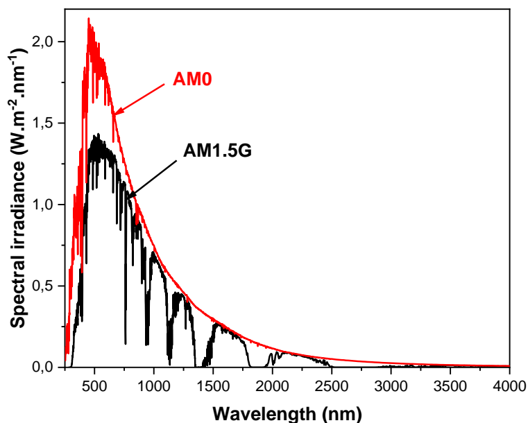
Figure 2: AM 1.5G solar spectrum compared to the AM0 spectrum outside the atmosphere. 5
