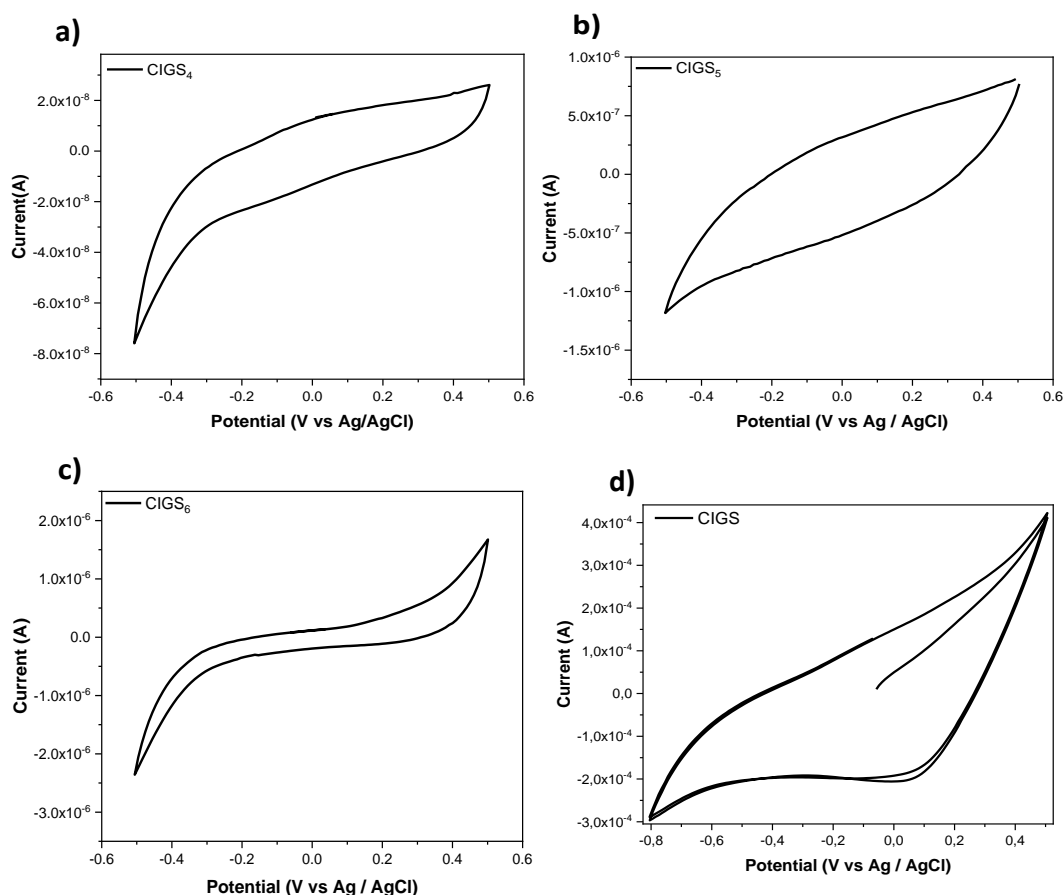
Figure 26: Cyclic voltammetry curves at a scan rate 5 mV/s for a) CIGS 4 , b) CIGS 5 , c) CIGS 6 and d) CIGS.
