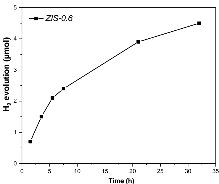
Figure 40: Photocatalytic H 2 evolution as a function of time of ZIS-0.6 using triethanolamine (pH=8) as sacrificial electron donor.
