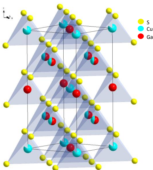
Figure 8: \text{CuGa}_3\text{S}_5 stannite structure-type.
