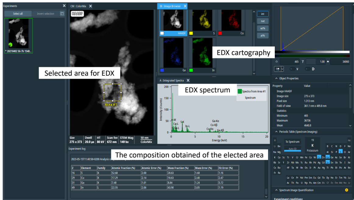
Figure 43: Main window of the Velox software used to analyse HAADF images and EDX analysis results.
