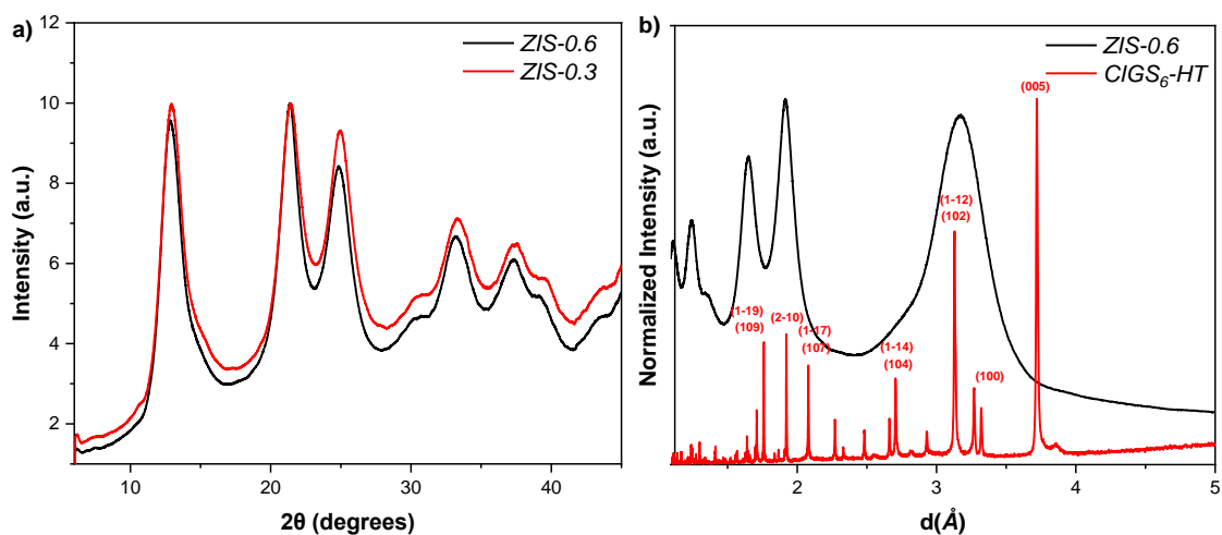
Figure 26: X-ray patterns of a) the prepared ZIS samples and b) the ZIS-0.6 sample compared to CIGS 6 -HT.
