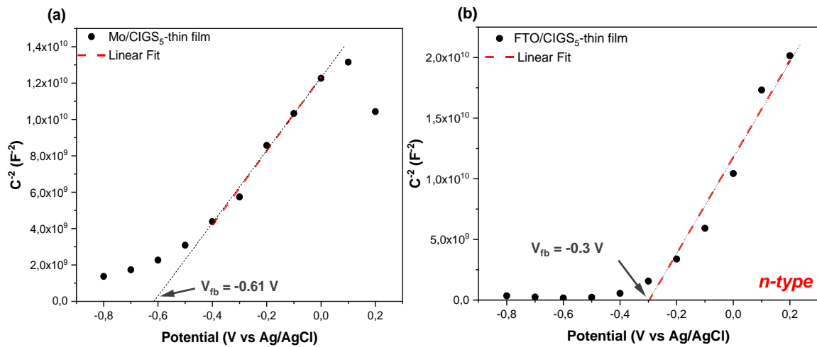
Figure 24: Mott Schottky plots of a) SLG/Mo/CIGS 5 and b) SLG/FTO/CIGS 5 thin films with the estimated flat band potentials from the linear fit of the slopes.
