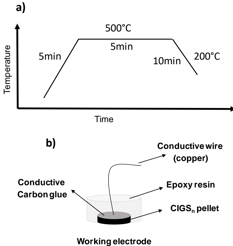
Figure 40: Preparation of the working electrode: a) Temperature protocol of CIGS n sintering using spark plasma sintering SPS. b) Schematic representation of prepared working electrode.
