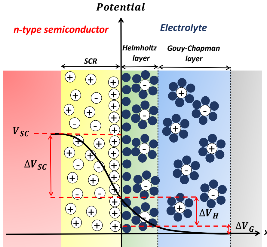
Figure 11: Schematic representation of an n-type semiconductor electrolyte interface with different layers involved: space charge region SCR layer (semiconductor side), Helmholtz layer and Guy Chapman layer (electrolyte side), showing the gradient potential difference between the layers.
