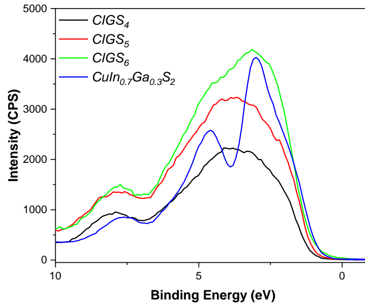
Figure 33: XPS valence band spectra of CIGS 4 , CIGS 5 , CIGS 6 and CuIn 0.7 Ga 0.3 S 2 (CIGS) compounds in the range 10 to 0 eV. 1
