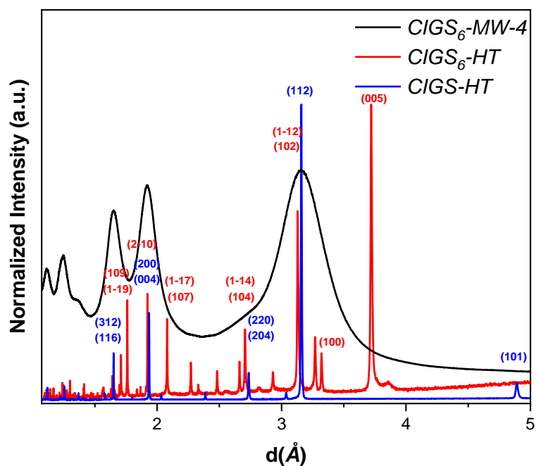
Figure 21: X-ray diffraction patterns of CIGS 6 -MW-4 compared to the high temperature standards (CIGS 6 and CIGS chalcopyrite).
