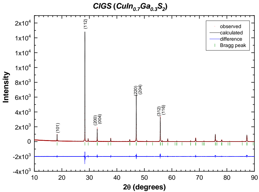
Figure 5: XRD pattern and Le Bail refinement of the CIGS (CuIn 0.7 Ga 0.3 S 2 ) compound.
