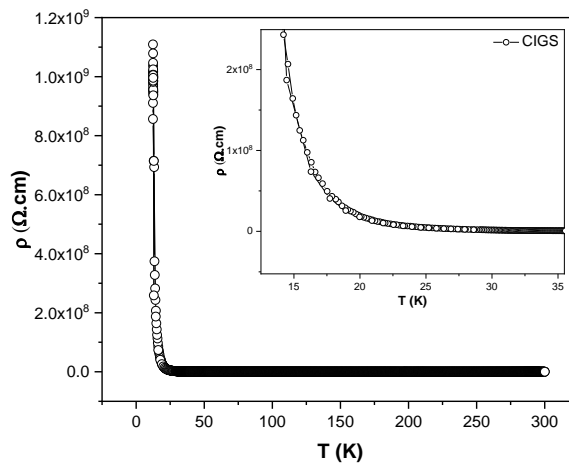
Figure 30: Variation of the resistivity in function of the temperature of the CIGS sample.
