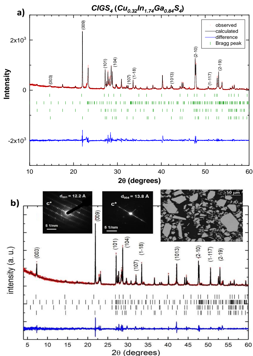
Figure 2: XRD pattern and Le Bail refinement of the \text{CIGS}_4 (\text{Cu}_{0.32}\text{In}_{1.74}\text{Ga}_{0.84}\text{S}_4) compound a) prepared during the thesis b) with electron image and electron diffraction patterns presented in the backscattered. Figure from reference Caldes et al 1
