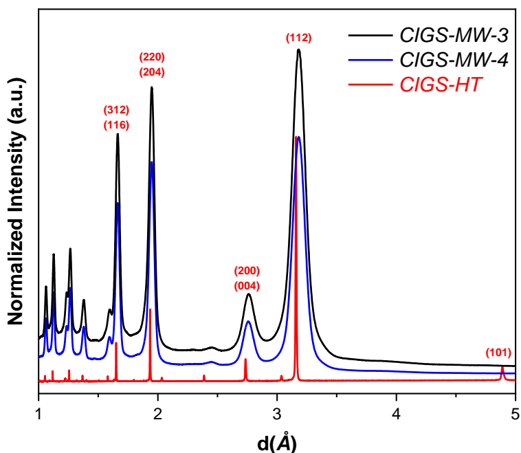
Figure 13: X-ray diffraction patterns of CIGS-MW-3 and CIGS-MW-4 compounds compared to that of CIGS-HT.
