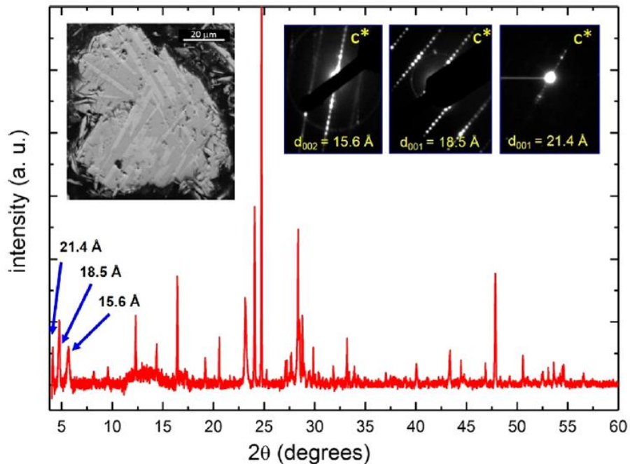
Figure 10: XRD pattern of Cu 0.4 (In 0.5 Ga 0.5 ) 1.2 S 2 multiphasic compound. The corresponding electronic diffraction patterns and SEM electron image are inserted in the top of the figure. Figure from Caldes et al. 61
