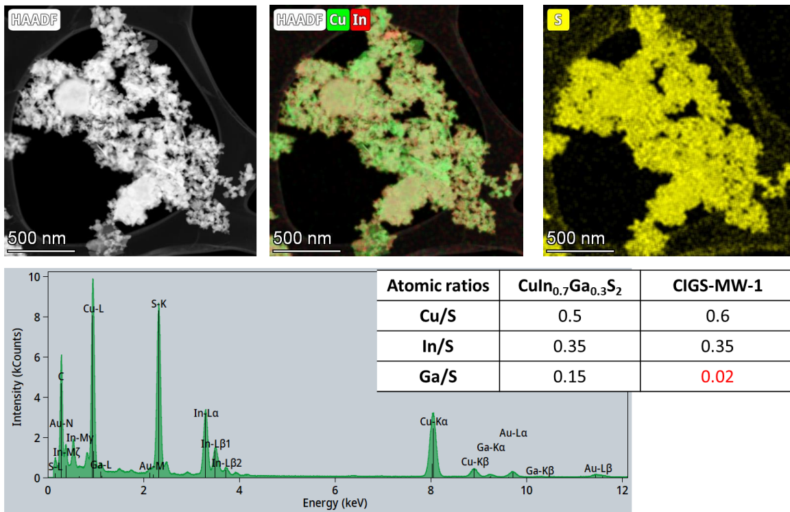
Figure 10: HAADF image and EDX mapping of CIGS-MW-1 nanograins revealing an inhomogeneous sample. The inserted table compares atomic ratios of experimental average composition of the nanograins agglomerates, with theoretical ones of the chalcopyrite \text{CuIn}_{0.7}\text{Ga}_{0.3}\text{S}_2 . A significant gallium deficit is highlighted.
