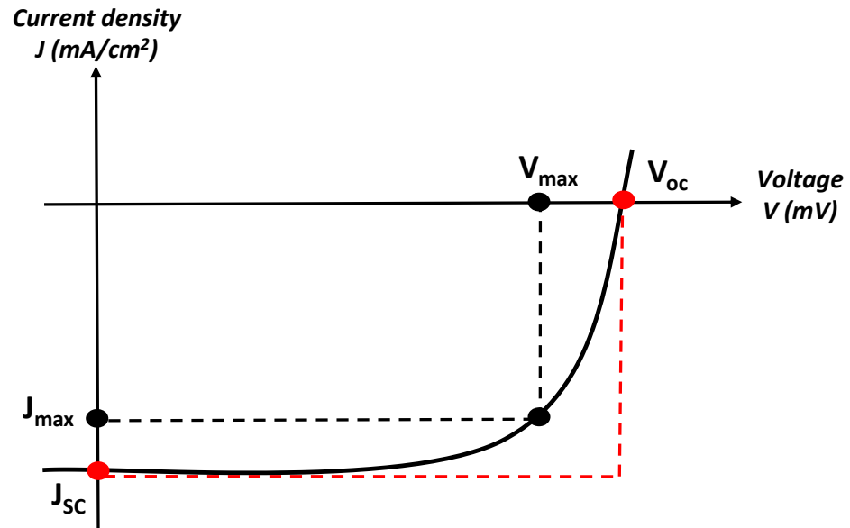
Figure 45: Characteristic JV (current density versus voltage) curve of a solar cell under illumination.
