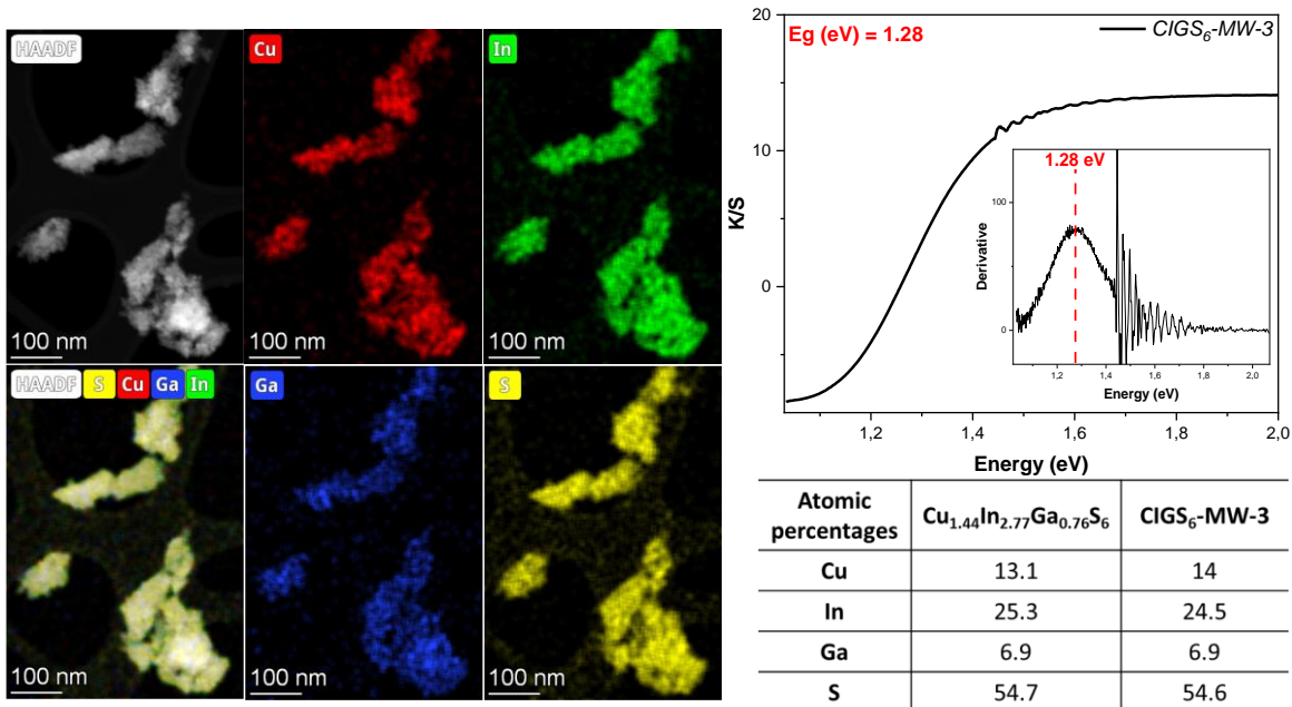
Figure 17: EDX mapping of sample \text{CIGS}_6\text{-MW-3} , showing a homogeneous composition of the nanograins agglomerates close to the target composition \text{Cu}_{1.44}\text{In}_{2.77}\text{Ga}_{0.76}\text{S}_6 (see inserted table). In the top right, Kubelka-Munk transformed reflectance spectra of \text{CIGS}_6\text{-MW-3} compound.
