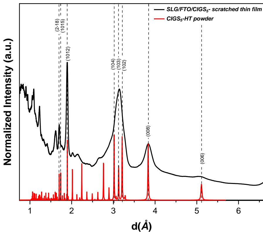
Figure 13: X-ray diffraction patterns of the powder from scratched CIGS 5 thin films on FTO covered soda lime glass compared to the reference powder of the same target composition Cu_{0.63}In_{1.9}Ga_{1.26}S_5 .
