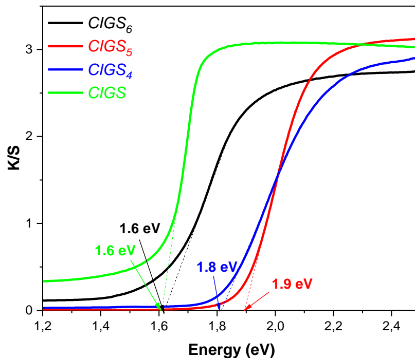
Figure 6: Kubelka-Munk transformed reflectance spectra of the CIGS chalcopyrite and the lamellar compounds: CIGS_4 , CIGS_5 and CIGS_6 .
