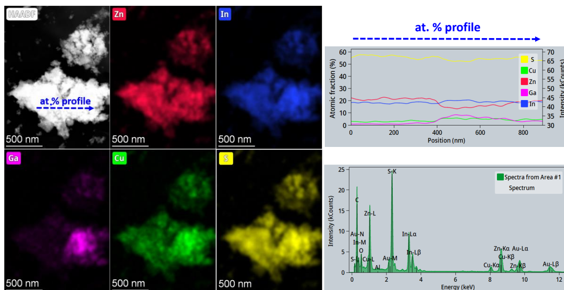
Figure 24: EDX mapping and atomic fraction profile of ZIS-0.6, showing the inhomogeneity of the sample. In the bottom right, the EDX spectrum of ZIS-0.6 compound.
