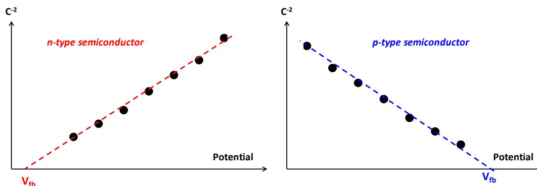
Figure 18: Mott-Schottky plots depending on the applied potential for n-type (negative slope) and p-type (positive slope) semiconductors.
