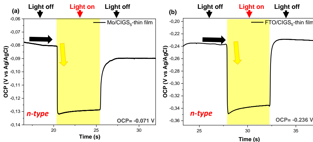
Figure 26: Chronopotentiometry curves under illumination (indicated by the yellow region) and under dark of thin films: a) SLG/Mo/CIGS 5 . b) SLG/FTO/CIGS 5 .
