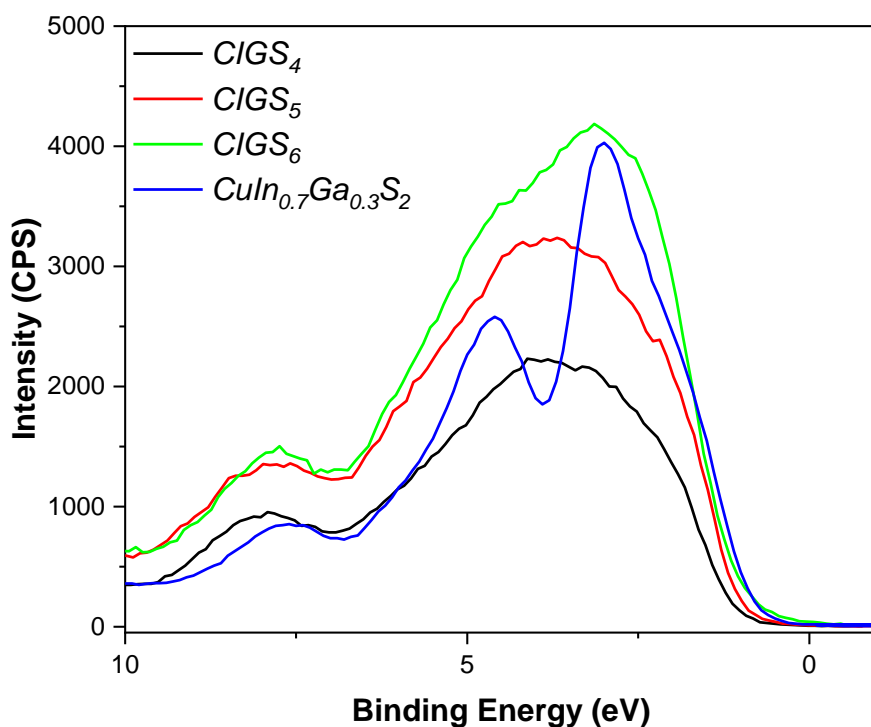
Figure 13: XPS valence band spectra of CIGS n lamellar compounds and CIGS (CuIn 0.7 Ga 0.3 S 2 ) chalcopyrite. 61
