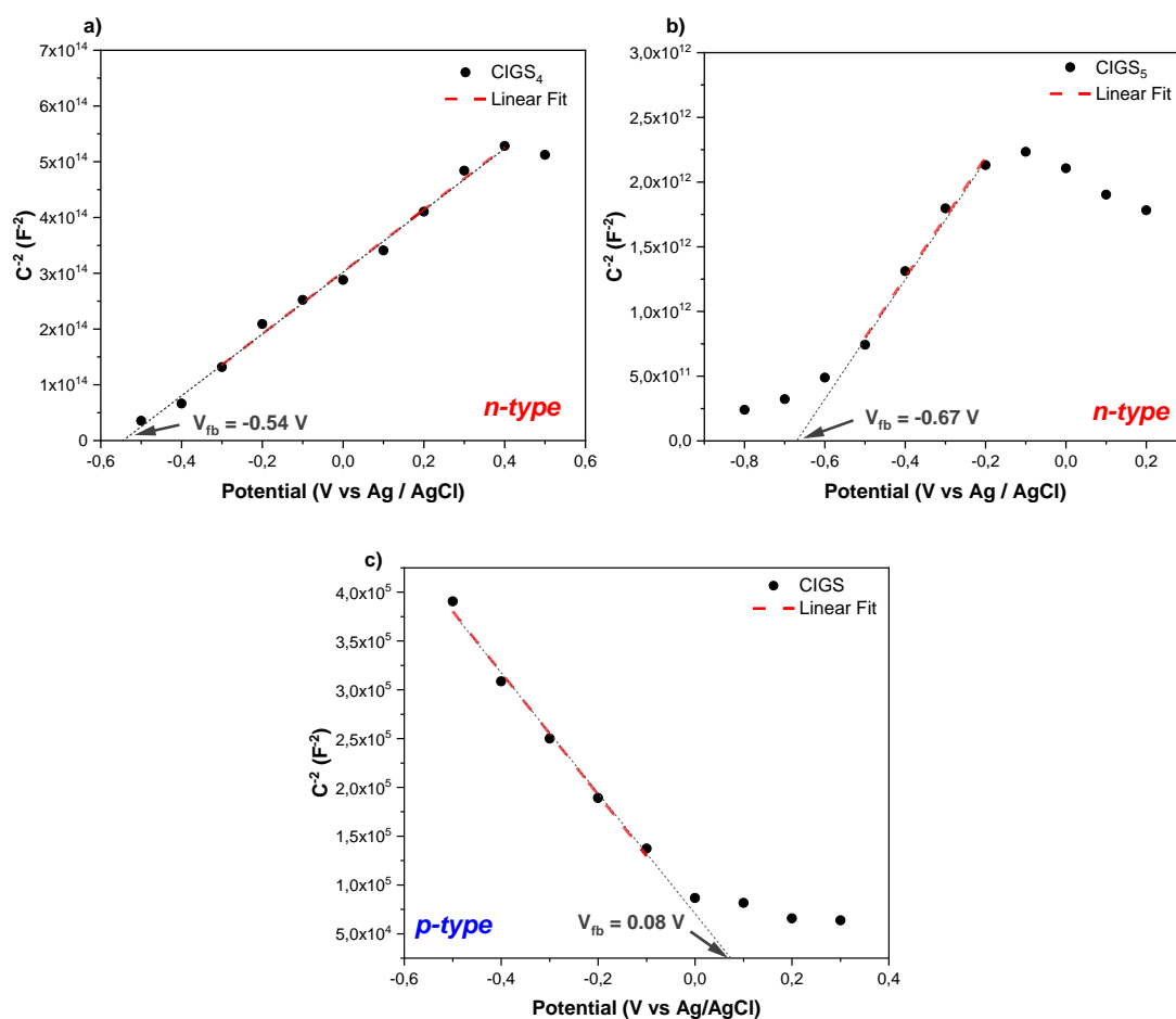
Figure 28: Mott-Schottky C^2 - E (V vs Ag/AgCl) plots modelled at high frequencies (1– 10 kHz), with linear fit of the slopes to determine the flat band potentials for: a) CIGS 4 , b) CIGS 5 and c) CIGS.
