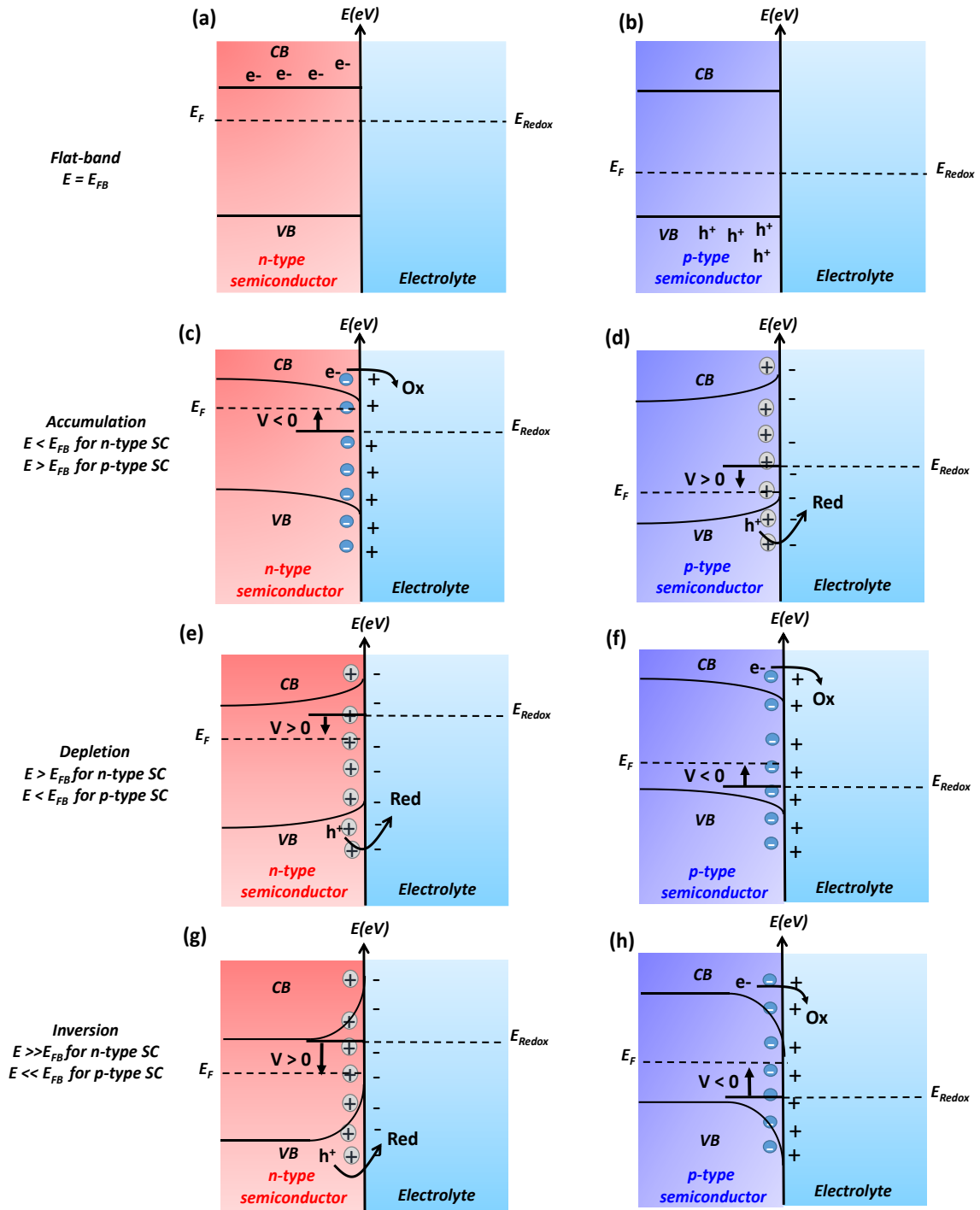
Figure 13: Schematic representation of bands bending for n-type and p-type semiconductors on contact with the electrolyte during applying a potential bias, presenting all possible situations.
