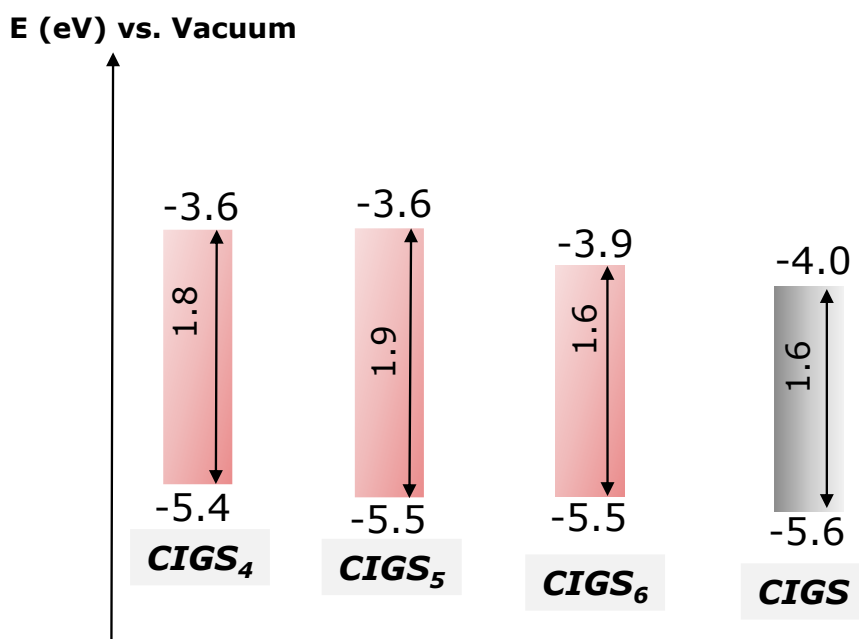
Figure 35: Schematic representation of the calculated energy levels of the conduction and valence band of the CIGS_n lamellar compounds compared to CIGS chalcopyrite.
