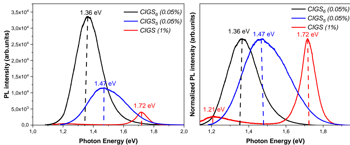
Figure 37: Photoluminescence spectra at 488 nm of CIGS 6 and CIGS 5 lamellar compounds compared to the CIGS chalcopyrite.
