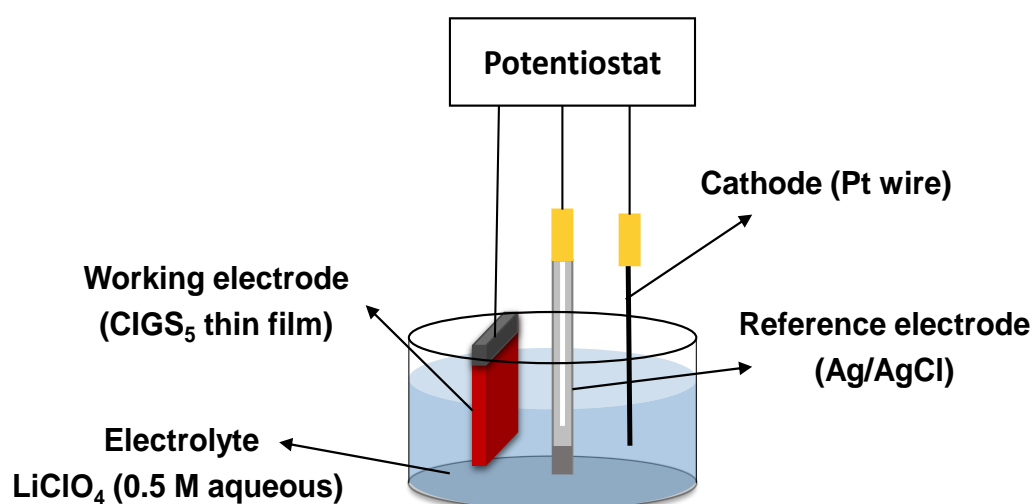
Figure 21: Schematic representation of the three electrodes cells used during the electrochemical and photo-electrochemical measurements on \text{CIGS}_5 thin films.
