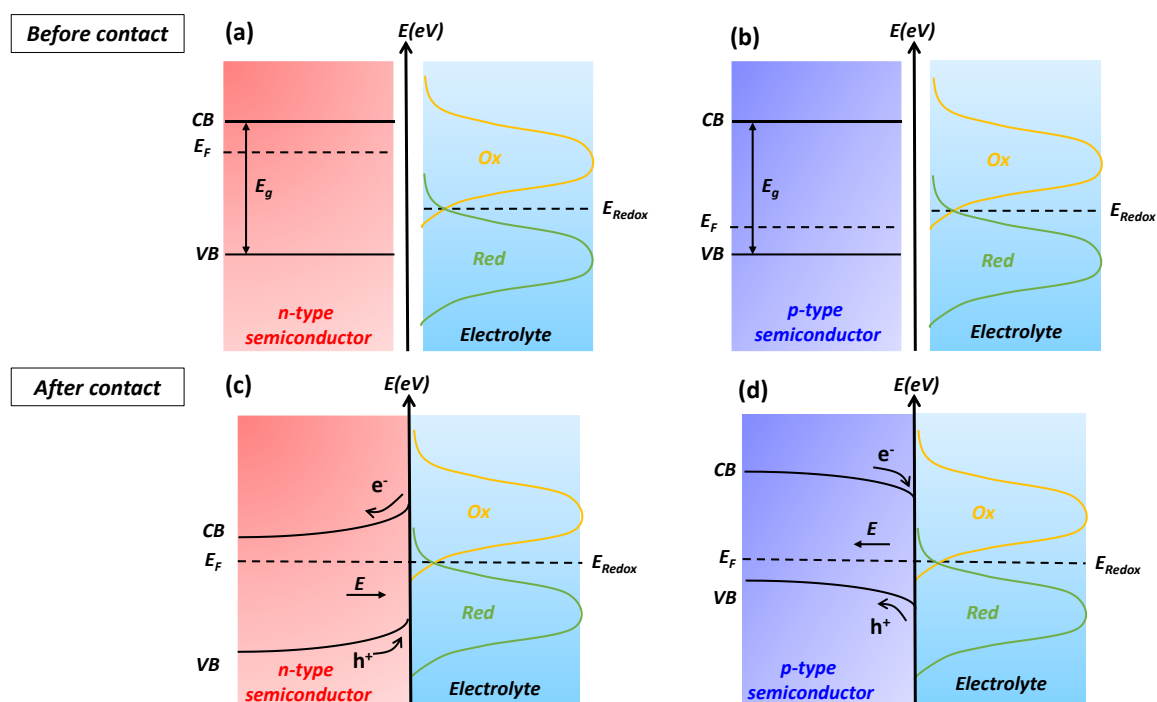
Figure 10: Schematic representation of Fermi levels alignment during the formation of a semiconductor/electrolyte interface.
