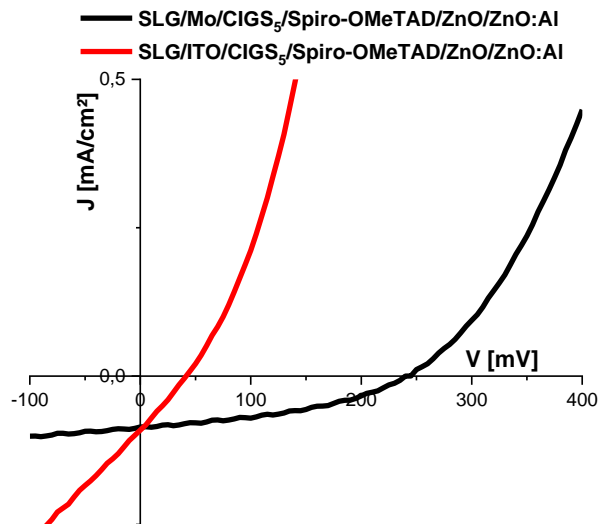
Figure 40: current voltage (JV) curves measured under illumination of the SLG/Mo/CIGS5/Spiro-OMeTAD/ZnO/ZnO:Al and SLG/ITO/CIGS5/Spiro-OMeTAD/ZnO/ZnO:Al.
