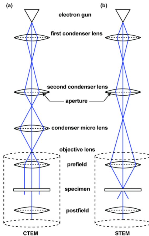
Figure 41: Simplified schematic of principle of (a) TEM and (b) the scanning mode STEM. 64
