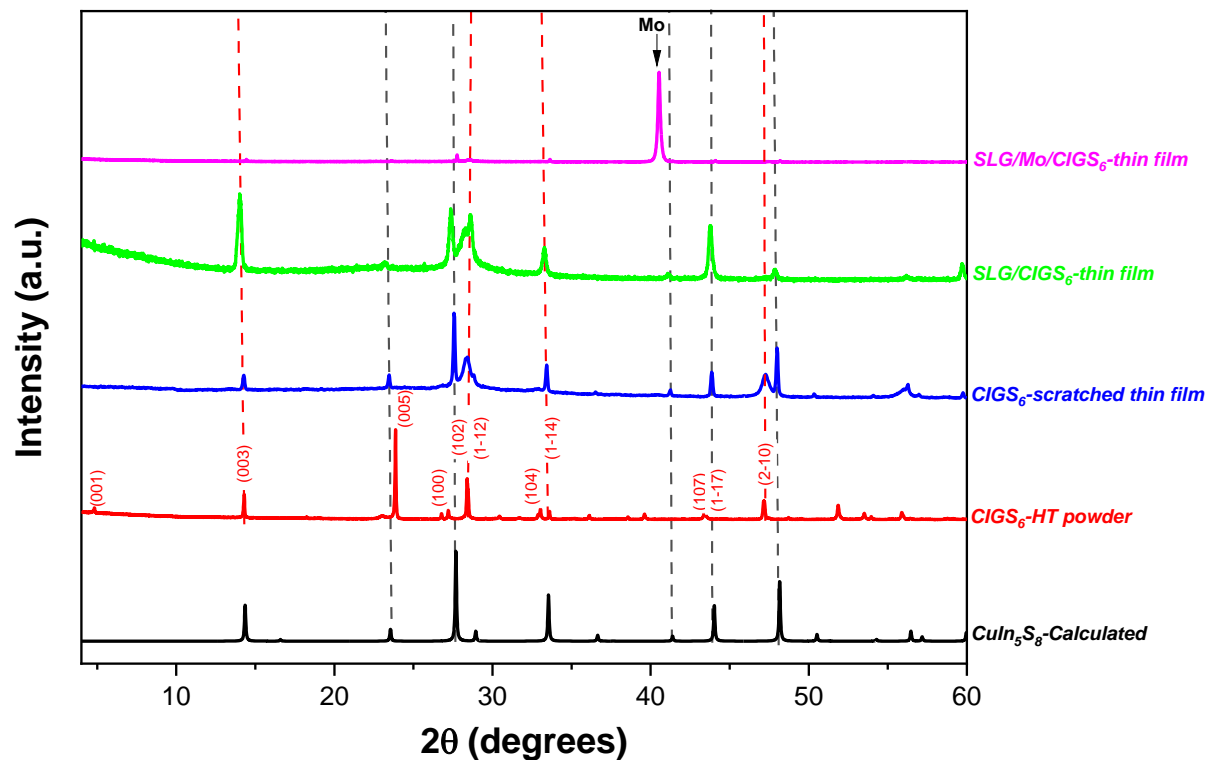
Figure 10: X-ray diffraction patterns of the deposited CIGS 6 thin films on glass and on Mo covered soda lime glass compared to the reference powder of the same target composition Cu 1,44 In 2,77 Ga 0,76 S 6 and the secondary phase observed CuIn 5 S 8 .
