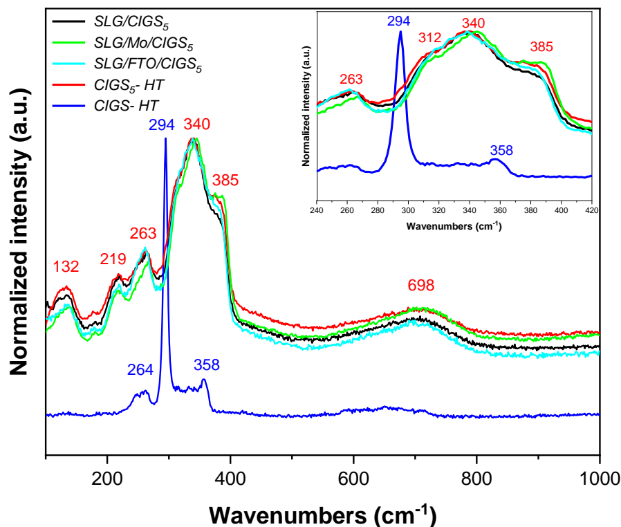
Figure 16: Raman spectra at excitation wavelength 514 nm of CIGS 5 thin films deposited on SLG, on SLG/Mo and SLG/FTO compared to the CIGS 5 reference powder and the CIGS chalcopyrite, with a zoom on the range (240 – 420 cm -1 ) on the top.
