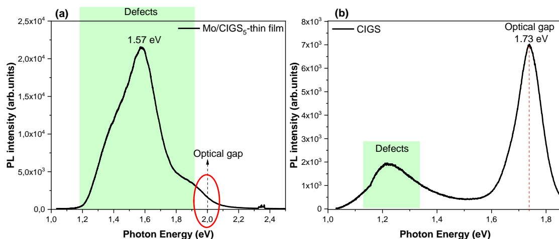
Figure 20: Photoluminescence spectra at 488 nm of (a) thin film of \text{CIGS}_5 lamellar compound (b) CIGS chalcopyrite.
