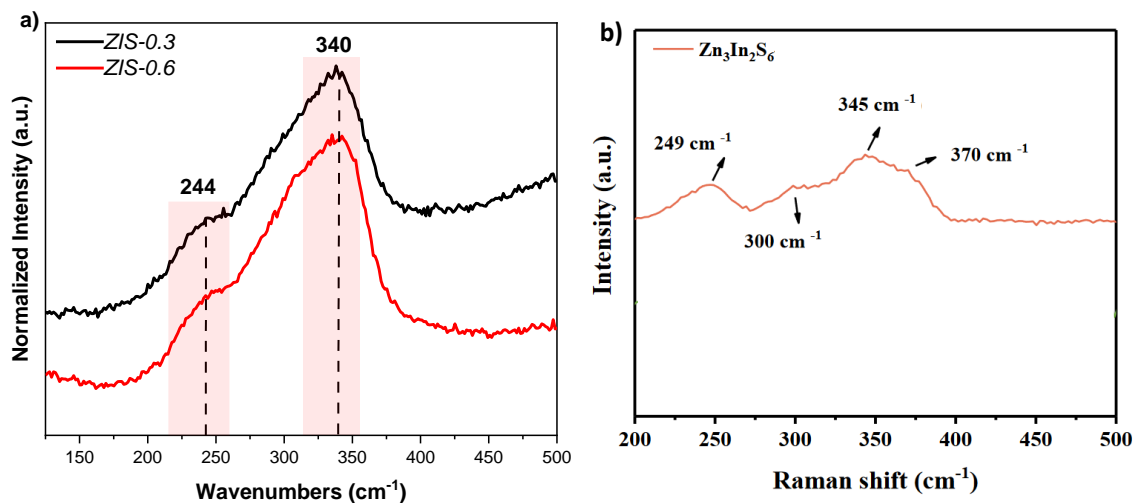
Figure 27: a) Raman spectra at 514 nm of ZIS-0.3 and ZIS-0.6 samples. b) Raman spectra of Zn 3 In 2 S 6 . Figure modified from the reference Luo et al. 60
