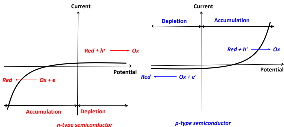
Figure 14: Current potential characteristics depending on the applied potential, presenting a saturated reduction current for p-type semiconductor and a saturated oxidation current for n-type semiconductor.
