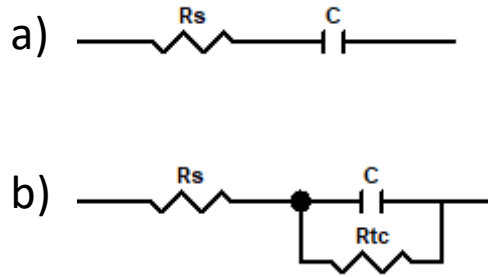
Figure 20: The Randles simplified circuits: a) RC circuit and b) the Randles circuit with a neglected Warburg.
