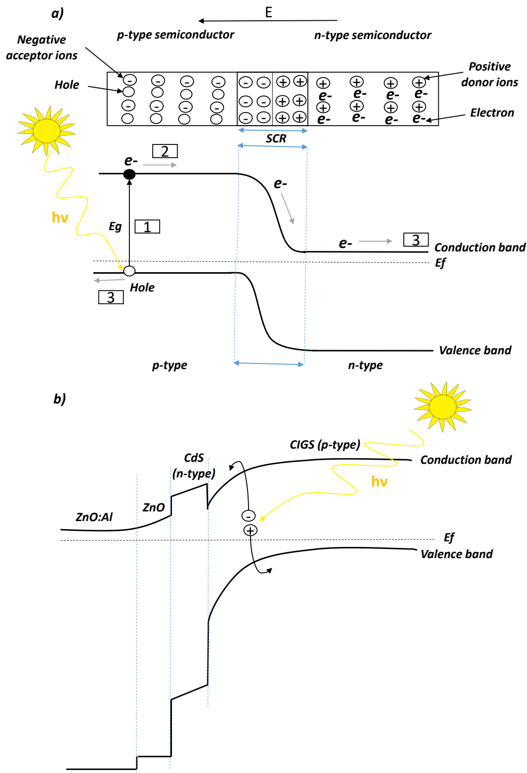
Figure 1: Schematic representation of a) the p-n junction and the mechanism of a silicon based solar cell presenting p-n homojunction. b) The band diagram of p-n heterojunction (CIGS solar cell).
