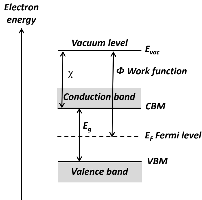
Figure 44: Schematic representation of the energy diagram of a semiconductor.
