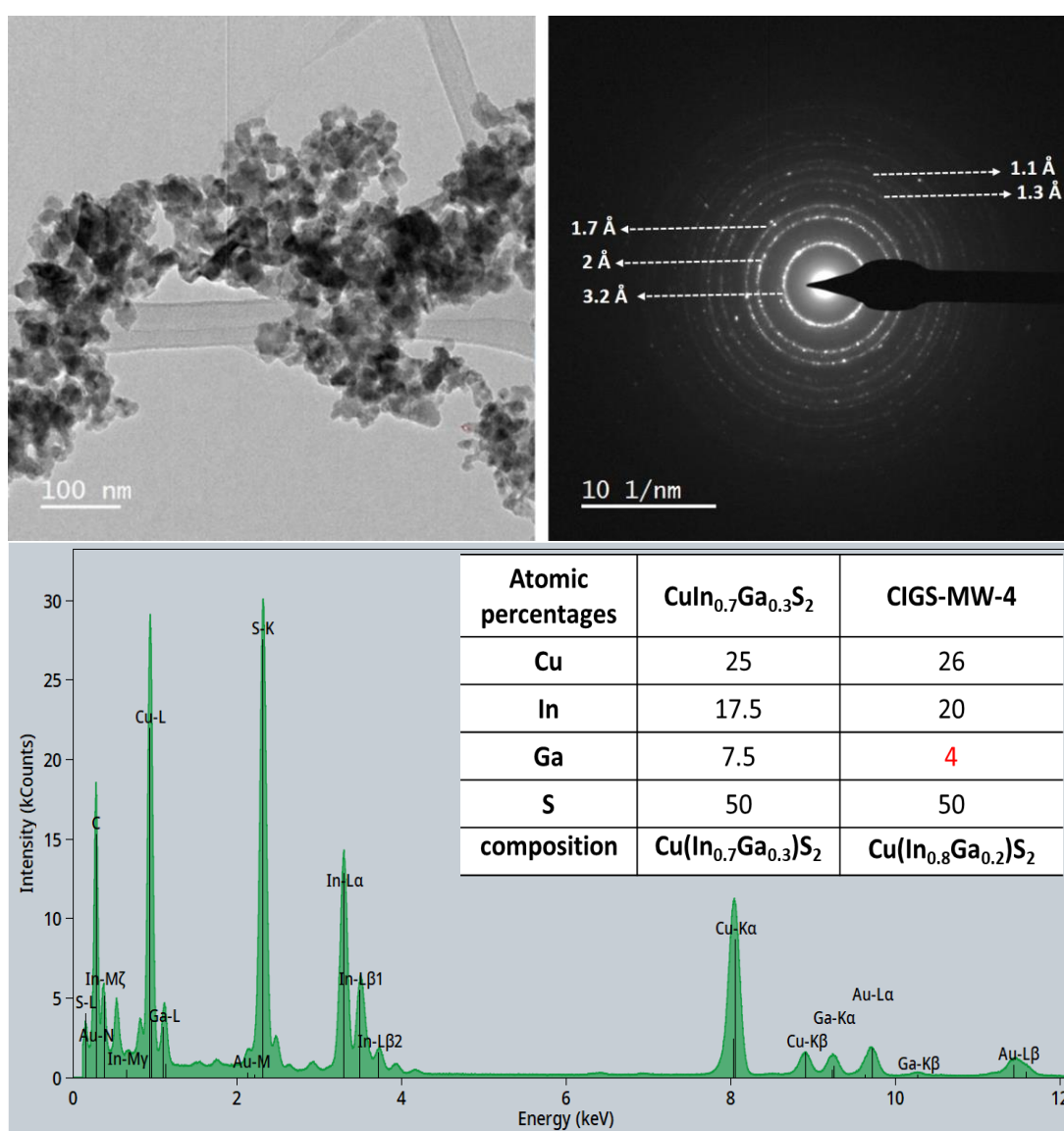
Figure 12: EDX spectrum of CIGS-MW-4 and TEM image showing agglomerates of nanocrystals. The inserted table presents CIGS-MW-4 atomic percentages obtained from EDX compared to theoretical ones.
