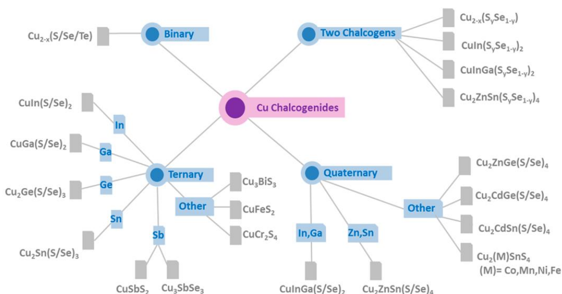
Figure 1: Schematic illustration of the different copper-based chalcogenide semiconductors available in the literature. Figure from Coughlan et al. 1
