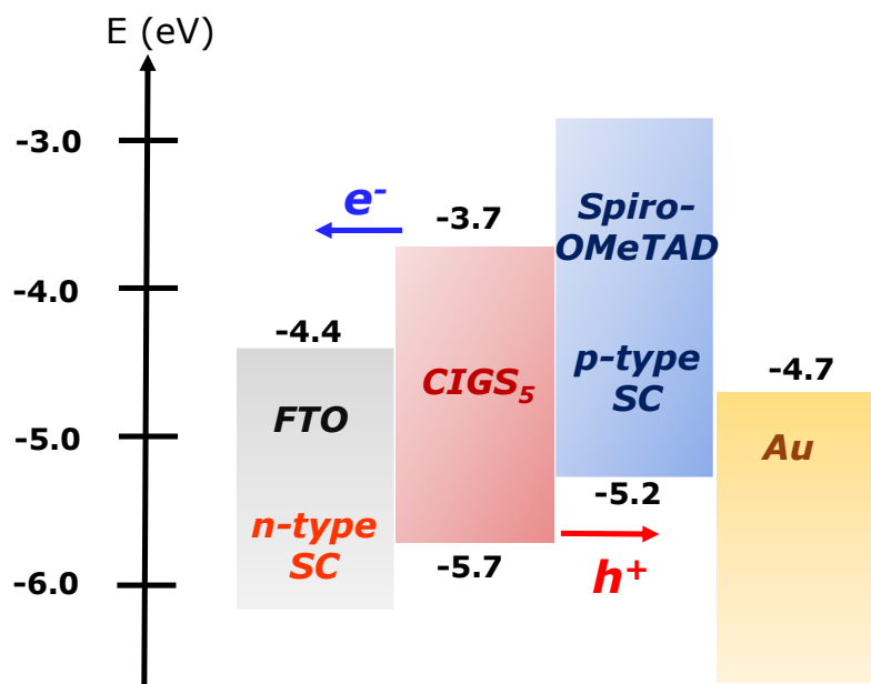
Figure 37: Energy diagrams of the prepared n-i-p architecture device at no contact.
