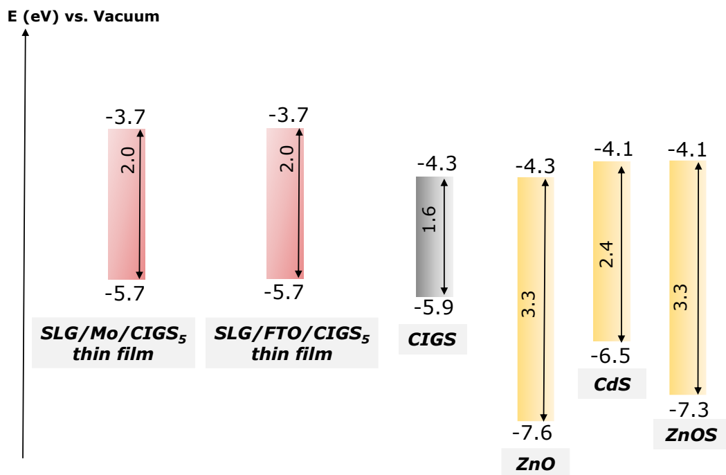
Figure 33: Schematic energy diagrams of CIGS 5 thin films and CIGS compound compared to those of main buffer layers used in CIGS-based solar cells.
