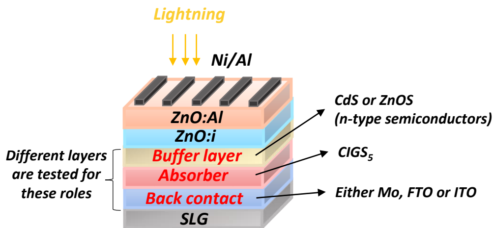
Figure 29: Schematic representation of the prepared device, with the different layers used.
