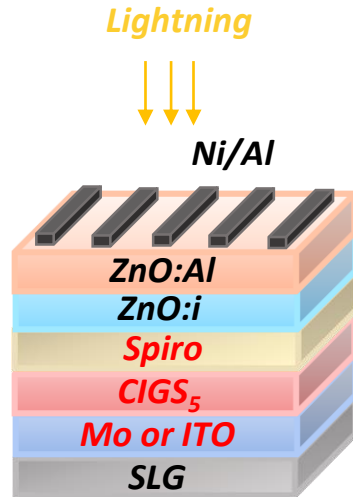
Figure 39: Schematic representation of the assembly prepared using spiro-OMeTAD as a buffer layer, with the different layers used.
