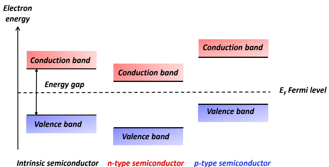
Figure 7: Fermi level positioning for different types of semiconductors (intrinsic, n-type and p-type semiconductors).
