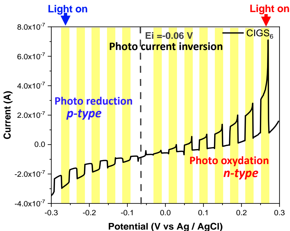
Figure 25: Current-potential curve measured under chopped illumination (yellow part) of CIGS 6 .
