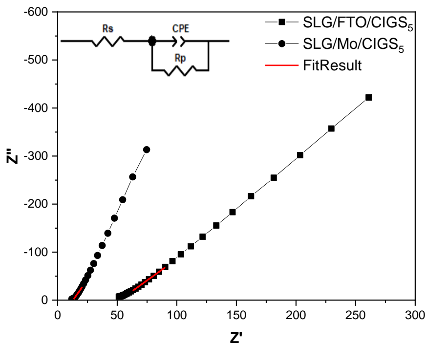
Figure 22: Nyquist curves at -0.3 V obtained from electrochemical impedance spectroscopy with the applied equivalent circuit for fitting at high frequencies (1-10 kHz) (red line) of CIGS 5 thin films deposited on SLG/Mo and on SLG/FTO.
