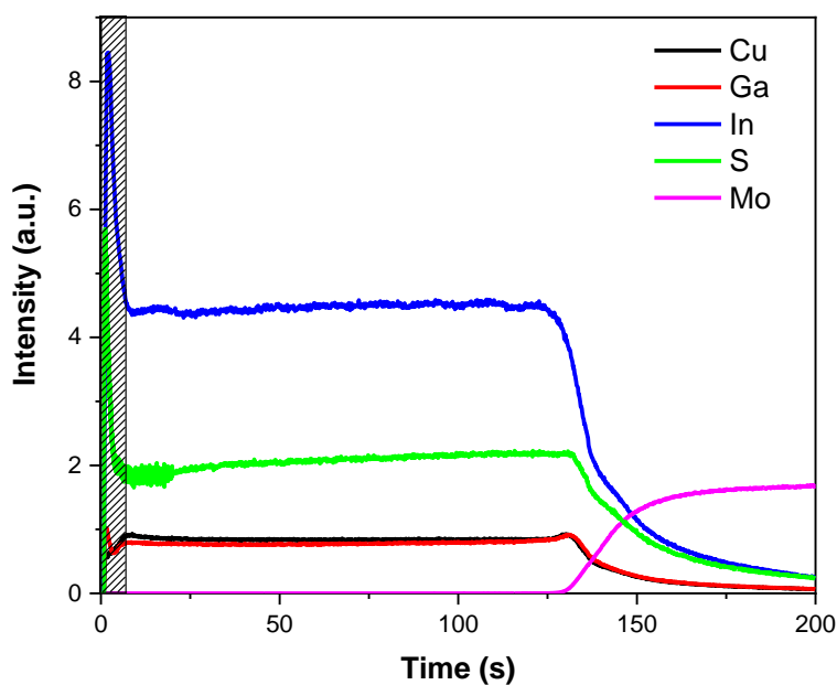
Figure 17: GDOES depth profile elementary analysis of CIGS 5 thin film deposited on Mo covered soda lime glass.
