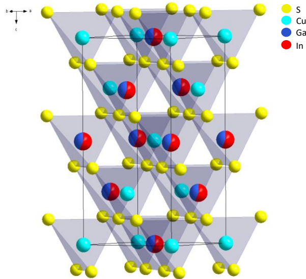
Figure 3: \text{CuIn}_{0.7}\text{Ga}_{0.3}\text{S}_2 chalcopyrite structure-type.
