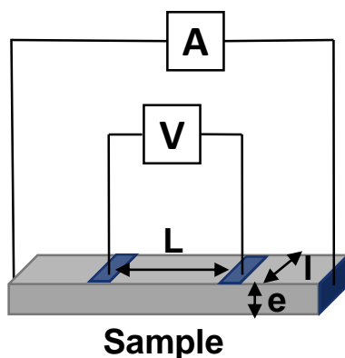
Figure 41: Schematic representation of four-point probe measurements.
