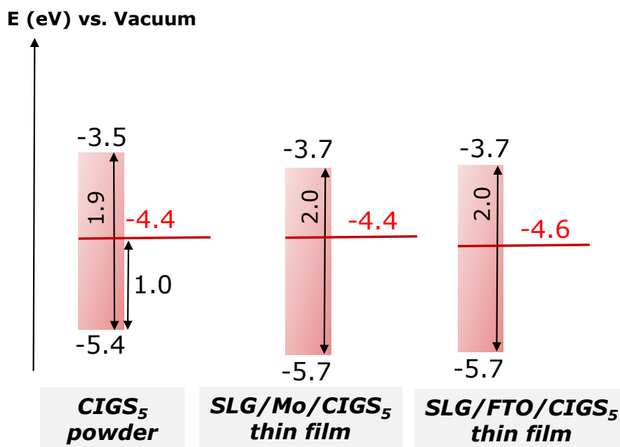
Figure 25: Schematic representation of the energy bands on absolute scale with respect of the vacuum of the CIGS 5 thin films compared to the reference CIGS 5 powder.
