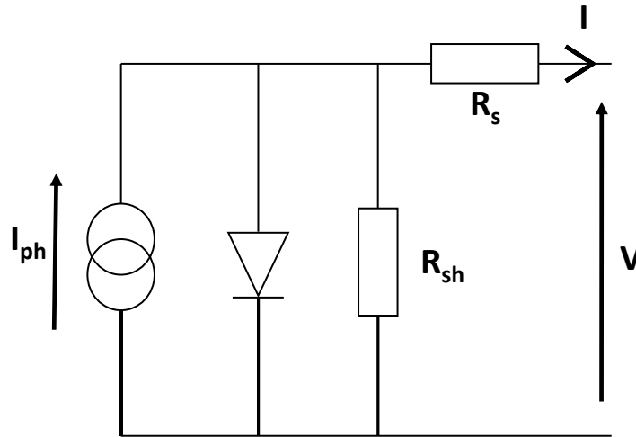
Figure 3: Equivalent electrical circuit of a photovoltaic cell with I_{ph} : the photogenerated current, R_s : series resistor and R_{sh} : parallel resistor.
