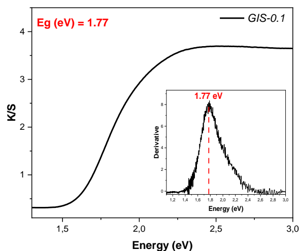
Figure 33: Kubelka-Munk transformed reflectance spectrum of GIS-0.1 copper poor sample.
