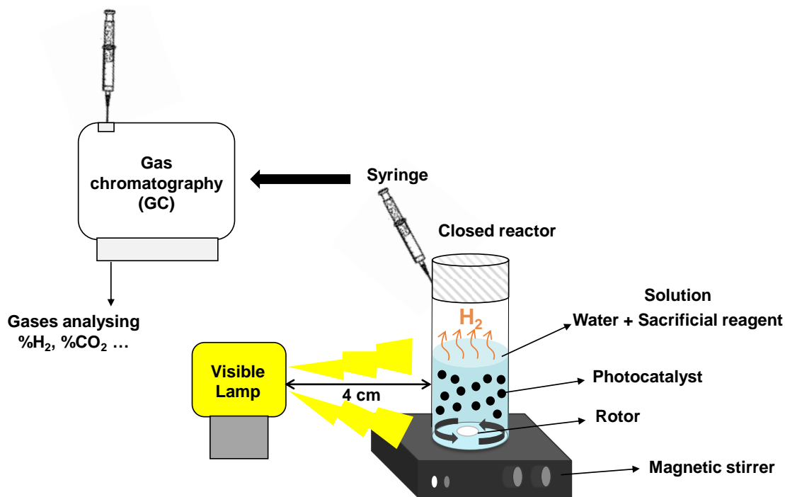
Figure 37: A schematic representation of the set-up used for photocatalytic hydrogen production.
