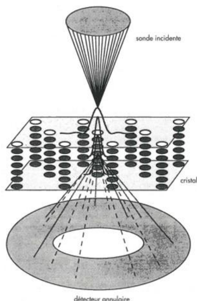
Figure 42: Principle of HAADF contrast formation. 65
