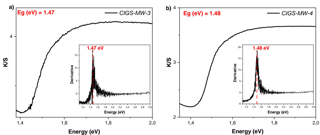
Figure 15: Kubelka-Munk transformed reflectance spectra of a) CIGS-MW-3 and b) CIGS-MW-4 compounds.
