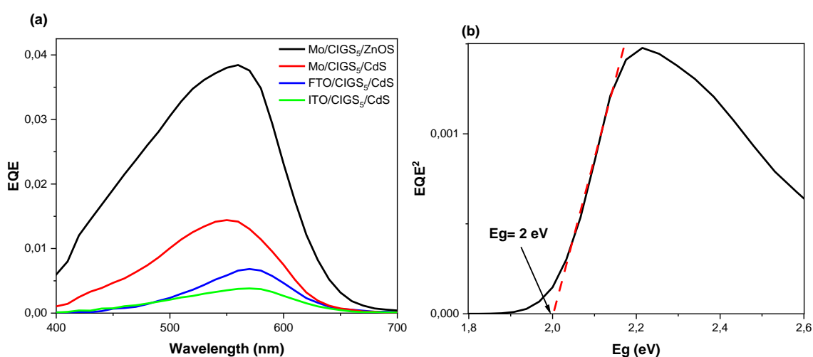
Figure 32: (a) External quantum efficiency (EQE) curves of the prepared devices. (b) Band gap determination from external quantum efficiency (EQE) curve of the CIGS 5 absorber.
