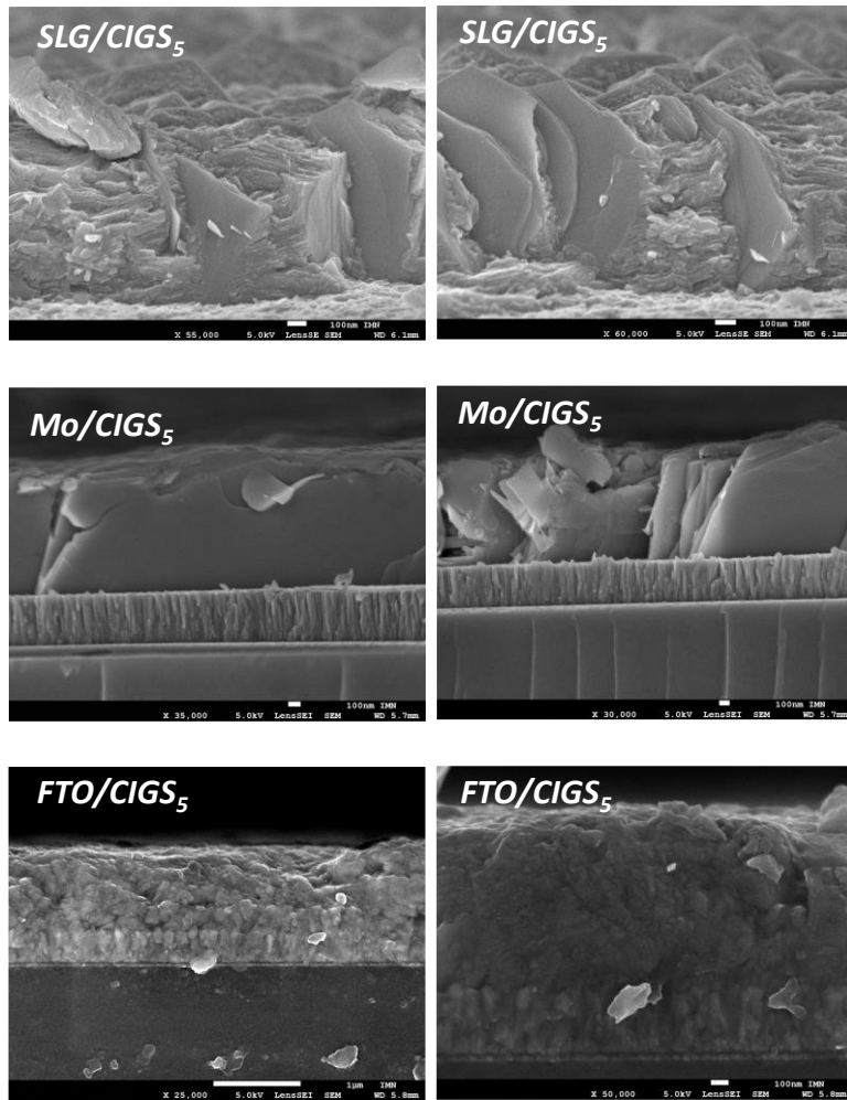
Figure 34: SEM images of cross sections for investigated CIGS 5 thin films with different substrates.
