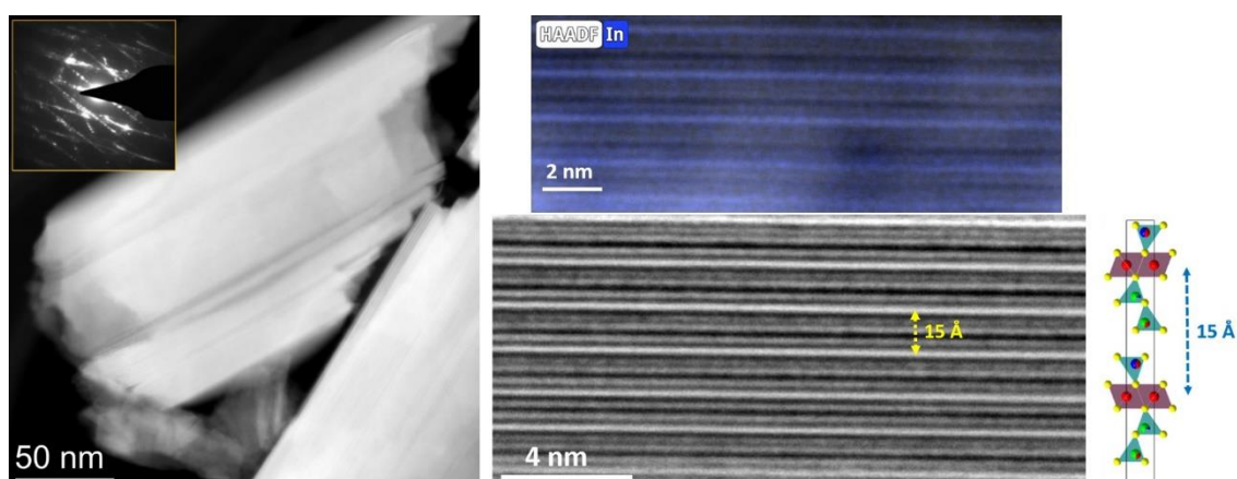
Figure 15: HAADF-STEM images of the powder from scratched CIGS 5 thin film, highlighting the stacking layers on the compound (on the left). The In-S layers are imaged as the bright lines and the van der Waals gaps as the dark lines.
