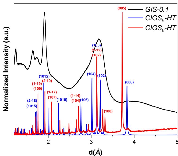
Figure 31: X-ray patterns of GIS-0.1 compared to \text{CIGS}_5 and \text{CIGS}_6 references.
