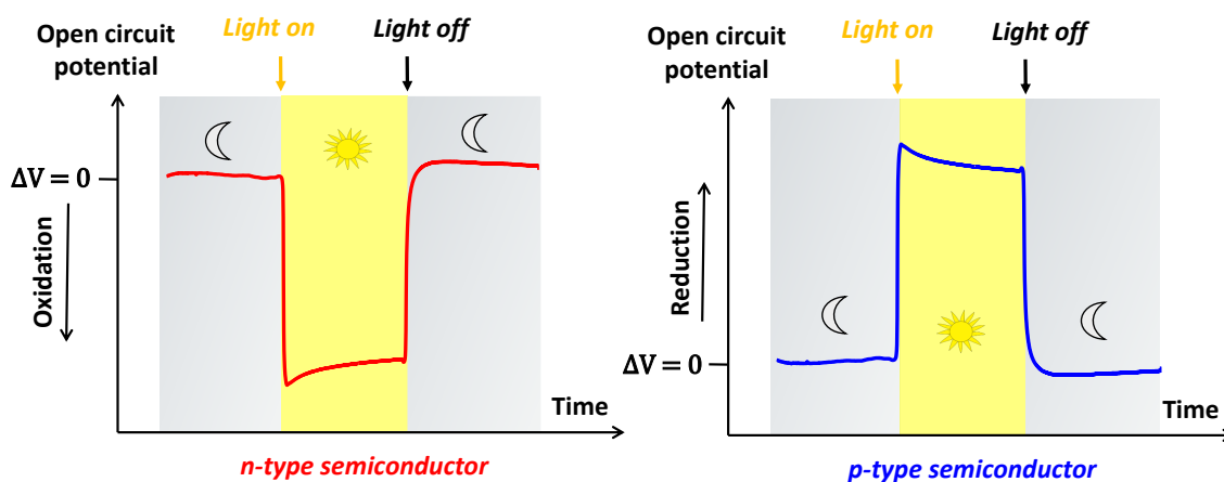
Figure 17: Chronopotentiometry curves under illumination for n-type and p-type semiconductors.
