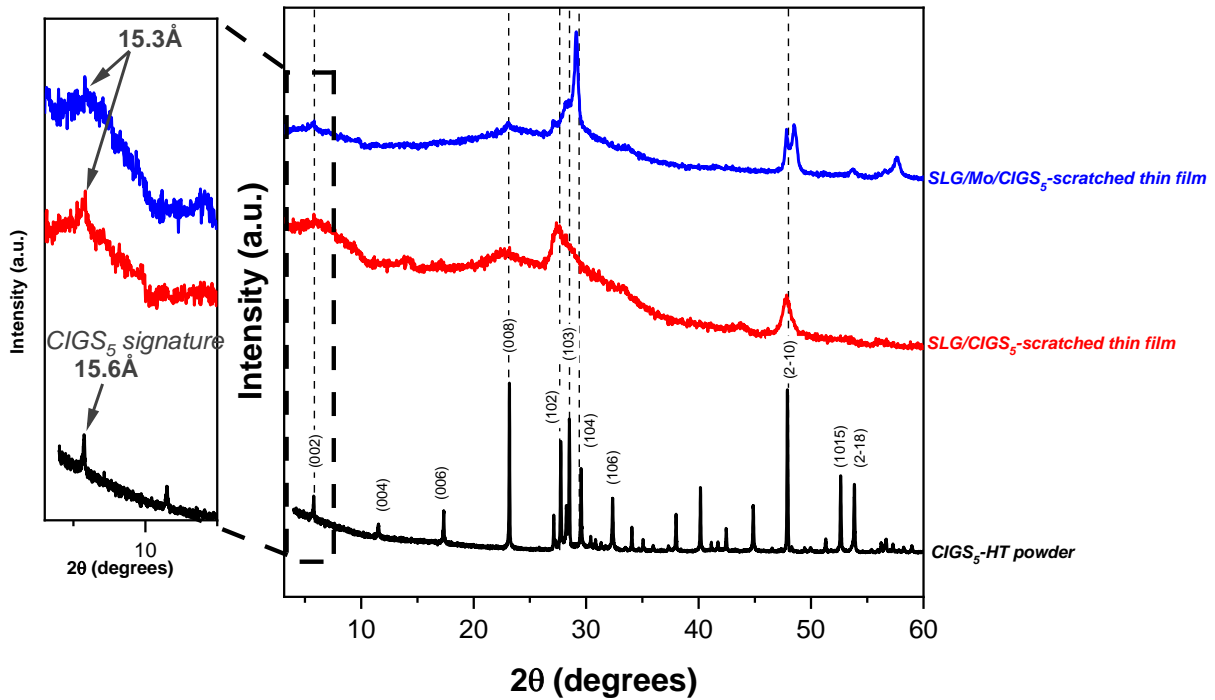
Figure 12: X-ray diffraction patterns of the powders from scratched CIGS 5 thin films on glass and on Mo covered soda lime glass compared to the reference powder of the same target composition Cu_{0.63}In_{1.9}Ga_{1.26}S_5 .
