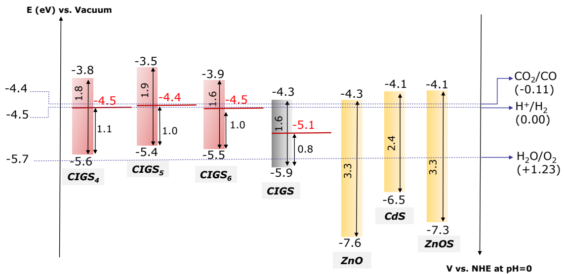
Figure 39: Energy diagrams of CIGS n lamellar compounds and CIGS chalcopyrite with the corresponding redox potentials involved in photocatalyzed applications.
