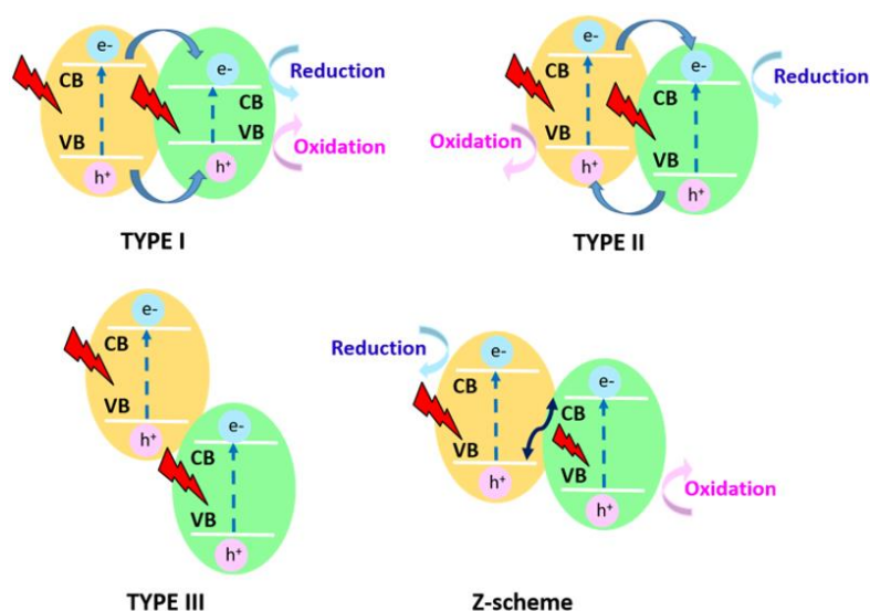
Figure 3: Schematic illustration of the different heterojunction photocatalysts classified based on their energy band alignments (type I, type II, and type III).
