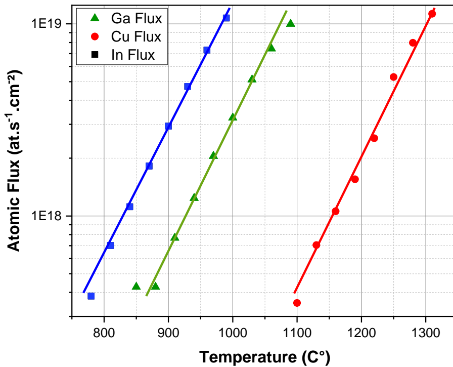
Figure 7: Calibration of the atomic flux of the elemental sources (Cu, In and Ga) as a function of the temperature.
