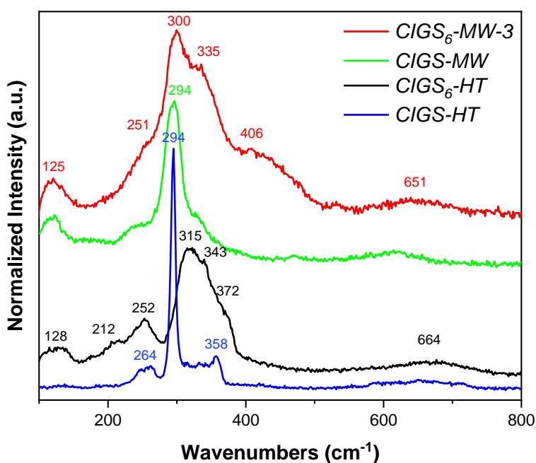
Figure 18: Raman spectra measured at 514 nm of \text{CIGS}_6\text{-MW-3} compared to those of \text{CIGS-MW} , \text{CIGS}_6\text{-HT} and \text{CIGS-HT} .
