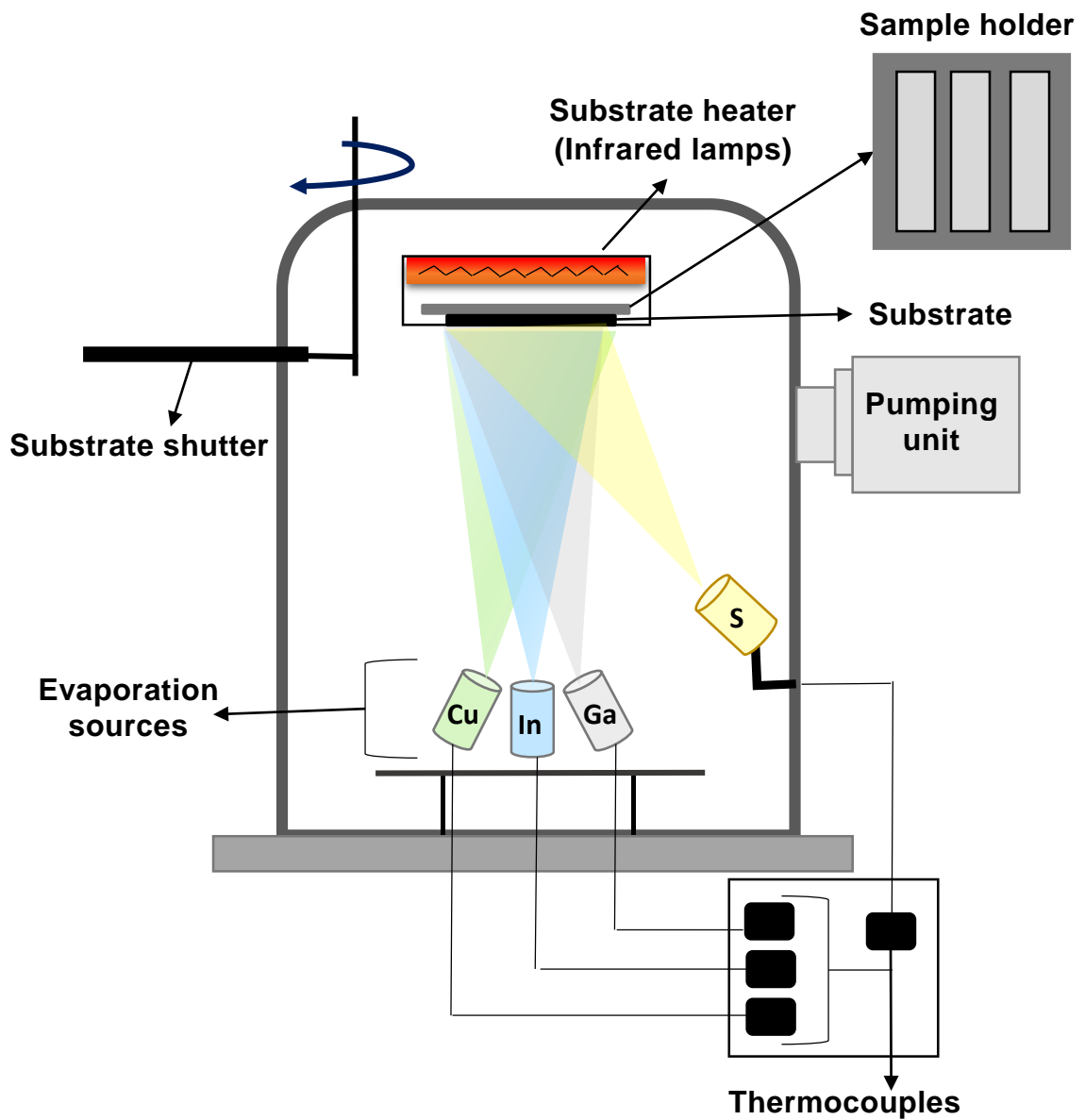
Figure 6: Schematic representation of a co-evaporation deposition chamber.
