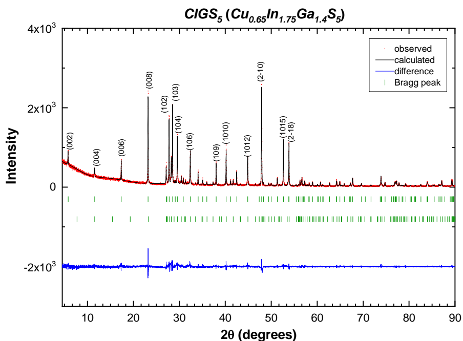
Figure 3: XRD pattern and Le Bail refinement of the \text{CIGS}_5 ( \text{Cu}_{0.65}\text{In}_{1.75}\text{Ga}_{1.4}\text{S}_5 ) compound.
