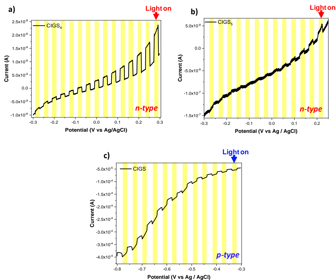
Figure 24: Current-potential curves measured under chopped simulated sunlight with the yellow part corresponding to the illumination time for: a) CIGS 4 , b) CIGS 5 and c) CIGS.
