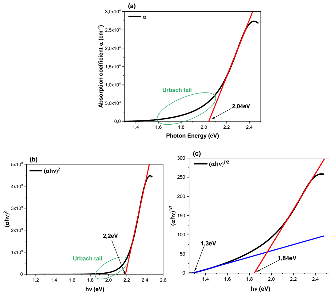
Figure 19: The CIGS_5/SLG a) absorption coefficient plotted spectrum. b) Tauc plot (\alpha hv)^2 versus (hv) that corresponds to direct optical band gap. c) Tauc plot (\alpha hv)^{1/2} versus (hv) that corresponds to indirect optical band gap. With extrapolation of the linear part to 0 indicating the obtained values.
