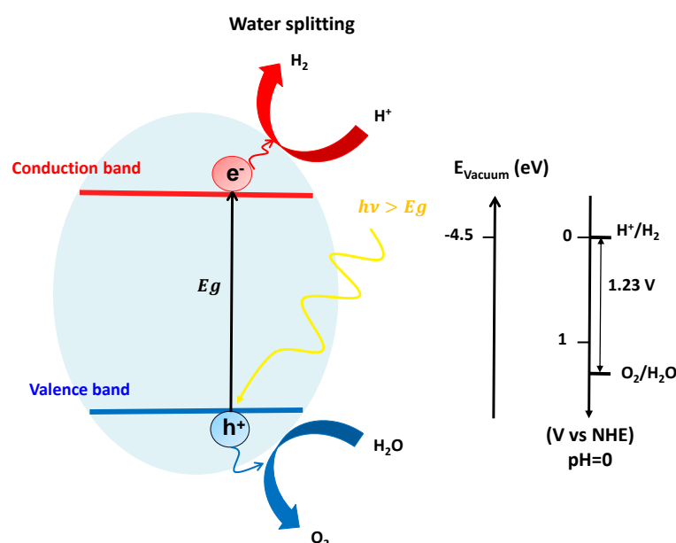
Figure 4: Schematic representation of the overall water splitting, showing the band edge positions of redox potentials of water splitting.
