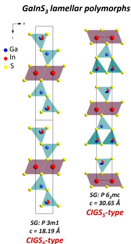
Figure 23: Lamellar polytypes of GaInS_3 : CIGS_6 -type and CIGS_5 -type.
