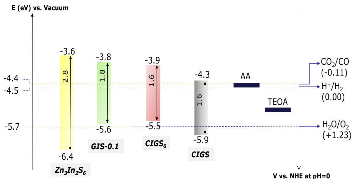
Figure 36: Energy diagram of the CIGS 6 , GIS-0.1, CIGS (either measured or calculated, chapter 2) and Zn 3 In 2 S 6 46,64 positioned to redox potential of the sacrificial electron donors used (AA and TEOA).
