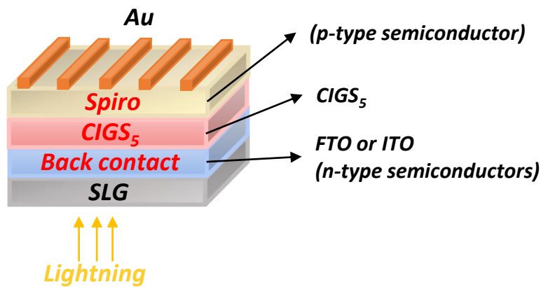
Figure 36: Schematic representation of the n-i-p prepared device, with the different layers used.
