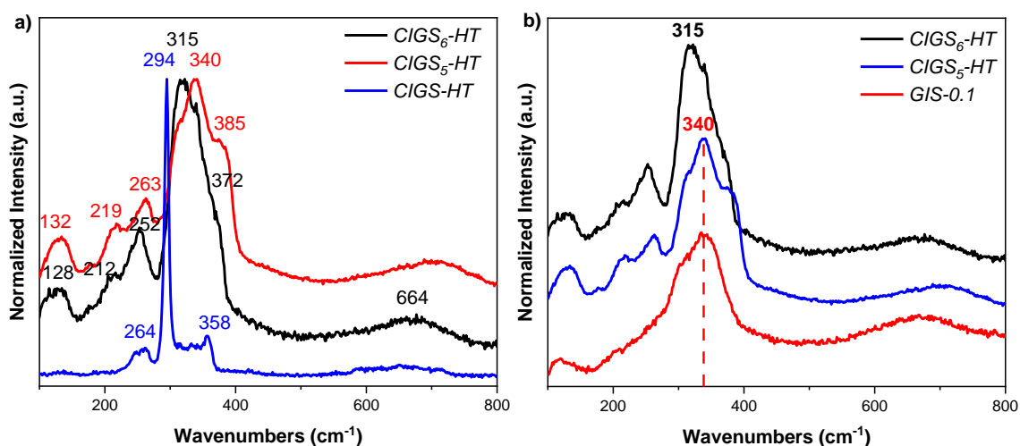
Figure 32: Raman spectra a) of reference compounds \text{CIGS}_5 -HT, \text{CIGS}_6 -HT and \text{CIGS}_5 -HT and b) of GIS-0.1 compared to the \text{CIGS}_5 and \text{CIGS}_6 references.
