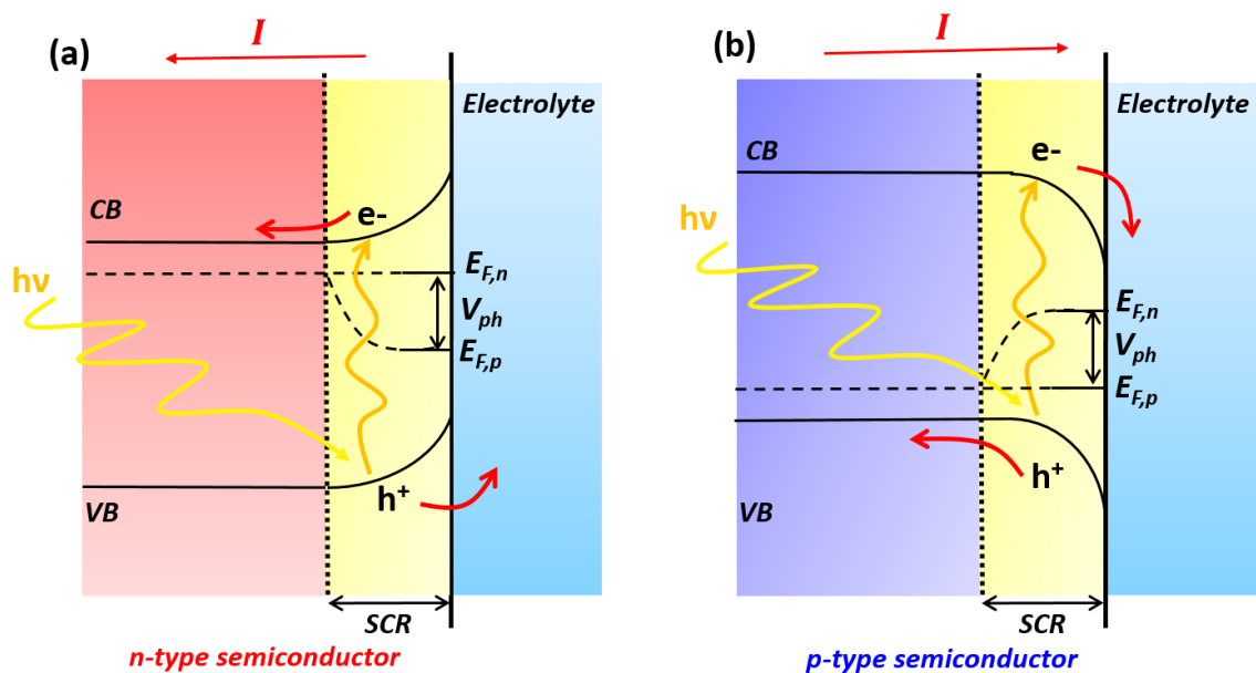
Figure 15: Schematic representation of bands diagrams of n-type and p-type semiconductors under illumination in depletion situation, illustrating the Fermi level split to create a photo voltage.
