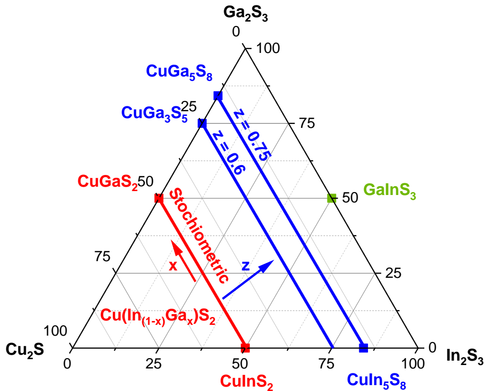
Figure 2: Pseudo-ternary diagram of the \text{Cu}_2\text{S} - \text{In}_2\text{S}_3 - \text{Ga}_2\text{S}_3 system.
