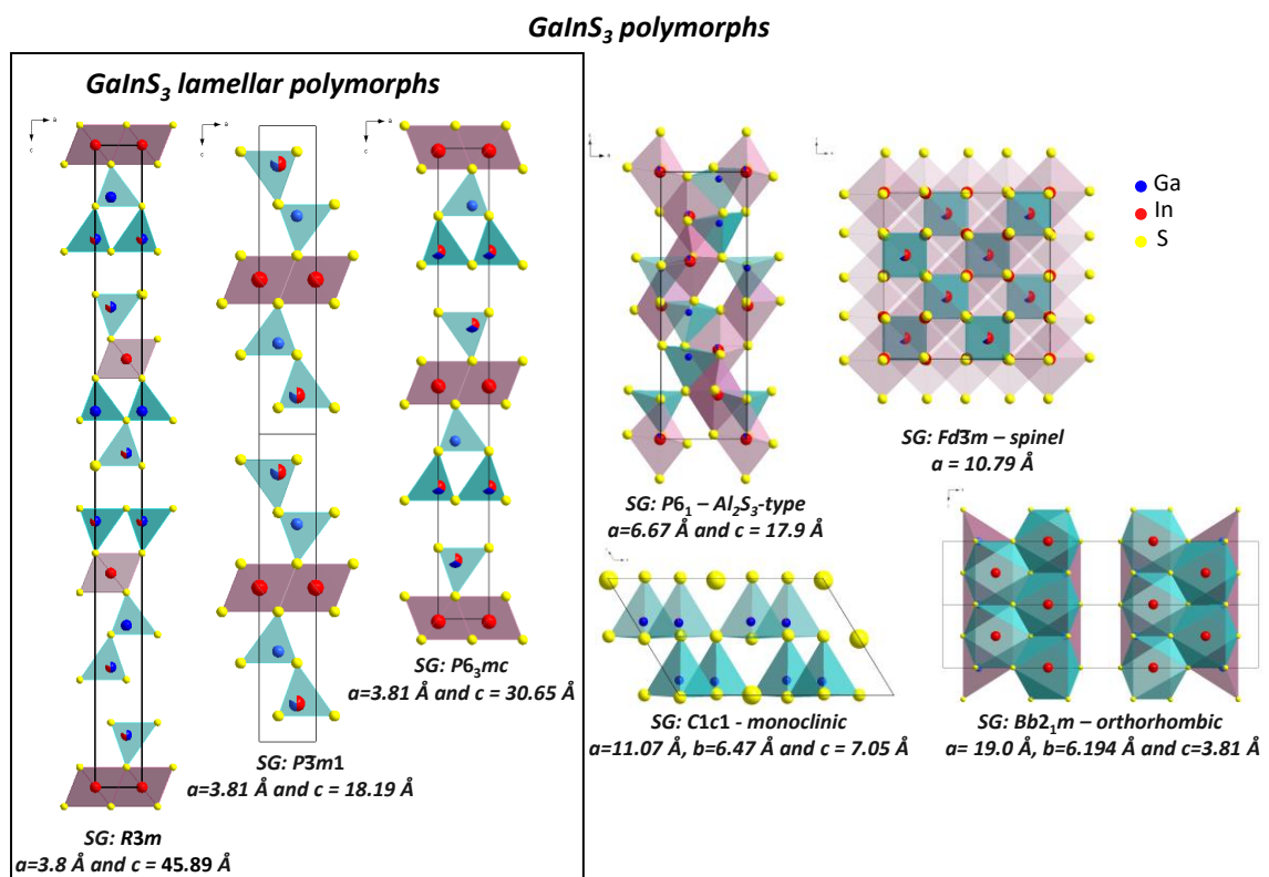
Figure 9: The structures of \text{GaInS}_3 different polymorphs, including the lamellar polymorphs.
