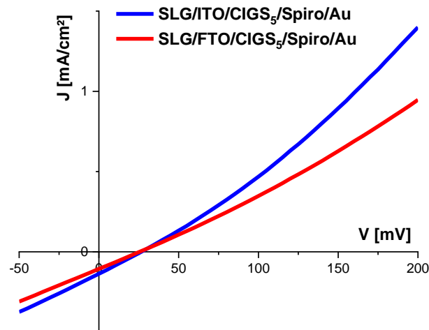
Figure 38: current voltage (JV) curves measured under illumination of the SLG/ITO/CIGS 5 /Spiro-OMeTAD/Au and SLG/FTO/CIGS 5 /Spiro-OMeTAD/Au.
