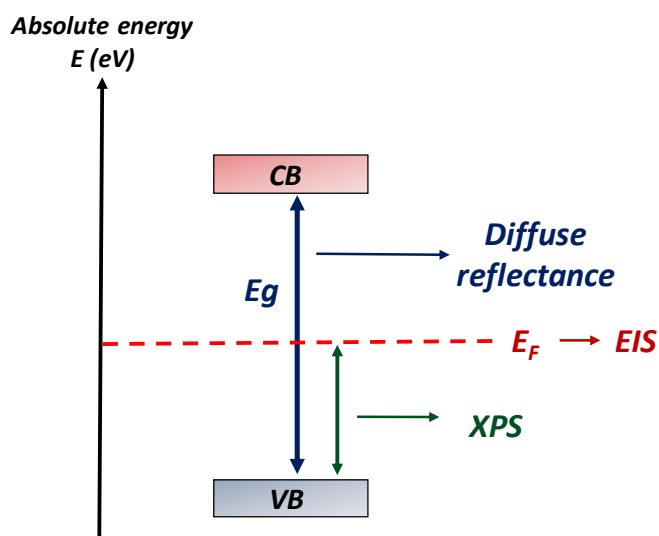
Figure 32: Schematic representation of the energy diagram construction by combining three techniques: diffuse reflectance, electrochemical impedance and x-ray spectroscopy photoelectron spectroscopies.
