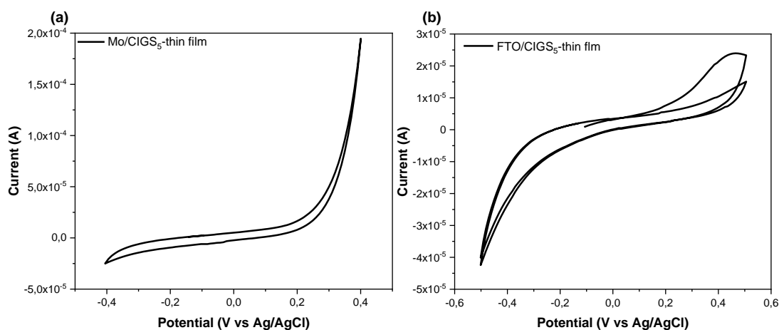
Figure 23: Cyclic voltammetry curve at a scan rate of 5 mV/s of CIGS 5 thin films deposited on a) SLG/Mo and b) on SLG/FTO.
