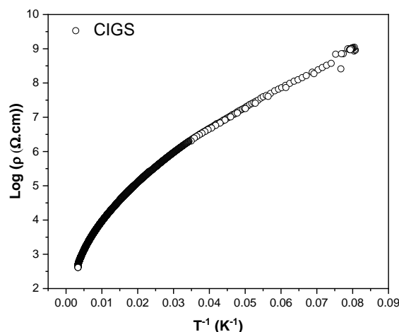
Figure 31: Variation of the exponential of the resistivity of the CIGS sample in function of the temperature.
