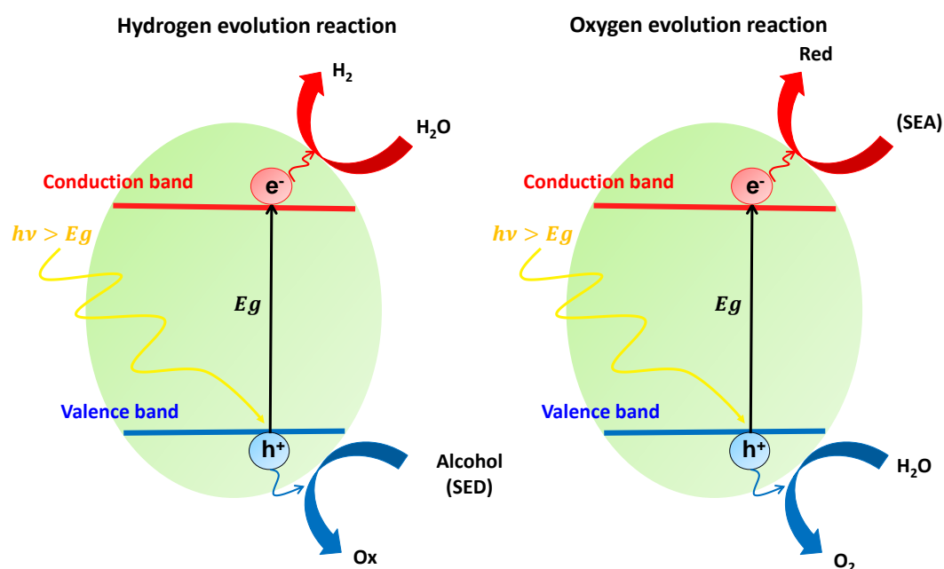
Figure 5: Schematic representation of the principle of hydrogen and oxygen production reactions using an alcohol as sacrificial reagent.
