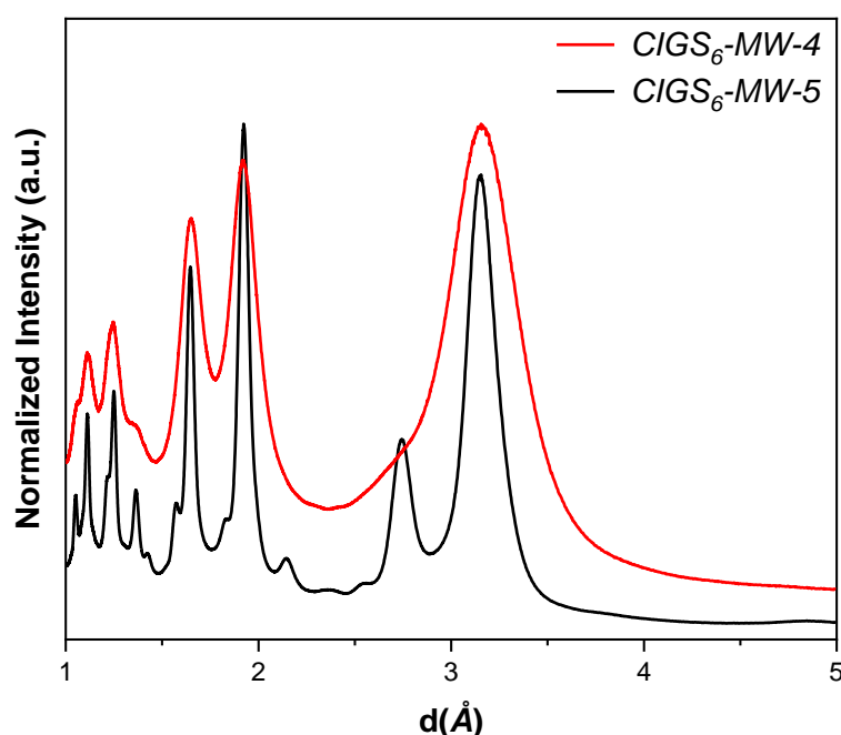
Figure 19: X-ray diffraction patterns of \text{CIGS}_6\text{-MW-4} (15') and \text{CIGS}_6\text{-MW-5} (30').
