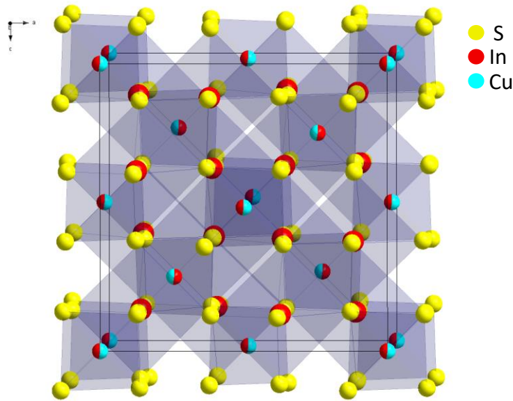
Figure 7: CuIn 5 S 8 thiospinel structure-type.
