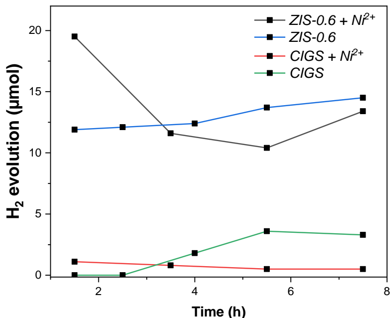
Figure 39: Photocatalytic H 2 evolution as a function of time of ZIS-0.6 and CIGS using acid ascorbic (pH=4) as sacrificial electron donor and NiCl 2 as co-catalyst.
