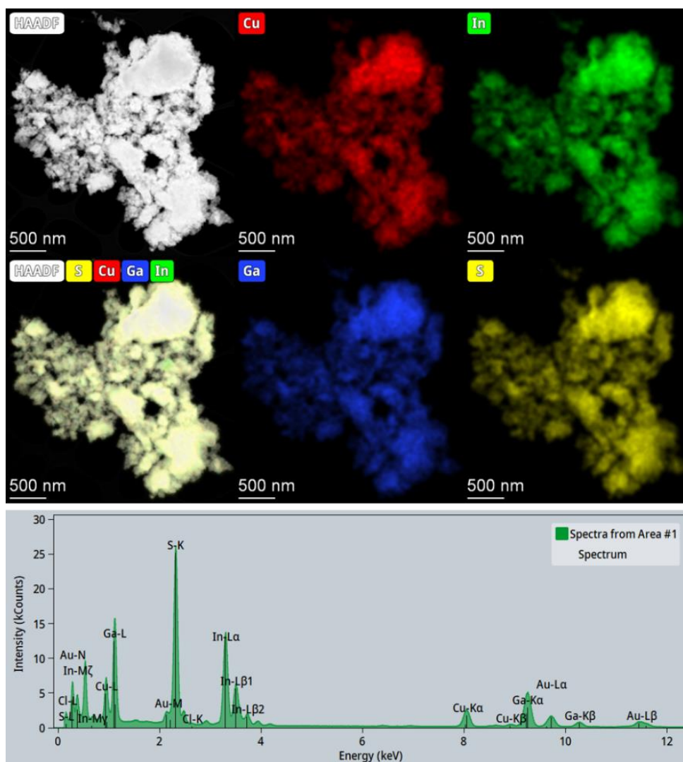
Figure 30: EDX mapping and EDX spectrum of GIS-0.1 copper poor compound.
