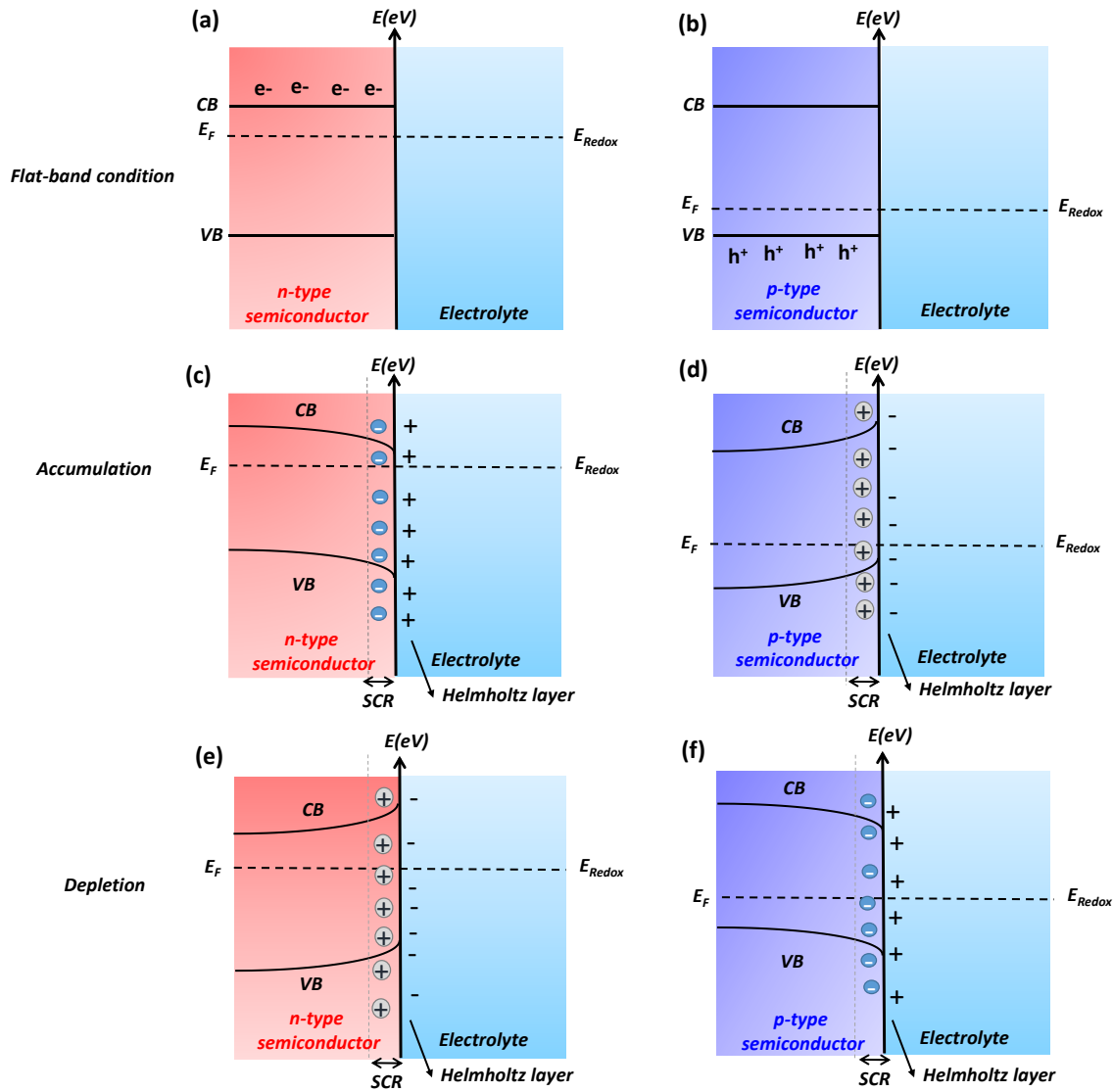
Figure 12: Schematic representation of bands bending for n-type and p-type semiconductors before and during contact with the electrolyte, presenting different situations.
