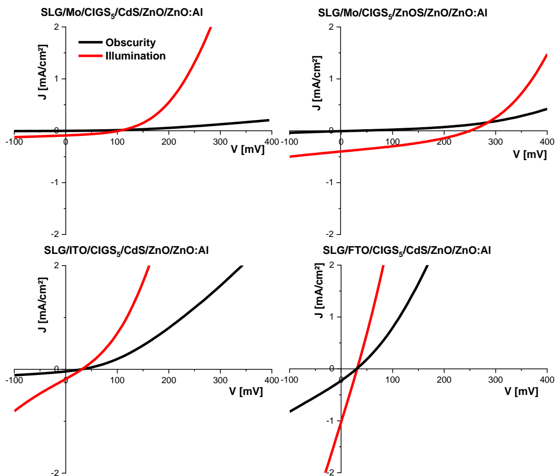
Figure 31: current voltage (JV) curves measured in dark and under illumination of the solar cells prepared from the different investigated films
