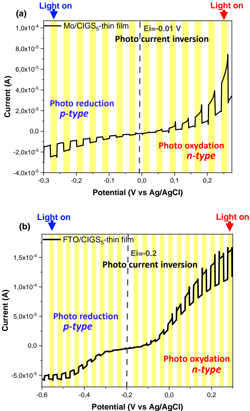
Figure 28: Current-potential curve measured under chopped simulated sunlight with the yellow part corresponds to the illumination time for CIGS 5 thin films: a) SLG/Mo/CIGS 5 . b) SLG/FTO/CIGS 5 .
