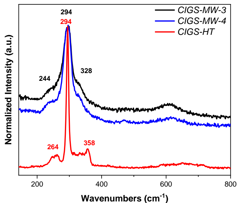
Figure 14: Raman spectra measured at 514 nm of CIGS-MW-3 and CIGS-MW-4 compounds compared to that of CIGS-HT.
