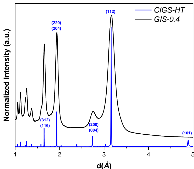
Figure 28: X-ray pattern of copper rich sample GIS-0.4 compared to that of CIGS chalcopyrite.
