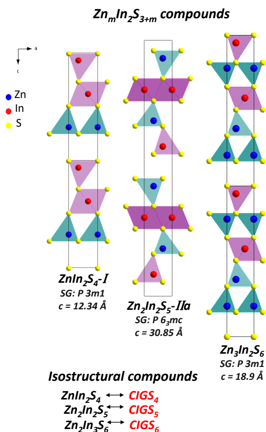
Figure 7: Structures of Zn_mIn_2S_{3+m} compounds ( m = 1, 2 and 3 ) isostructural of CIGS_n compounds.
