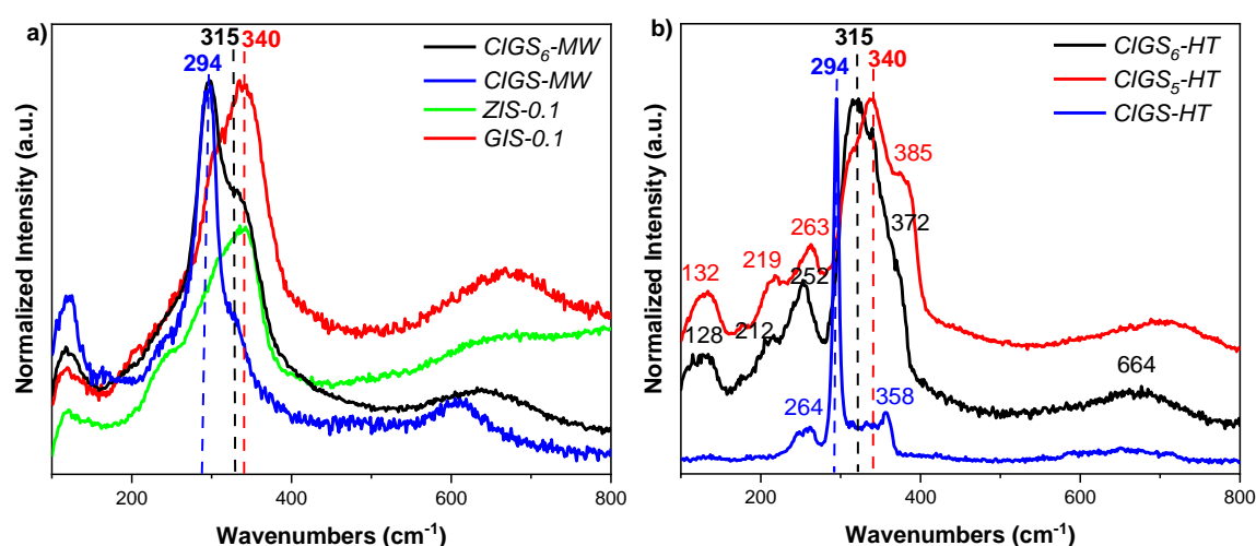
Figure 34: Raman spectra a) of CIGS and all the lamellar compounds prepared by microwave-assisted solvothermal synthesis and b) of reference compounds CIGS-HT, CIGS 5 -HT and CIGS 6 -HT.
