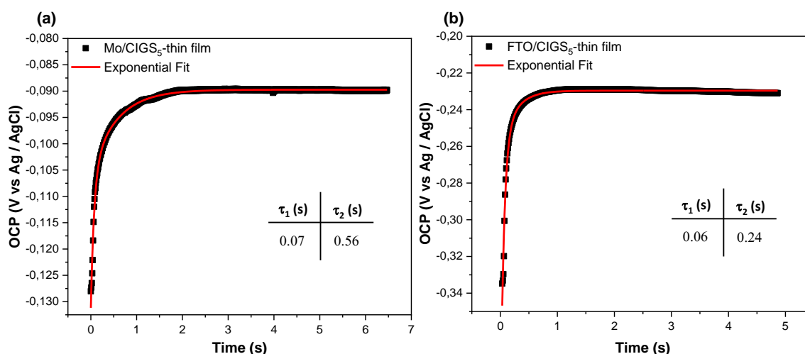
Figure 27: Open circuit curves under dark fitted using the exponentials in order to determine the charge carrier lifetime for of thin films: a) SLG/Mo/CIGS 5 . b) SLG/FTO/CIGS 5 .
