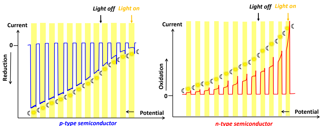
Figure 16: Current potential curves under chopped illumination, for p-type (photo-reduction) and n-type (photo-oxidation) semiconductors.
