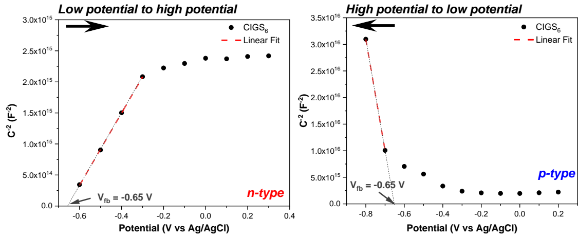
Figure 29: Mott-Schottky plots of CIGS 6 with the flat band potentials, when performing the experiment from low potential to high potential and high potential to low potential.
