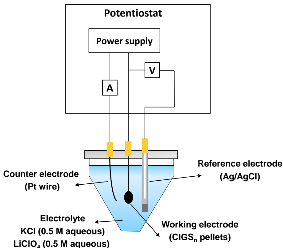
Figure 9: Schematic representation of electrochemical cell with three electrodes, with specific electrodes and electrolyte used during this PhD.
