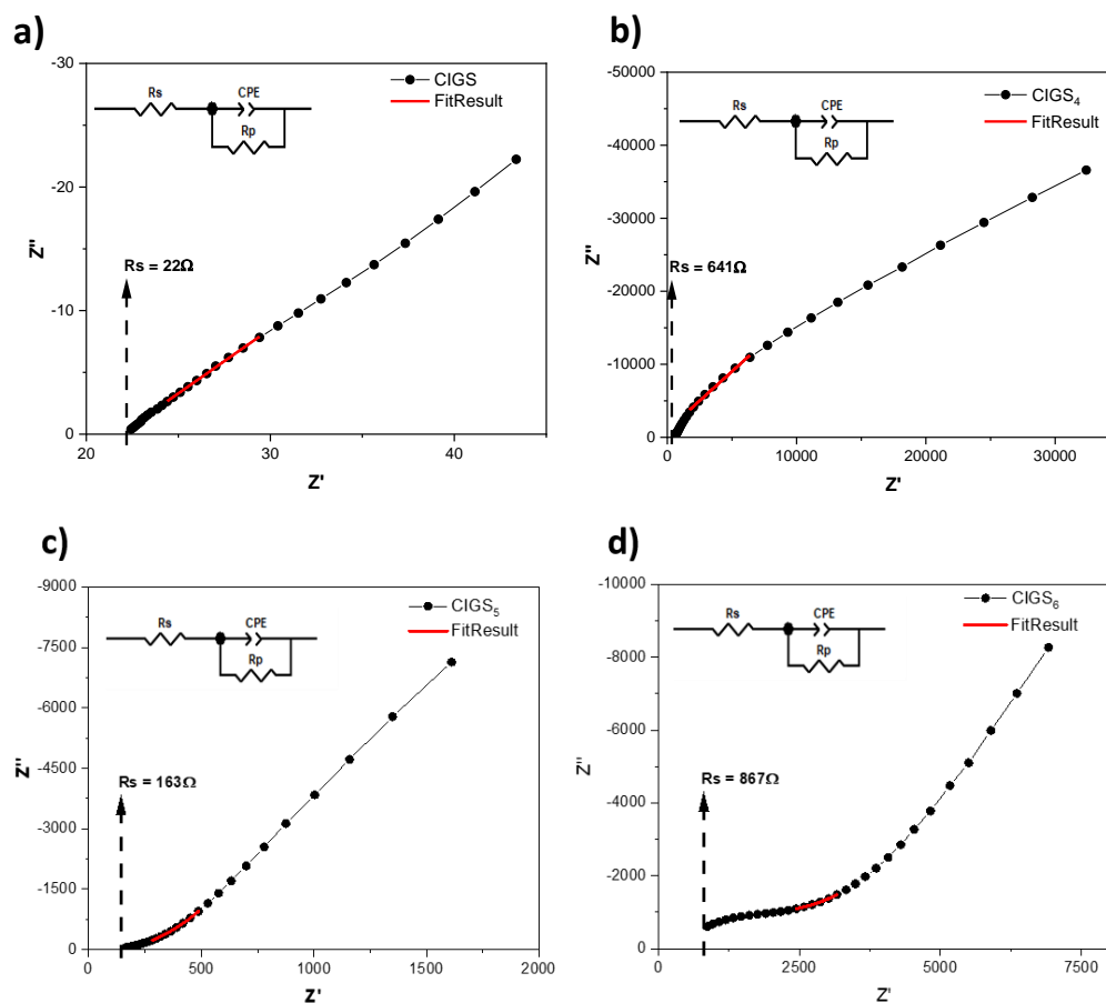
Figure 27: Nyquist plots of the electrochemical impedance circuit in the dark with the applied equivalent circuit for fitting at high frequencies (1– 10 kHz) of: a) CIGS, b) CIGS 4 , c) CIGS 5 and d) CIGS 6 .
