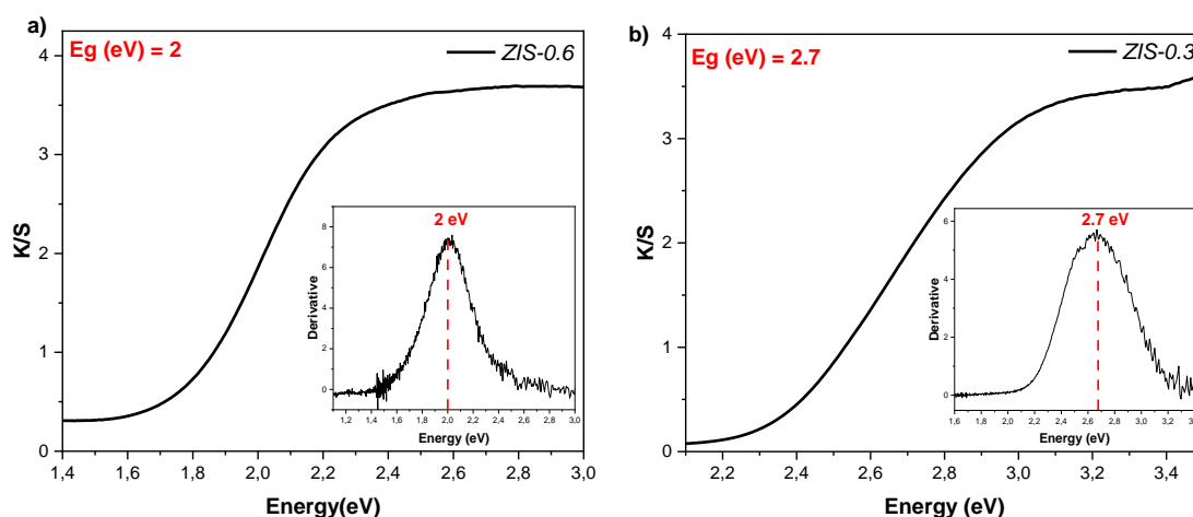
Figure 25: Kubelka-Munk transformed reflectance spectra of the a) ZIS-0.6 and b) ZIS-0.3 samples.
