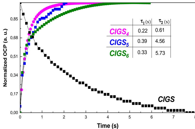
Figure 38: Normalized chronopotentiometry after stopping the illumination of all compounds.
