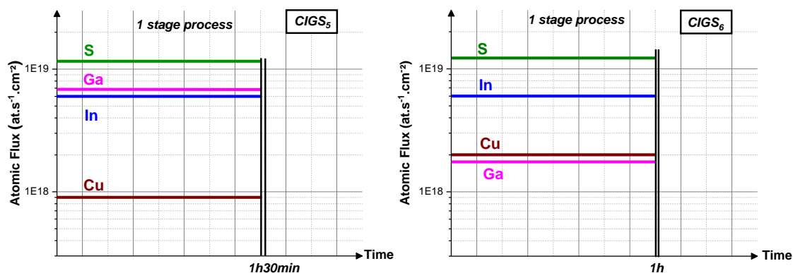
Figure 8: The 1-stage process followed for CIGS 5 and CIGS 6 deposition.
