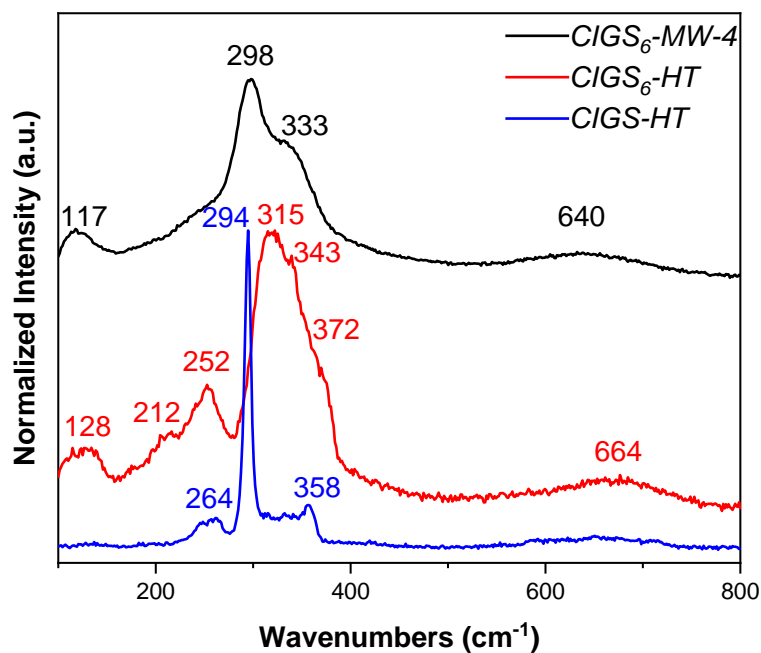
Figure 22: Raman spectra measured at 514 nm of CIGS 6 -MW-4 compared to the CIGS and CIGS 6 high temperature powders.
