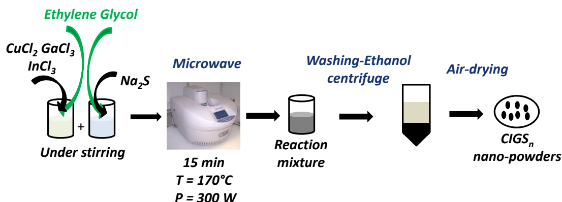
Figure 9: Synthesis protocol followed to prepare the \text{CIGS}_n nanopowders using microwave-assisted solvothermal synthesis.
