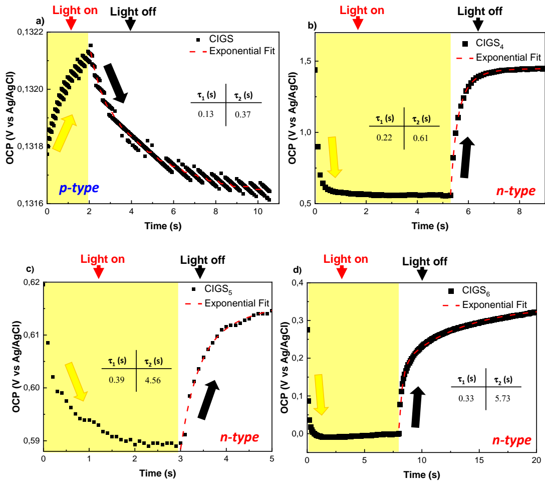
Figure 23: Open circuit potential (OCP) curves under illumination (yellow region) and under dark of a) CIGS, b) CIGS 4 , c) CIGS 5 and d) CIGS 6 . The photogenerated charge carrier lifetimes in the inserted tables were determined by fitting the OCP decay curves after stopping the illumination by two decreasing exponential functions.
