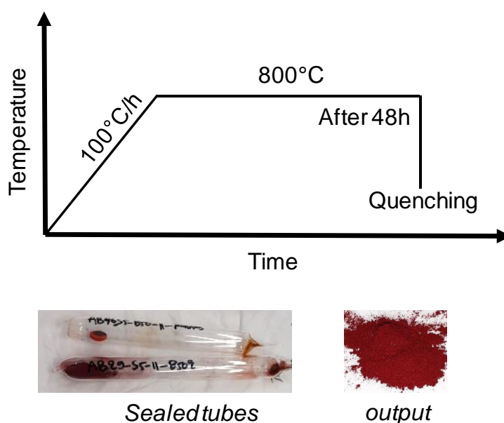
Figure 1: Protocol followed for the synthesis and annealing of high temperature powders by the ceramic route.
