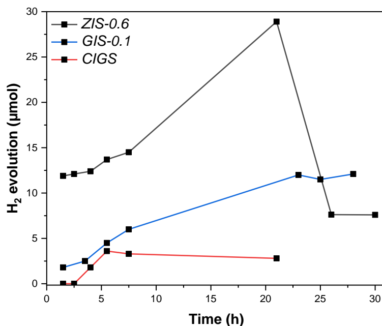
Figure 38: Photocatalytic H 2 evolution as a function of time of ZIS-0.6, GIS-0.1 and CIGS using acid ascorbic (pH=4) as sacrificial electron donor.
