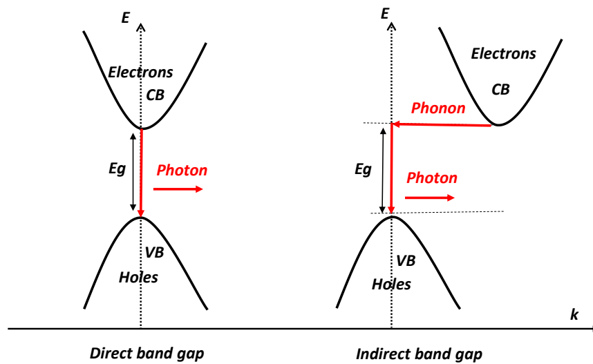
Figure 8: Schematic representation of direct and indirect band gap semiconductors.
