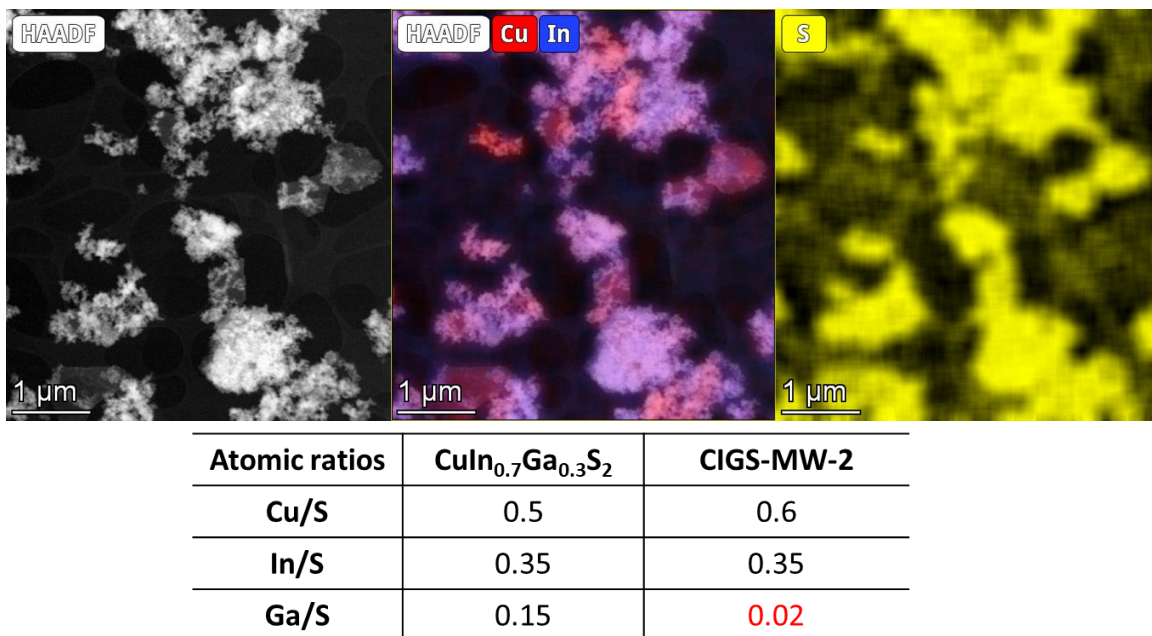
Figure 11: EDX mapping of sample CIGS-MW-2 showing an inhomogeneous chemical composition of the nanograins agglomerates. A significant gallium deficit compared to the target composition \text{CuIn}_{0.7}\text{Ga}_{0.3}\text{S}_2 is noted (see inserted table).
