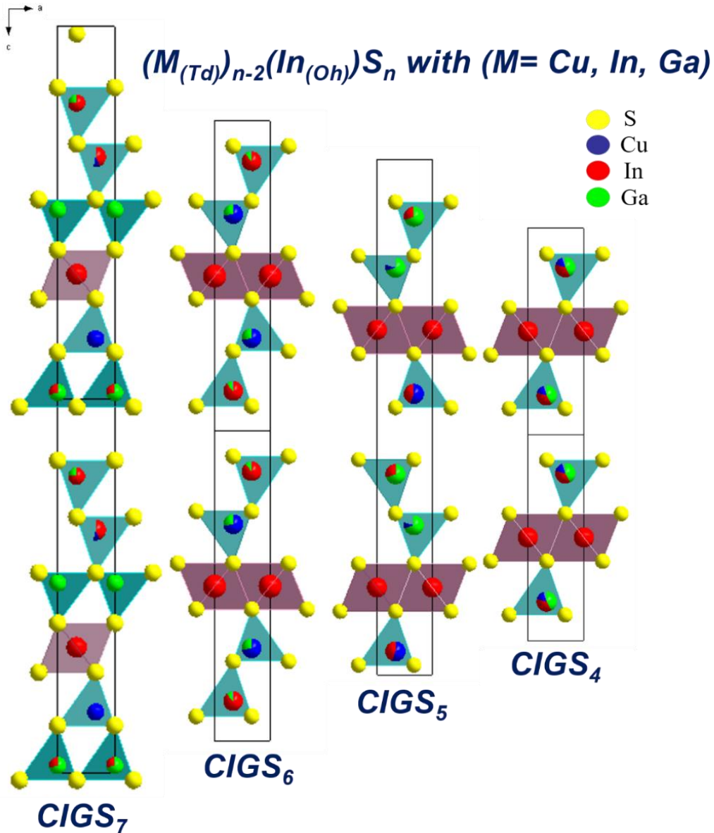
Figure 11: CIGS 7 (Cu 1.1 In 2.49 Ga 1.8 S 7 ), CIGS 6 (Cu 1.44 In 2.77 Ga 0.76 S 6 ), CIGS 5 (Cu 0.65 In 1.75 Ga 1.4 S 5 ) and CIGS 4 (Cu 0.32 In 1.74 Ga 0.84 S 4 ) lamellar compounds structures.
