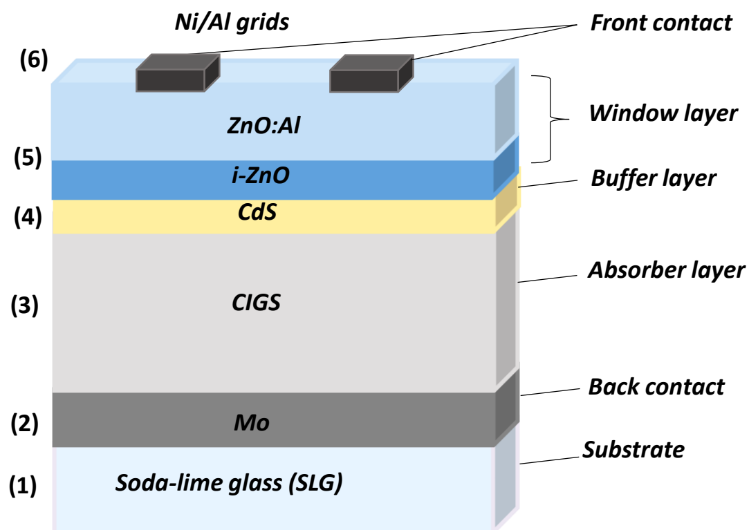
Figure 5: Schematic representation of a standard CIGS cell.
