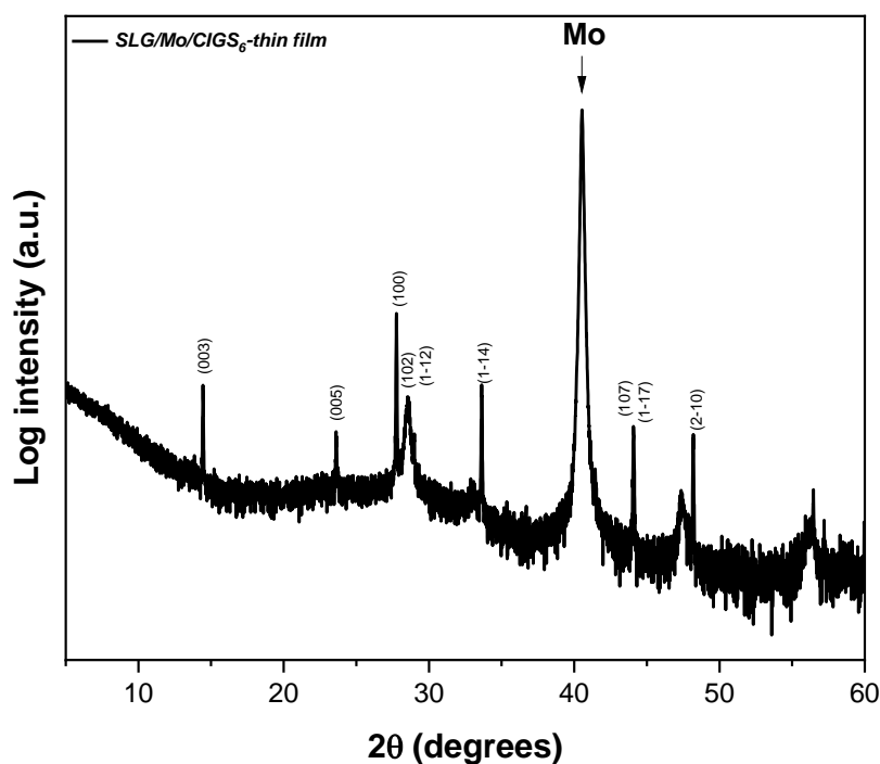
Figure 11: X-ray diffraction pattern of CIGS 6 deposited on Mo-covered soda lime glass on a logarithmic scale.
