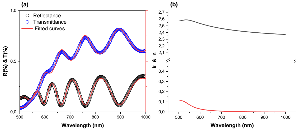
Figure 18: a) The experimental optical transmission T and the reflection R spectra of CIGS_5/SLG and their fitted curves. b) The refractive index n and the extinction coefficient k computed after a certain number of iterations.
