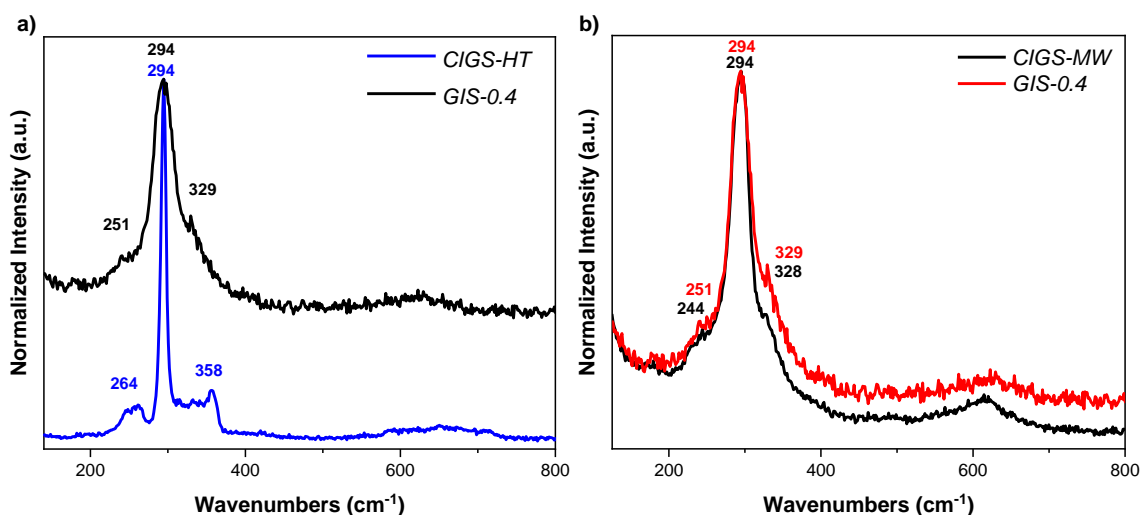
Figure 29: Raman spectra of GIS-0.4 copper rich sample compared to a) CIGS chalcopyrite high temperature reference and b) CIGS-MW chalcopyrite prepared by microwaves.
