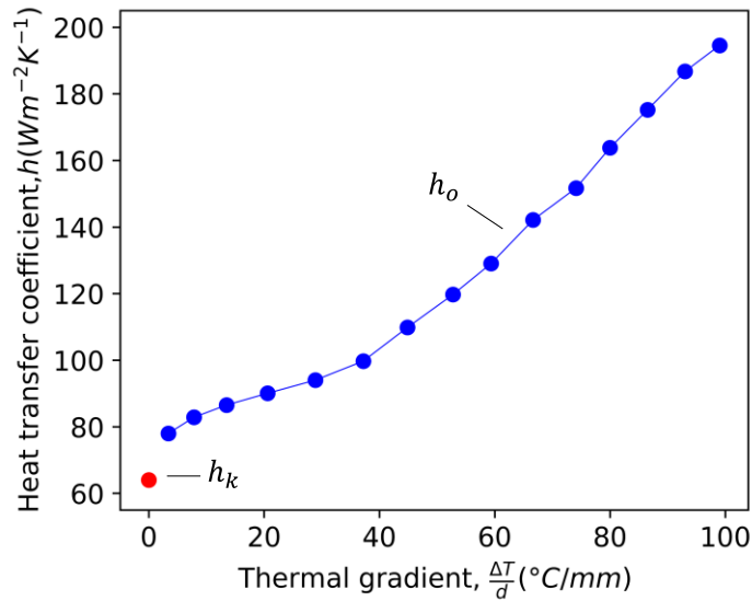
Fig 4.6. Convective heat transfer in coaxial test cell filled with DBT, and comparison with value h_k involving conduction only
