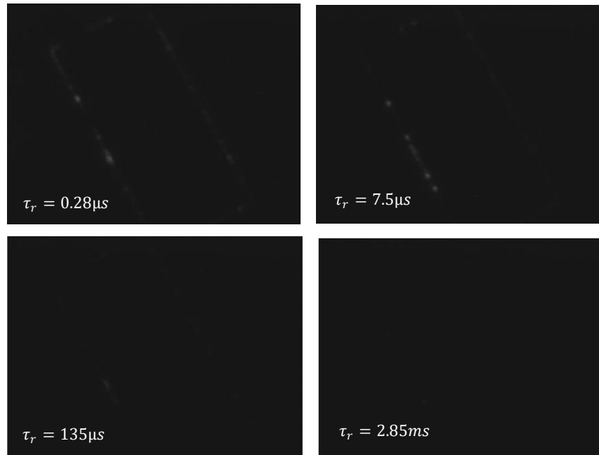
Fig 3.43. CCD camera observation of light under V_{BI} at 6kV(cc) with Si_3N_4 substrate (single layer) embedded in silicone oil at different rise time ( t_r )
