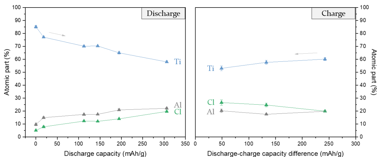
Figure S61. EDX elemental rates measurement of Ti, Al, and Cl along the first discharge (left) and charge (right) of the galvanostatic cycling experiment. The grey arrows indicate the reading order.
