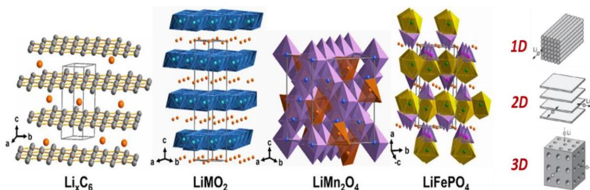
Figure 4. Various lithium-ion intercalation positive electrode materials. Consistently, the lithium-ion is displayed in orange. The diffusion of \text{Li}^+ can be whether 3D (such as in the spinel \text{LiMn}_2\text{O}_4 ), 2D (such as in the lamellar \text{LiMO}_2 or graphite), or 1D (such as in the olivine \text{LiFePO}_4 ). Adapted from 17 .
