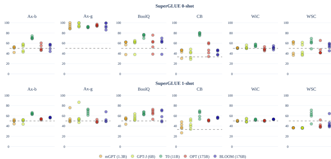
Figure 6.7: Performance of various LLMs on subset of tasks from SuperGLUE benchmark in zero- and one-shot prompt-based setting.
