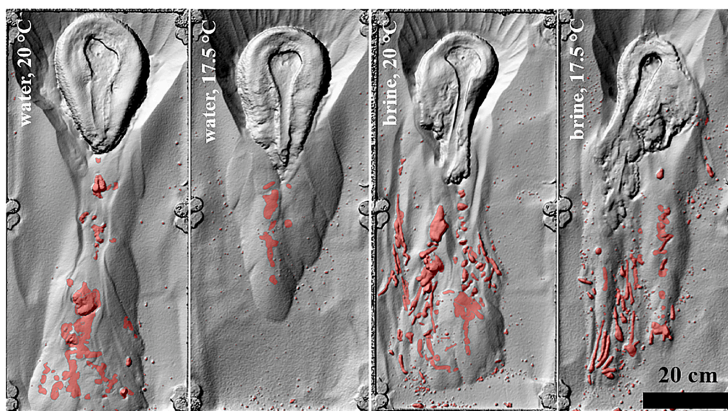
Fig. 15. comparison between water and brine flows, at 20 °C and 17.5 °C. Pellets are identified with the light red colour. A lot more pellets are formed with the brine flows and the resulting morphologies seem more chaotic. The hillshades displayed here are from experiments 03 (water, 20 °C), 05 (brine, 20 °C), 25 (water, 17.5 °C) and 30 (brine, 17.5 °C).
