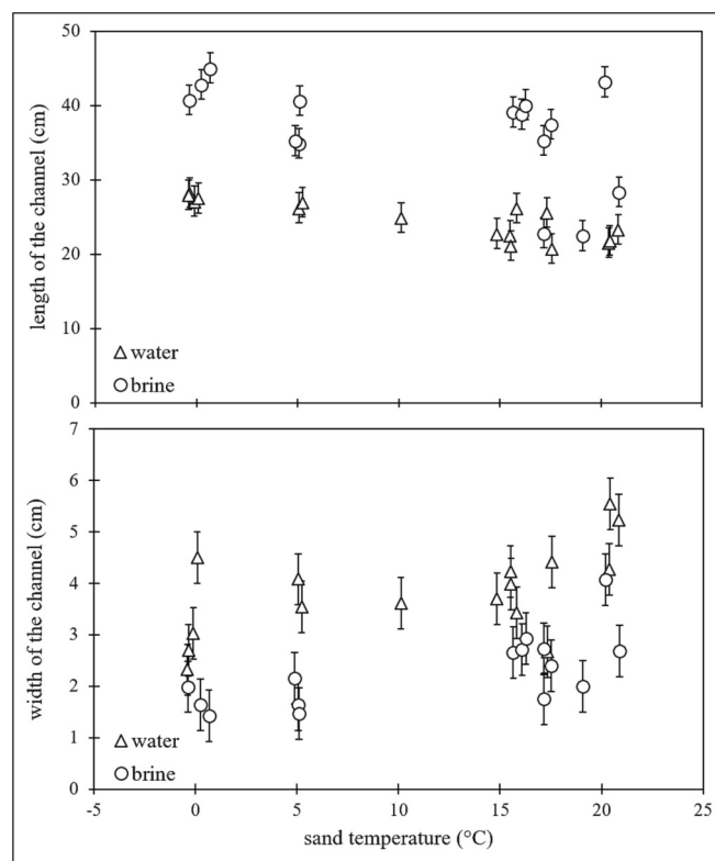
Fig. 13. length (top) and width (bottom) of the channel vs. sand temperature, for water (triangles) and brine experiments (circles). The errors in the sand temperature fall within the symbols. The errors in the length and width of the channels have been estimated at respectively 2 cm and 0.5 cm.
