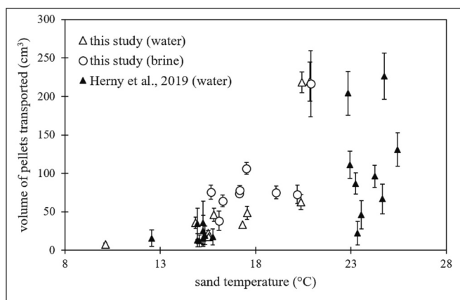
Fig. 14. volume of pellets moved vs. sand temperature. The experiments displayed here are the “hot” ones (sand temperature from 10 °C to 20 °C). The data from Herny et al. (2019) are added as small black triangles, and are water flows experiments only. The volume of covered pellets (our unit 6) was not measured by Herny et al. (2019) . The error bars on the sand temperature are negligible.
