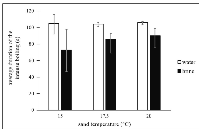
Fig. 10. average duration of the intense boiling for water and brine at 15, 17.5 and 20 °C. The error bars are defined as the shortest and the longest boiling durations observed at the different sand temperatures.
