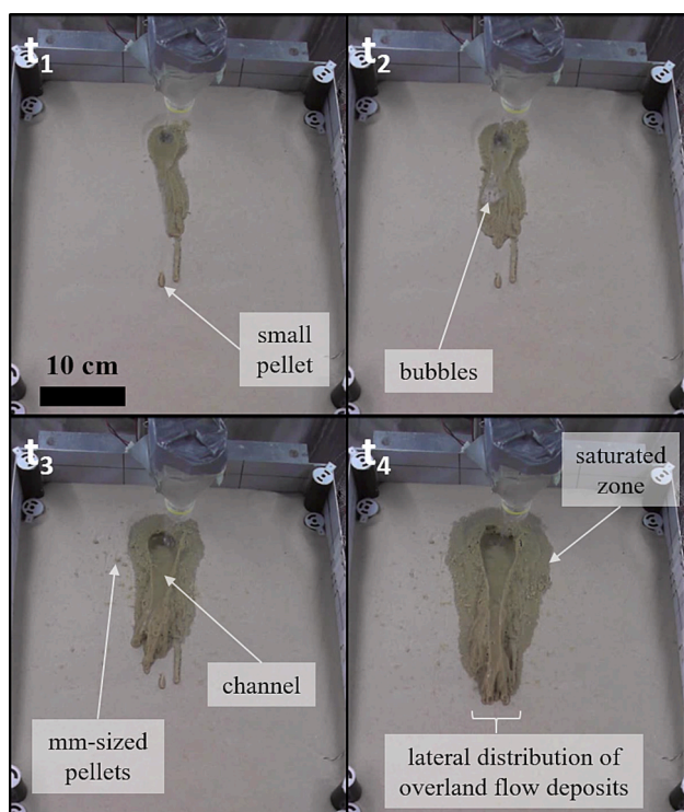
Fig. 8. images from experiment 16 (water, 5 °C) at t_1 = 5 s, t_2 = 10 s, t_3 = 30 s, t_4 = 60 s after the beginning of the experiment. We observe the growth of the channel and its deposits, enlargement of the saturated zone and ejection of mm-sized pellets.
