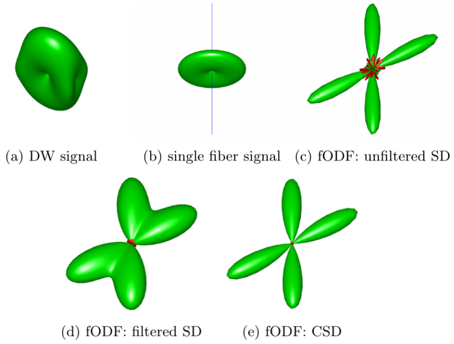
Figure 2.12 – Spherical deconvolution of a noiseless DW signal (a) with a single fiber response function (b) using unfiltered (c), filtered (d) and constrained (e). Green indicates positive amplitude, while red indicates negative amplitude. From [Jeurissen, 2012]
