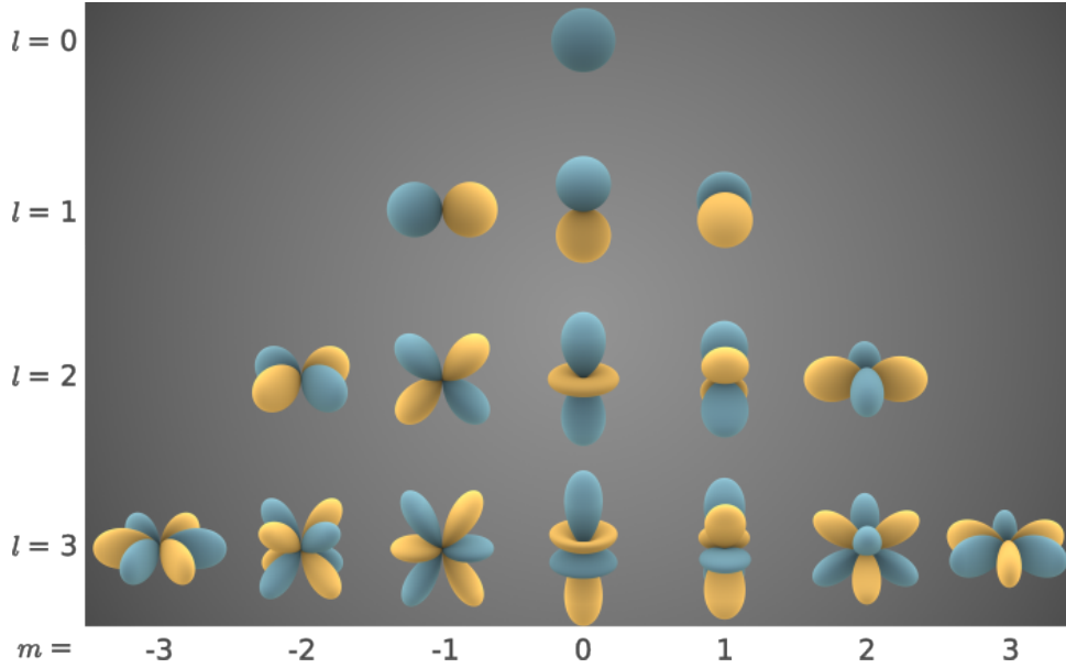
Figure 2.8 – Real part of the spherical harmonic basis up the order l = 3 . The function value is visualized as the distance from the origin to the surface. Blue indicates positive function values. Yellow indicates negative function values. From https://en.wikipedia.org/wiki/Spherical_harmonics .
