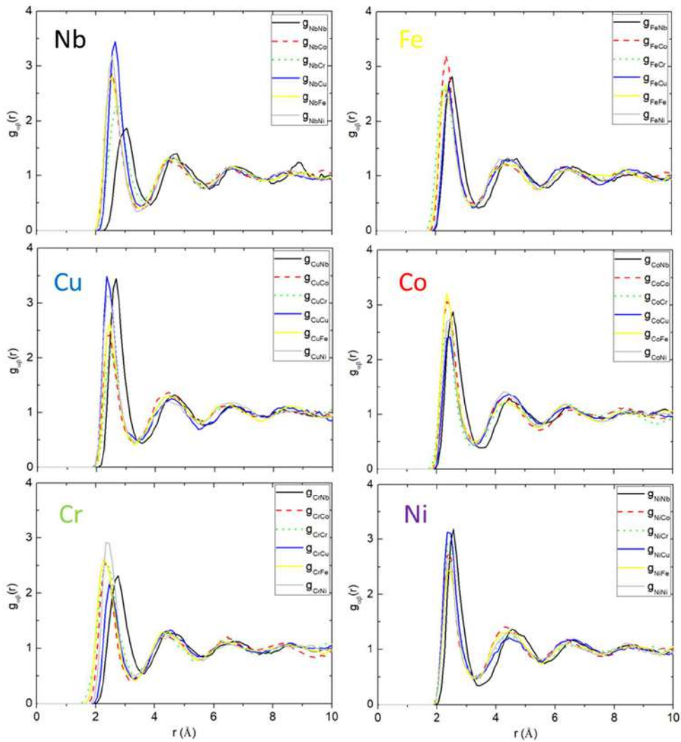
Figure 5.5 - AIMD (256 atoms) simulated partial pairs correlation functions of the melt CoCrCuFeNiNb_{0.95} (16 at.% Nb ) from NVT canonical at 2000 K after the simulation time of 9 ps, showing Cu clustering and short-range ordering between Nb -( Cu , Ni , Cr , Fe ), Fe -( Co , Cr ) and Cr -( Ni , Co , Fe ) pairs.
